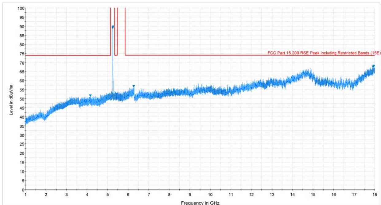
Plot 7-82. Radiated Spurious Plot above 1GHz (802.11a – U2A Ch. 56, Ant. Pol. V)
