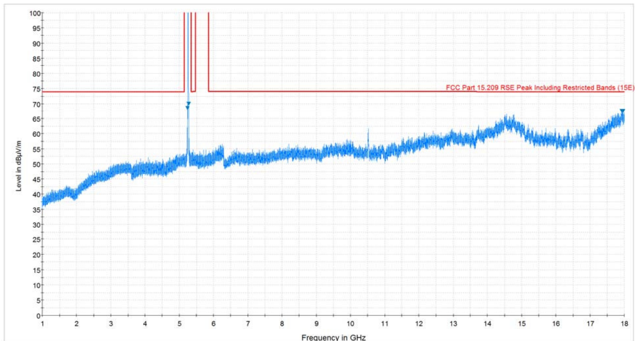
Plot 7-81. Radiated Spurious Plot above 1GHz (802.11a – U2A Ch. 56, Ant. Pol. H)
