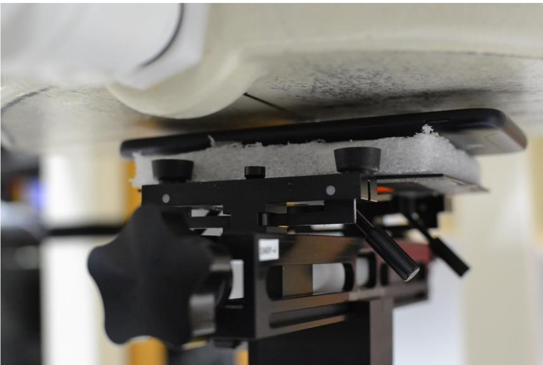
SAR Test Setup Photo 10- Front Side at 0.7 cm (Phablet)
