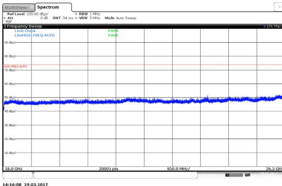
Plot 7-49. Radiated Spurious Plot above 18GHz (Pol. V)
