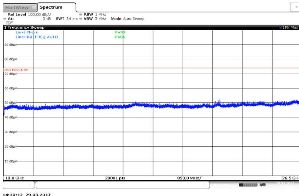
Plot 7-48. Radiated Spurious Plot above 18GHz (Pol. H)
