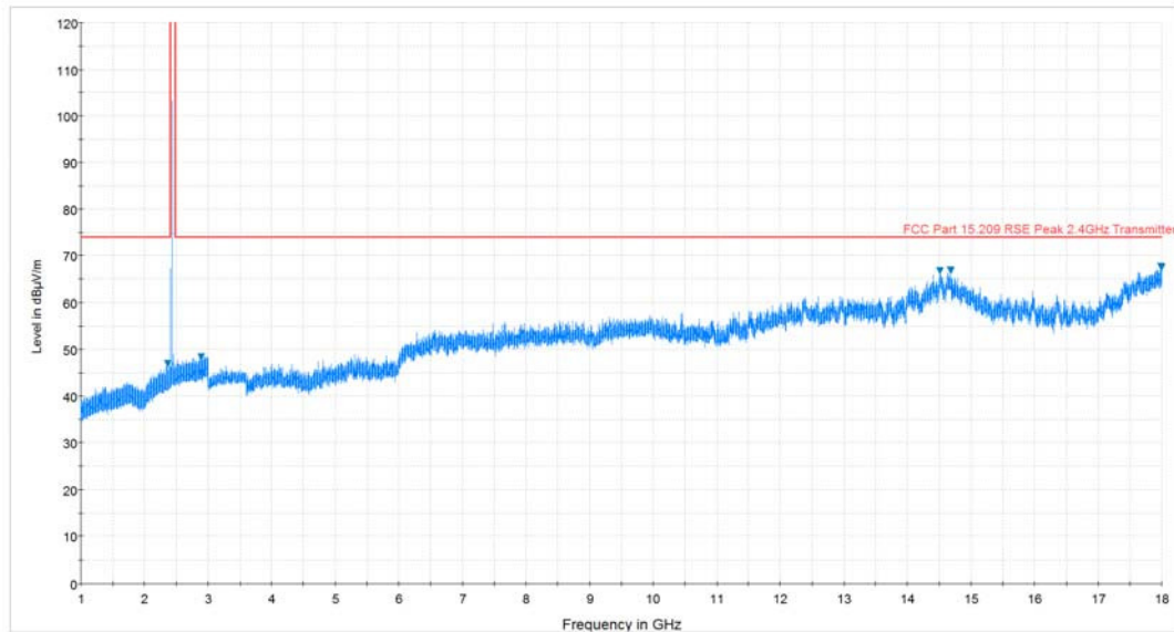
Plot 7-44. Radiated Spurious Plot above 1GHz (BT – Ch. 39, Ant. Pol. H)
