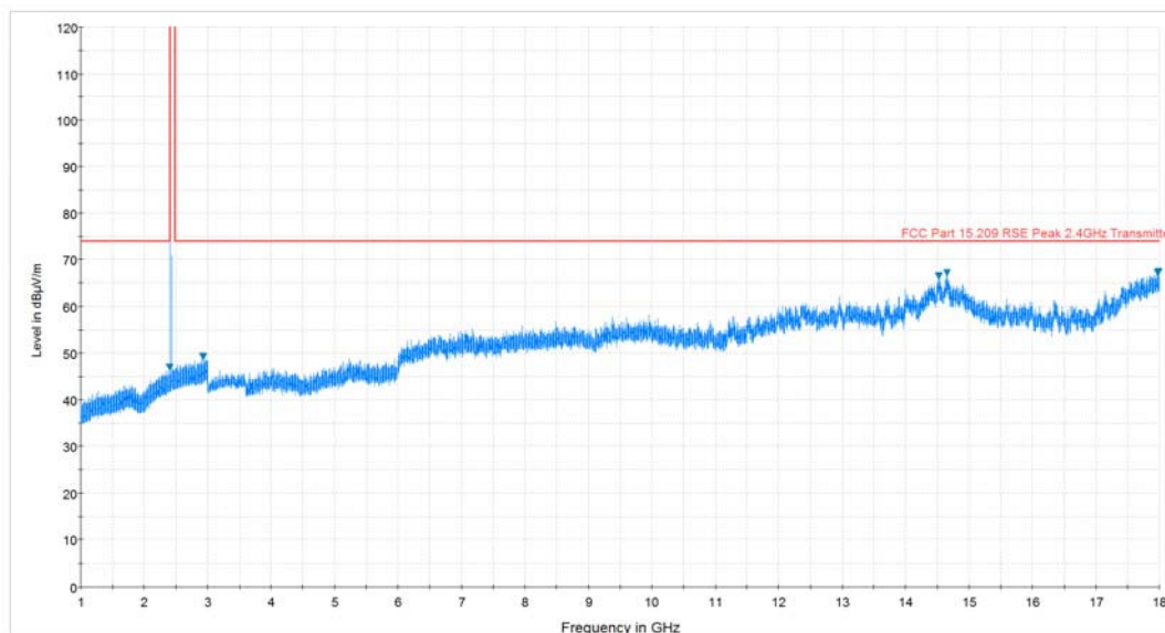
Plot 7-43. Radiated Spurious Plot above 1GHz (BT – Ch. 0, Ant. Pol. V)
