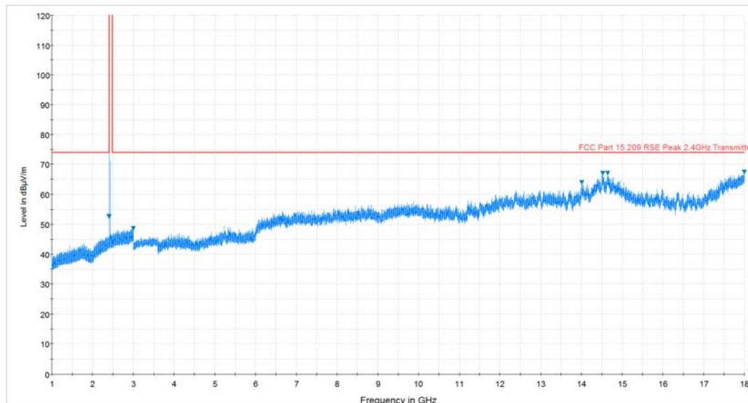
Plot 7-42. Radiated Spurious Plot above 1GHz (BT – Ch. 0, Ant. Pol. H)
