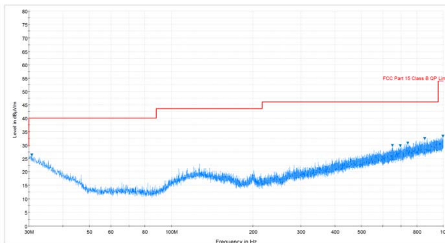
Plot 7-52. Radiated Spurious Plot below 1GHz (Pol. H)
