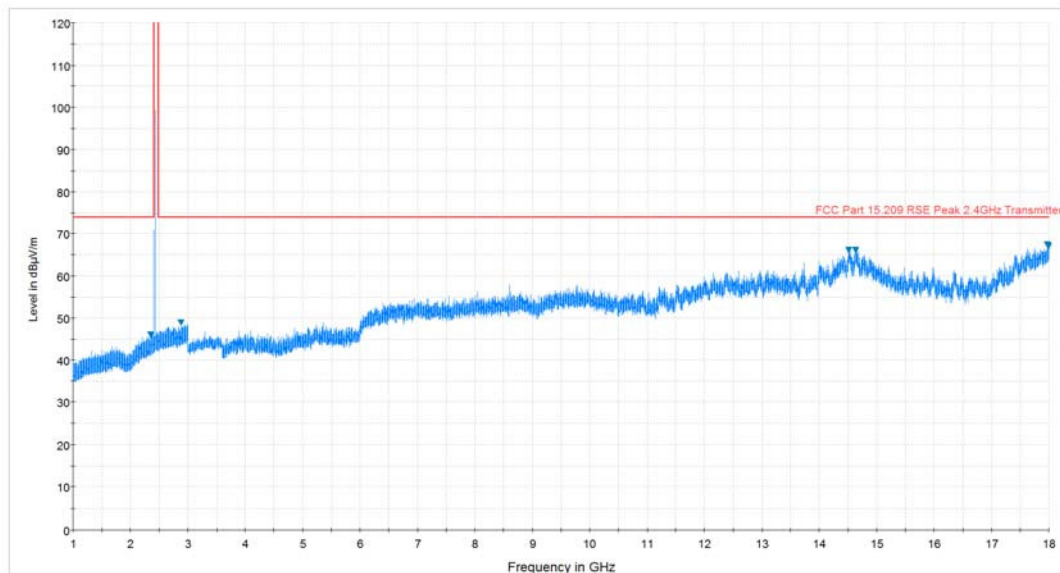
Plot 7-45. Radiated Spurious Plot above 1GHz (BT – Ch. 39, Ant. Pol. V)
