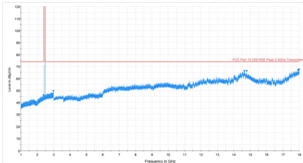
Plot 7-47. Radiated Spurious Plot above 1GHz (BT – Ch. 78, Ant. Pol. V)
