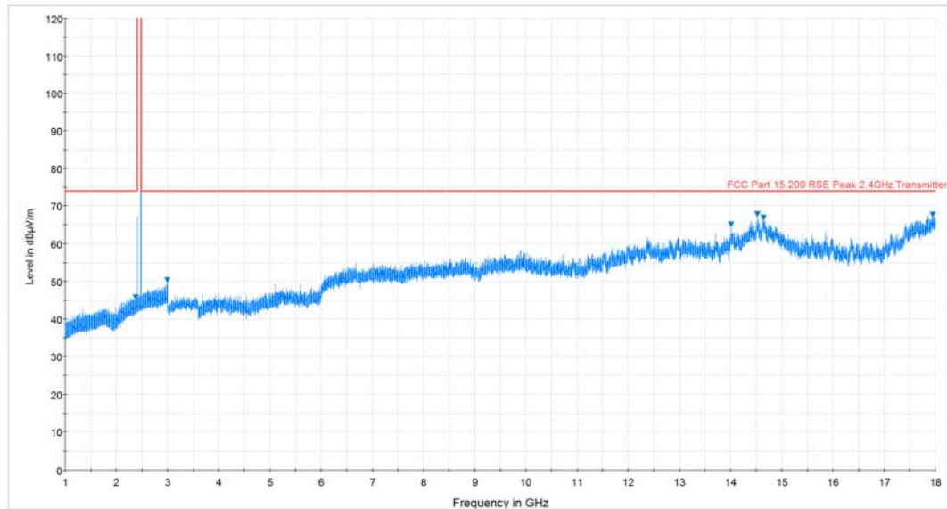
Plot 7-46. Radiated Spurious Plot above 1GHz (BT – Ch. 78, Ant. Pol. H)
