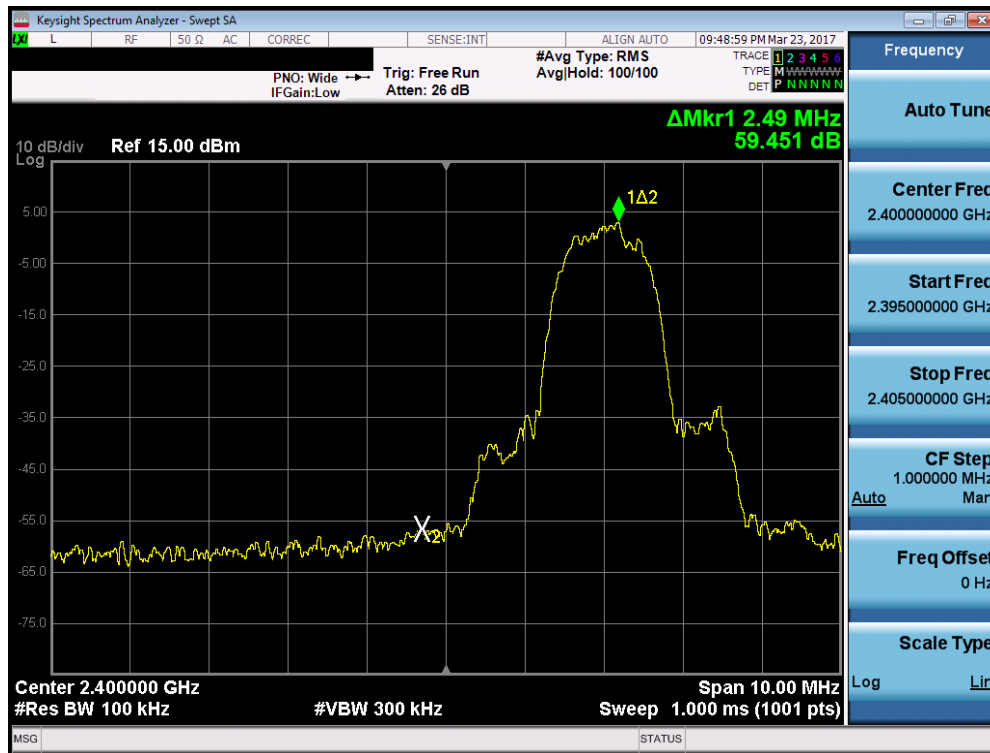
Plot 7-28. Band Edge Plot (Bluetooth with Hopping Disabled, 3 Mbps – Ch. 0)
