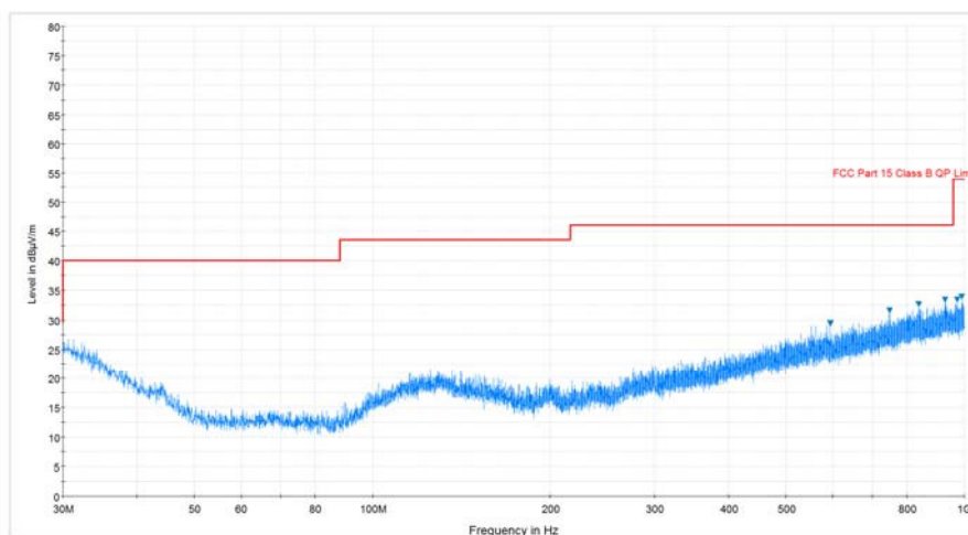
Plot 7-53. Radiated Spurious Plot below 1GHz (Pol. V)
