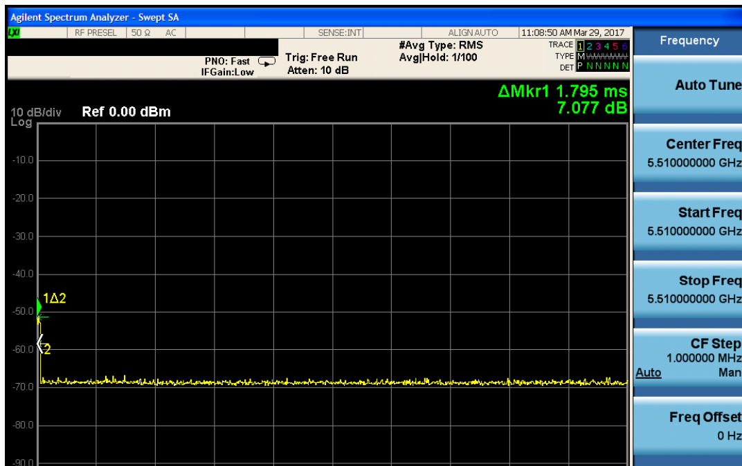
Figure 5-8. Band 2C Client Beacon Test – Monitoring live spectrum – Elapse time 10 minutes
