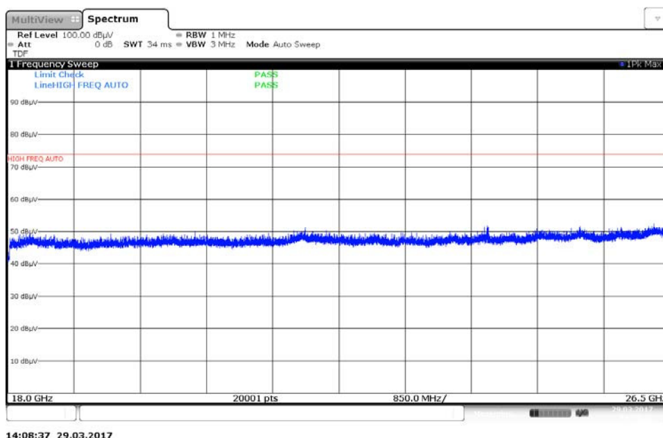
Plot 7-88. Radiated Spurious Plot above 18GHz - 26.5GHz (802.11a – Ant. Pol. V)
