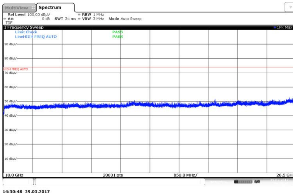
Plot 7-87. Radiated Spurious Plot 18GHz - 26.5GHz (802.11a – Ant. Pol. H)
