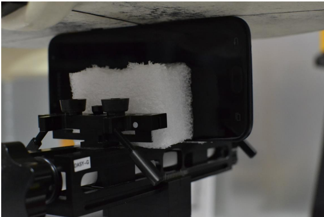
SAR Test Setup Photo 18- Right Edge at 0.0 cm (Phablet)
