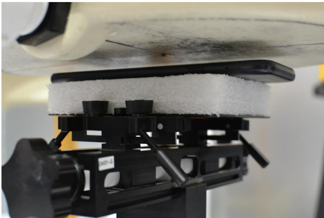
SAR Test Setup Photo 9- Front Side at 1.0 cm (Hotspot)
