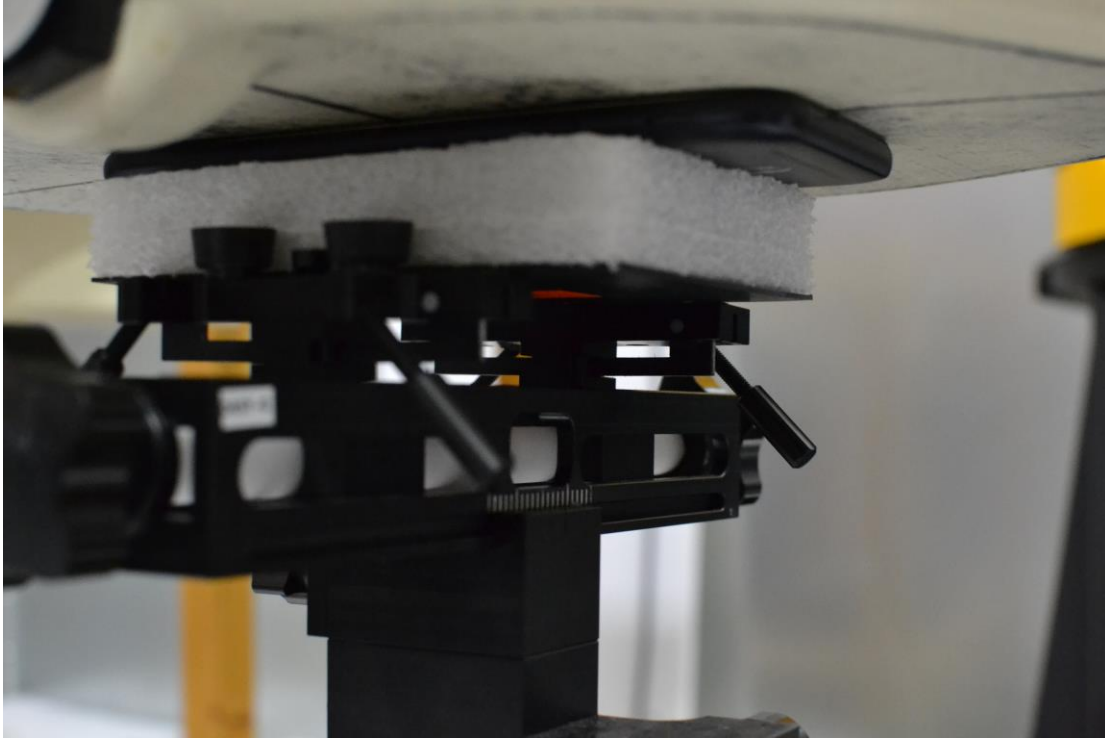
SAR Test Setup Photo 11- Front Side at 0.0 cm (Phablet)
