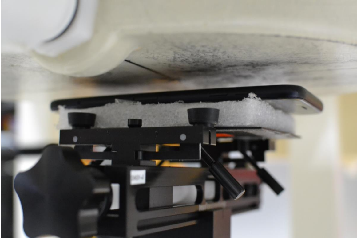
SAR Test Setup Photo 7- Back Side at 1.3 cm (Phablet)
