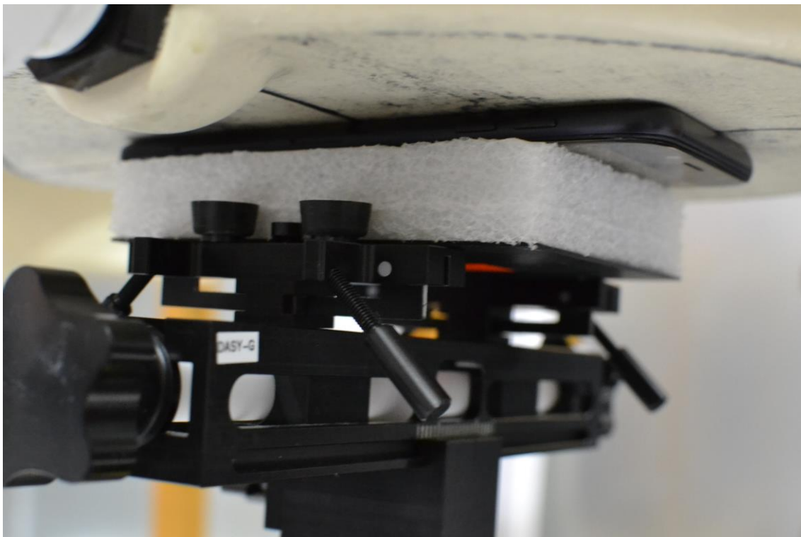
SAR Test Setup Photo 8- Back Side at 0.0 cm (Phablet)
