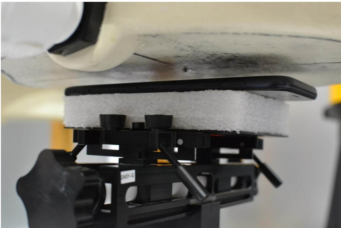
SAR Test Setup Photo 6- Back Side at 1.0 cm (Hotspot)
