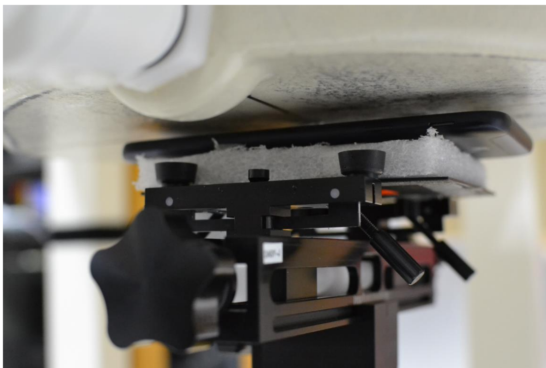
SAR Test Setup Photo 10- Front Side at 0.7 cm (Hotspot)
