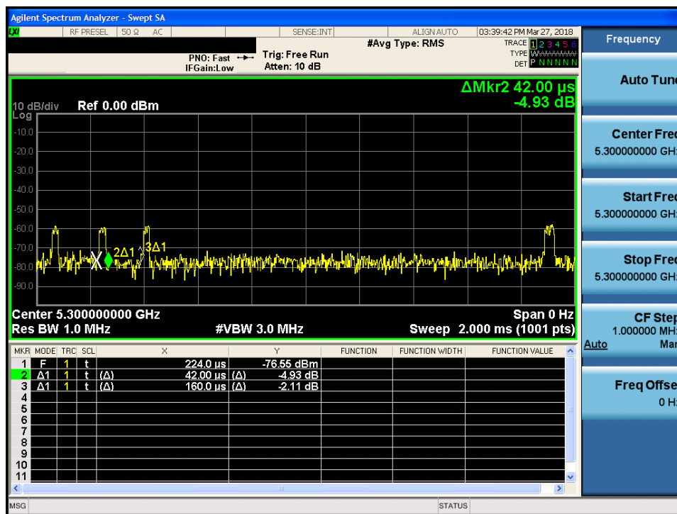
Figure 5-1. Band 2A Pulse Width & Period
