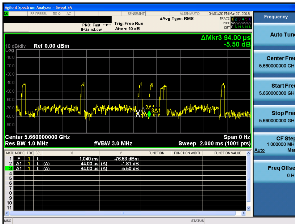
Figure 5-2. Band 2C Pulse Width & Period
