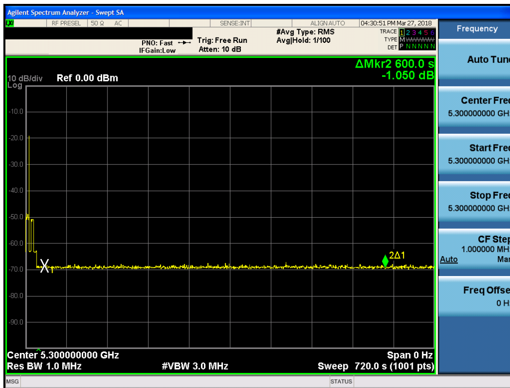
Figure 5-5. Band 2A Client Beacon Test – Monitoring live spectrum – Elapse time 10 minutes
