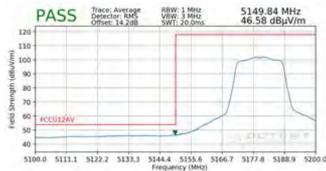
Plot 7-87. Radiated Lower Band Edge Plot (Average – UNII Band 1)
