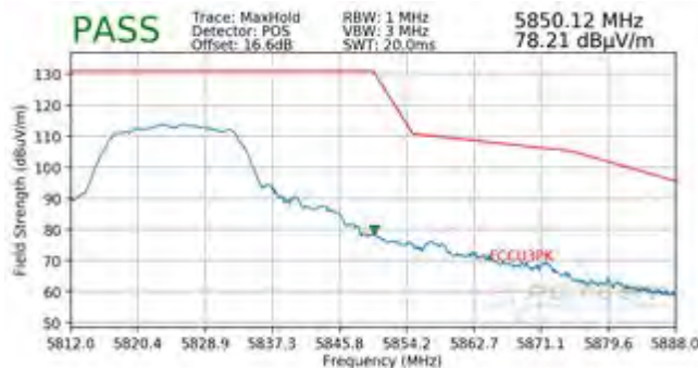
Plot 7-93. Radiated Upper Band Edge Plot (Peak – UNII Band 3)
