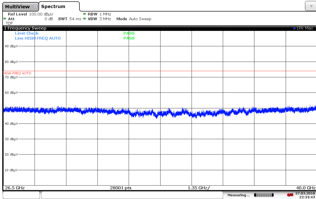
Plot 7-85. Radiated Spurious Plot 26.5GHz - 40GHz (802.11a) – Horizontal
