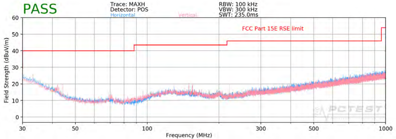
Plot 7-108. Radiated Spurious Plot below 1GHz (802.11a – U2C Ch. 120)
