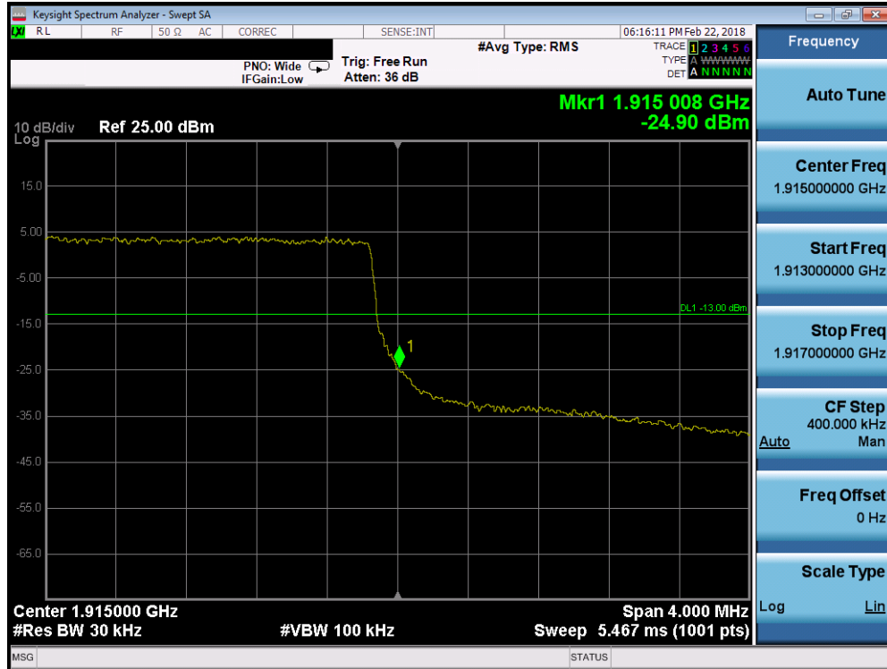
Plot 7-148. Upper Band Edge Plot (Band 25 - 3.0MHz QPSK - Full RB Configuration)
