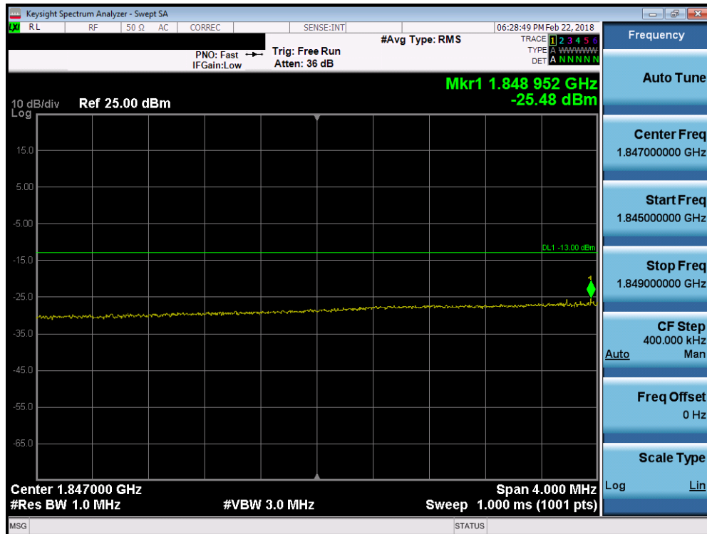
Plot 7-163. Lower Extended Band Edge Plot (Band 25/2 - 15.0MHz QPSK - Full RB Configuration)
