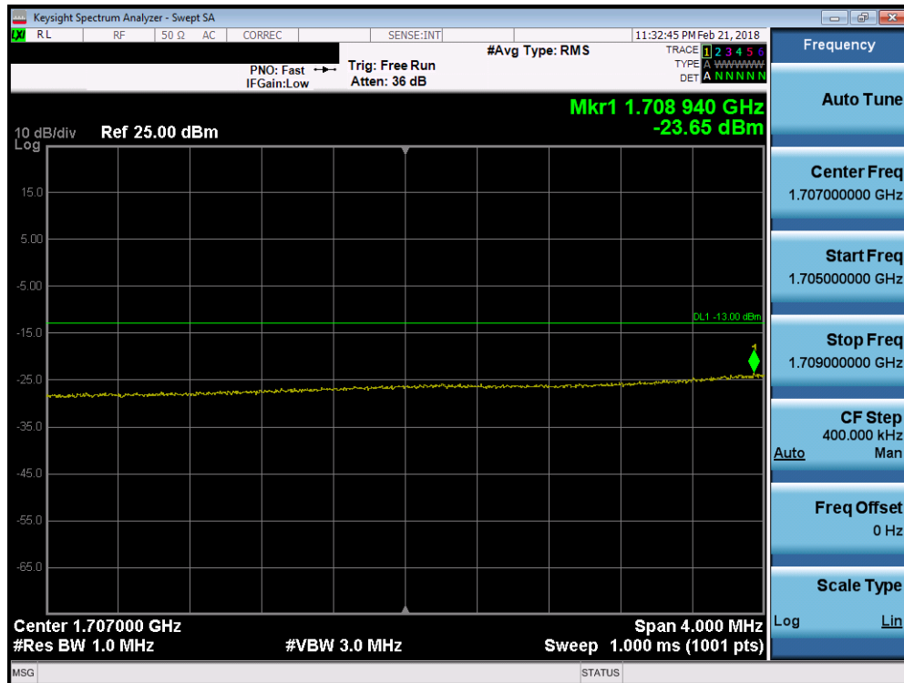
Plot 7-131. Lower Extended Band Edge Plot (Band 4 - 15.0MHz QPSK - Full RB Configuration)
