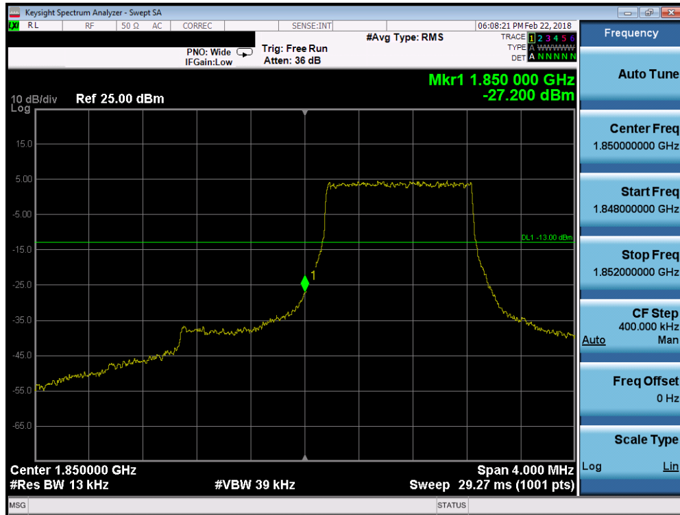
Plot 7-138. Lower Band Edge Plot (Band 25/2 - 1.4MHz QPSK - Full RB Configuration)
