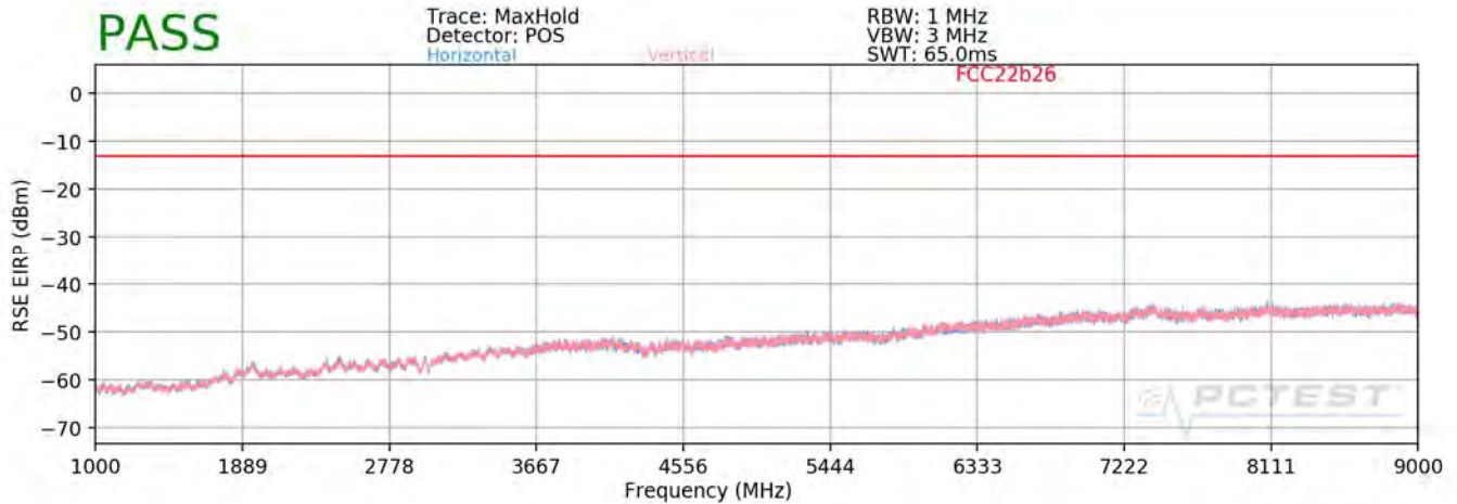
Plot 7-203. Radiated Spurious Plot above 1GHz (Band 26/5)
