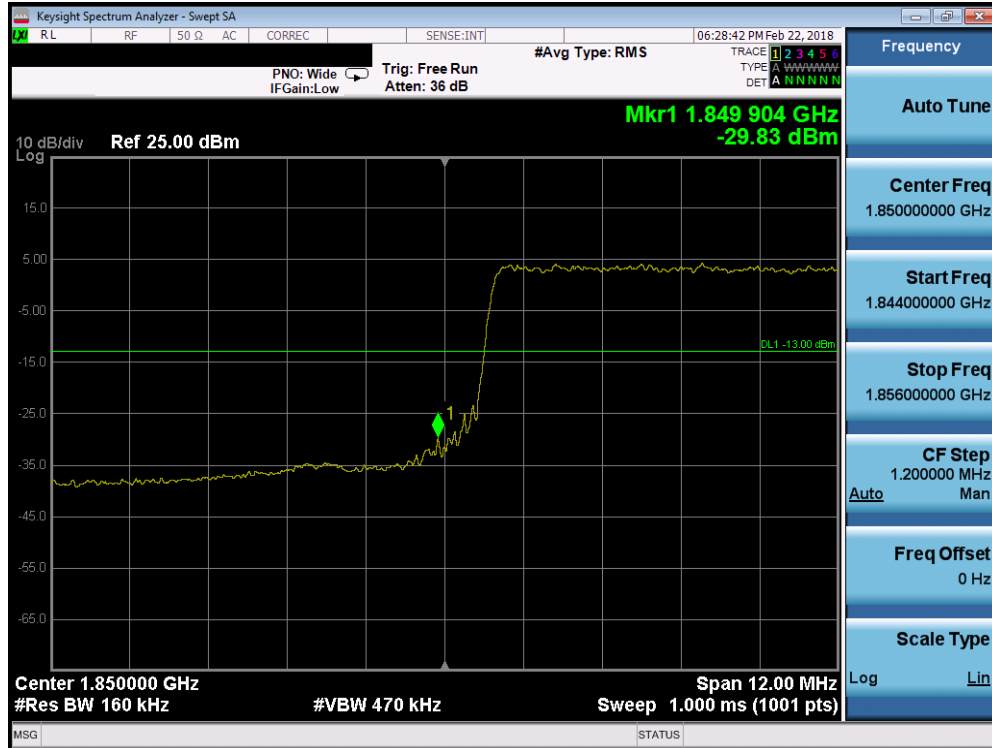
Plot 7-162. Lower Band Edge Plot (Band 25/2 - 15.0MHz QPSK - Full RB Configuration)
