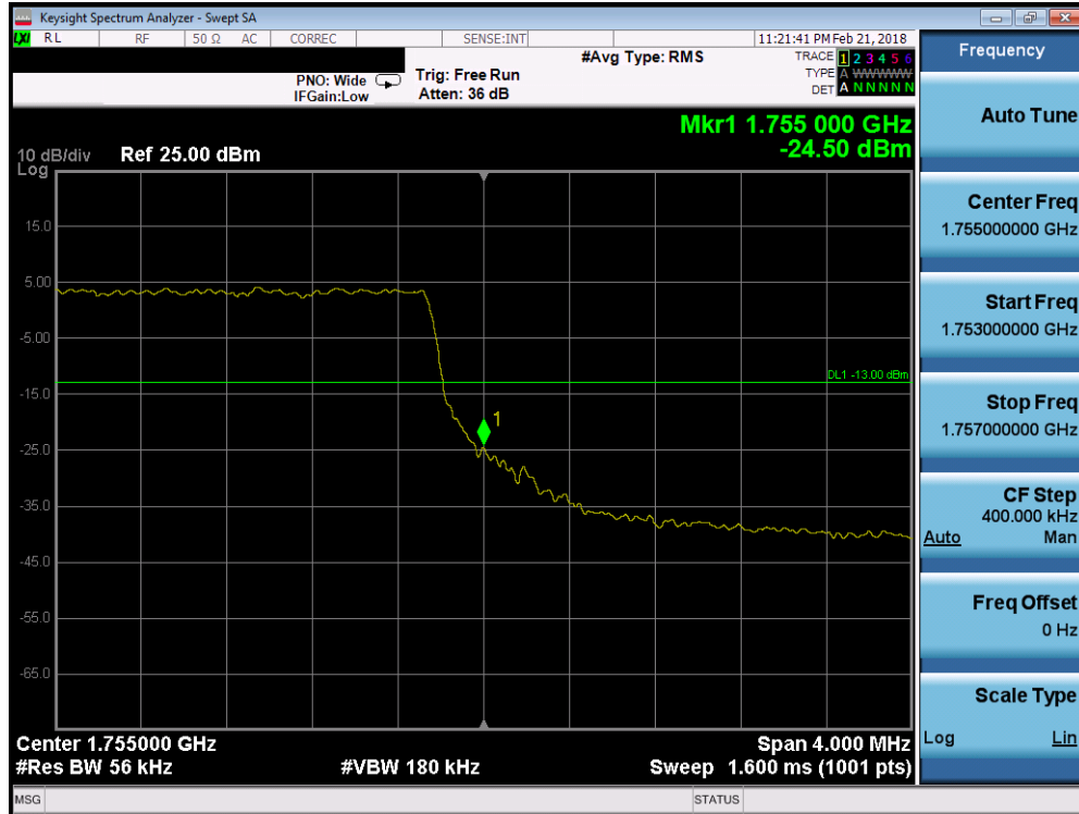
Plot 7-124. Upper Band Edge Plot (Band 4 - 5.0MHz QPSK - Full RB Configuration)
