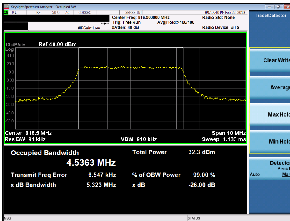
Plot 7-7. Occupied Bandwidth Plot (LTE B26 – 5MHz QPSK – RB Size 25– Low Channel)
