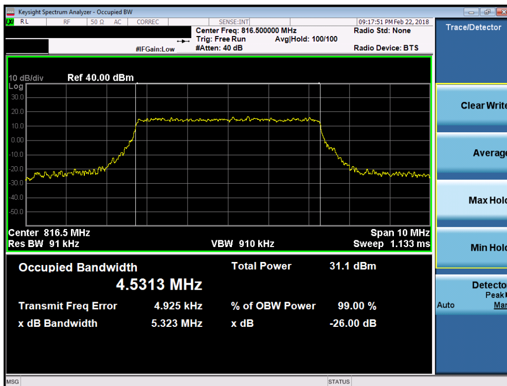
Plot 7-8. Occupied Bandwidth Plot (LTE B26 – 5MHz 16-QAM – RB Size 25– Low Channel)
