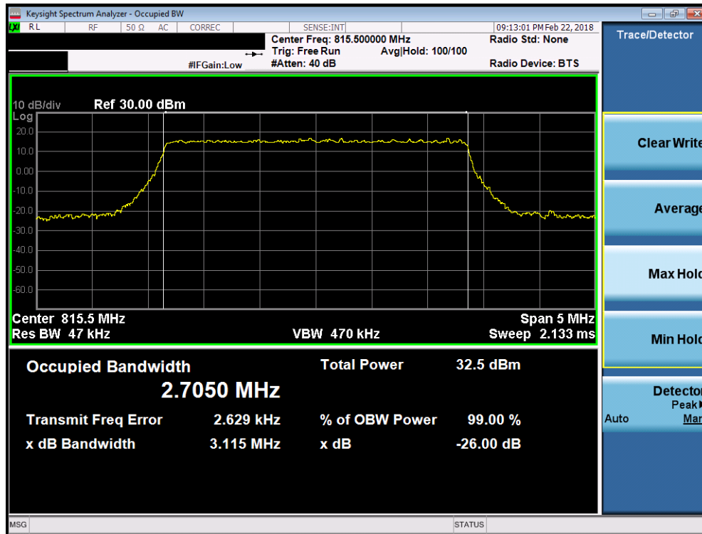
Plot 7-5. Occupied Bandwidth Plot (LTE B26 – 3MHz QPSK – RB Size 15– Low Channel)
