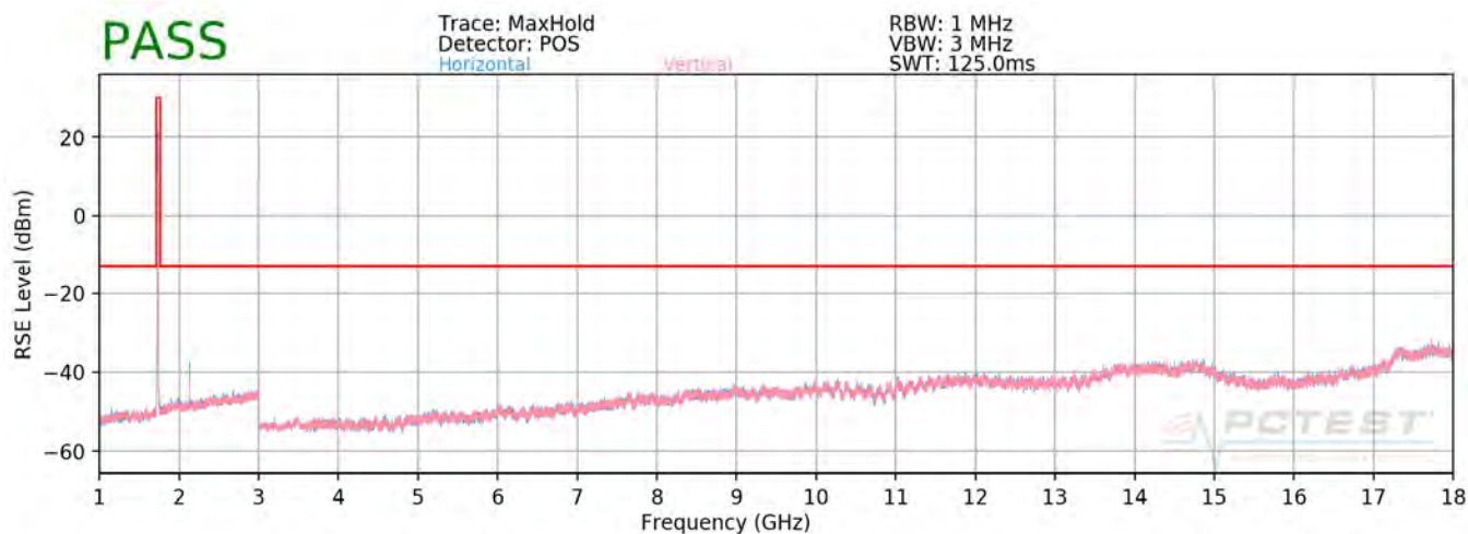
Plot 7-109. Radiated Spurious Plot Above 1GHz (AWS WCDMA Mode)
