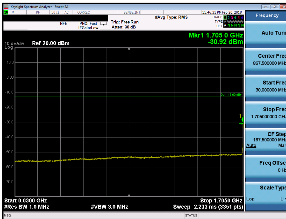
Plot 7-55. Conducted Spurious Plot (AWS WCDMA Mode - Low Channel)
