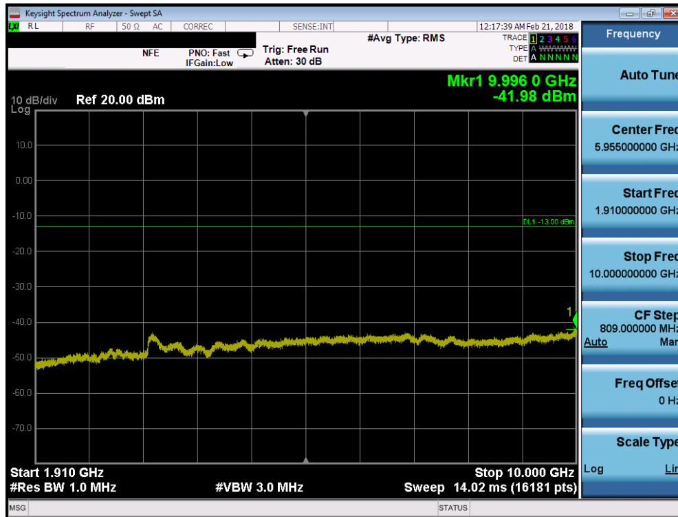
Plot 7-41. Conducted Spurious Plot (PCS CDMA Mode - Mid Channel)
