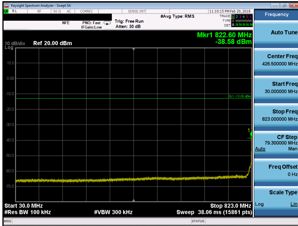
Plot 7-46. Conducted Spurious Plot (Cellular WCDMA Mode - Low Channel)
