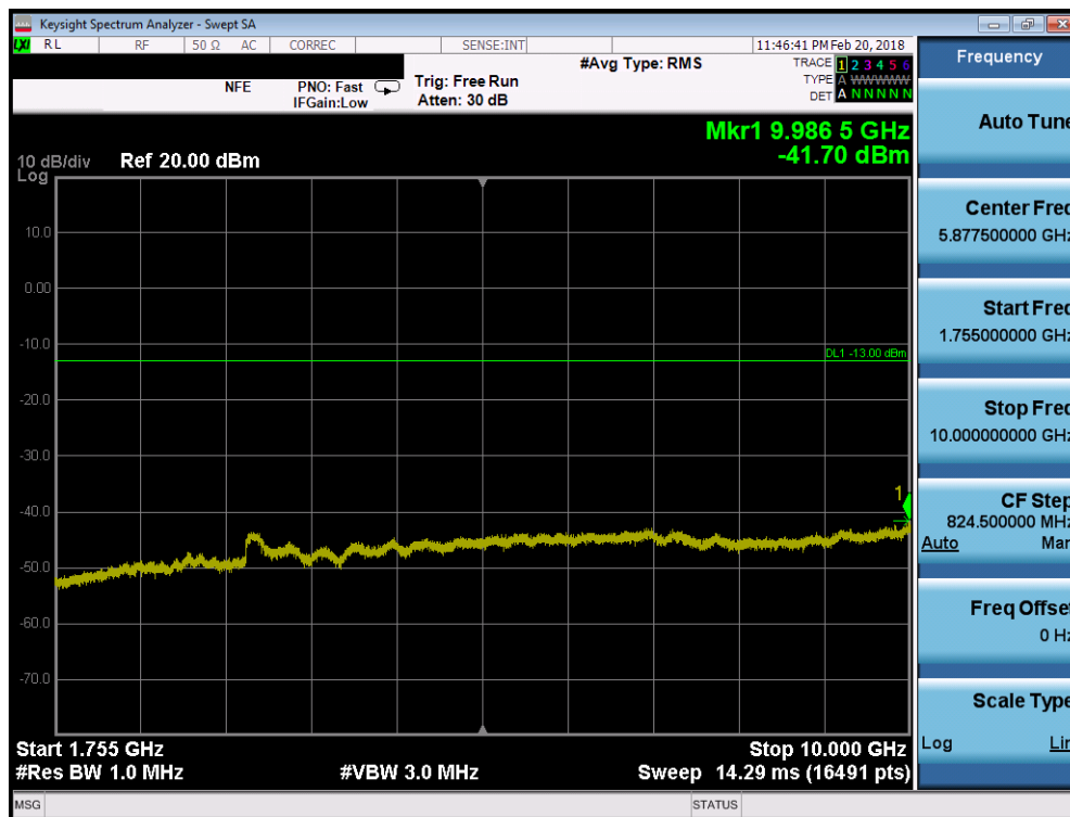
Plot 7-56. Conducted Spurious Plot (AWS WCDMA Mode - Low Channel)
