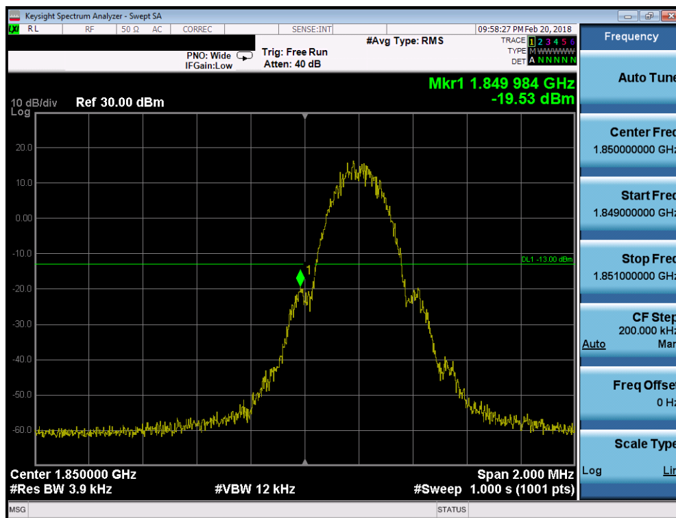
Plot 7-75. Band Edge Plot (PCS GPRS Mode - Low Channel)
