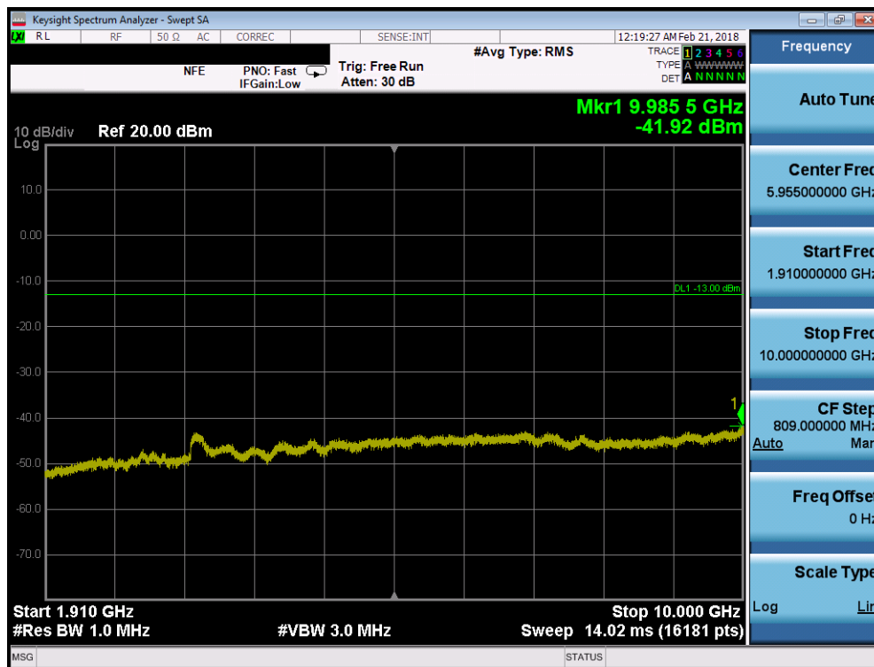
Plot 7-38. Conducted Spurious Plot (PCS CDMA Mode - Low Channel)
