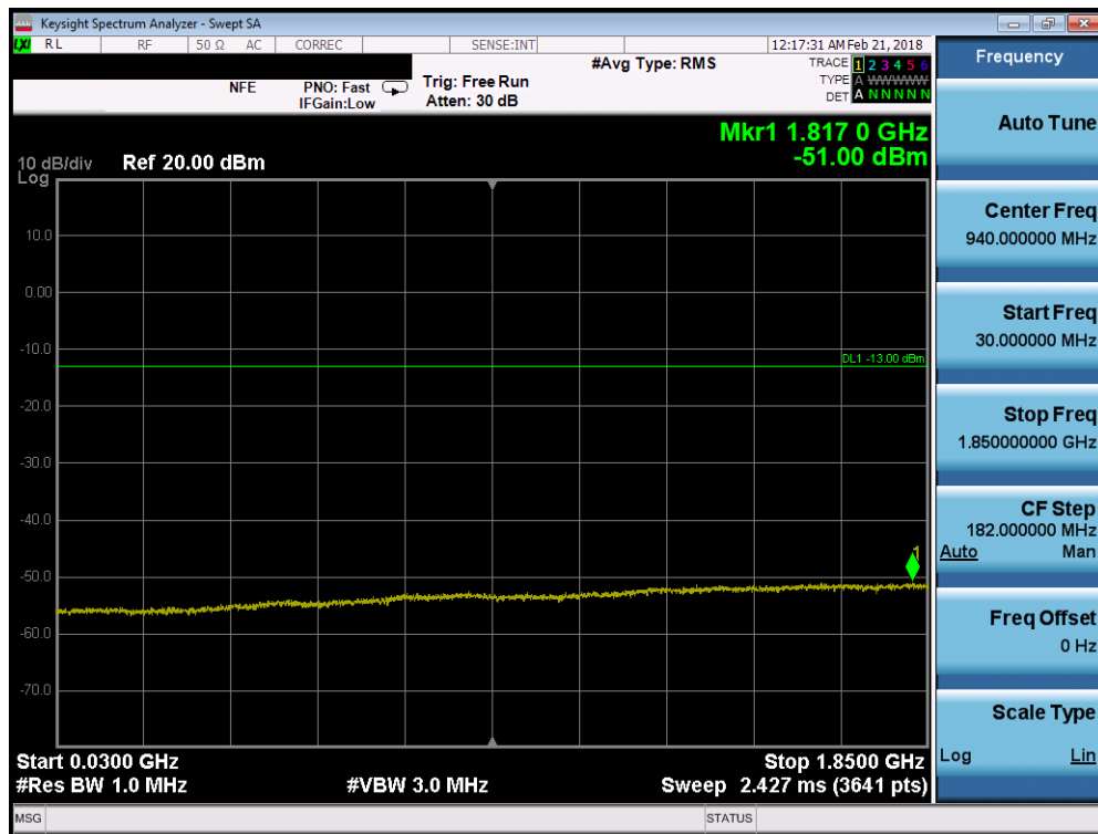
Plot 7-40. Conducted Spurious Plot (PCS CDMA Mode - Mid Channel)
