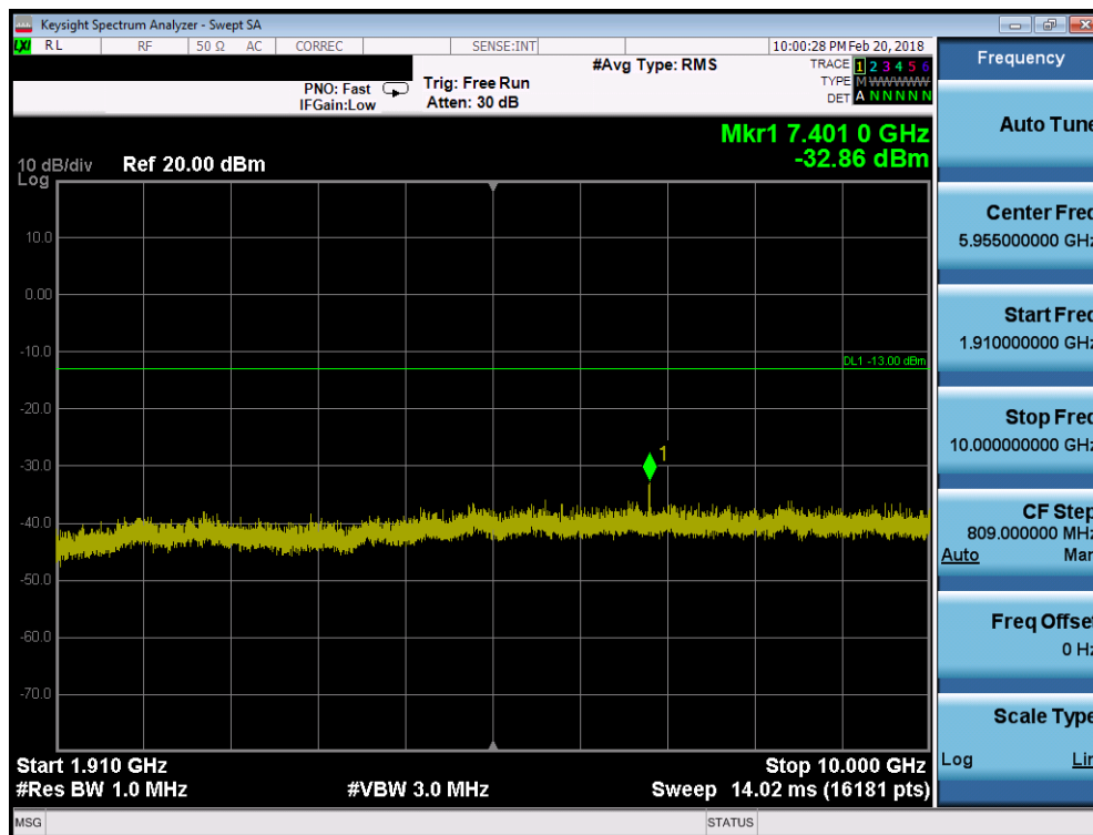
Plot 7-20. Conducted Spurious Plot (PCS GPRS Mode - Low Channel)
