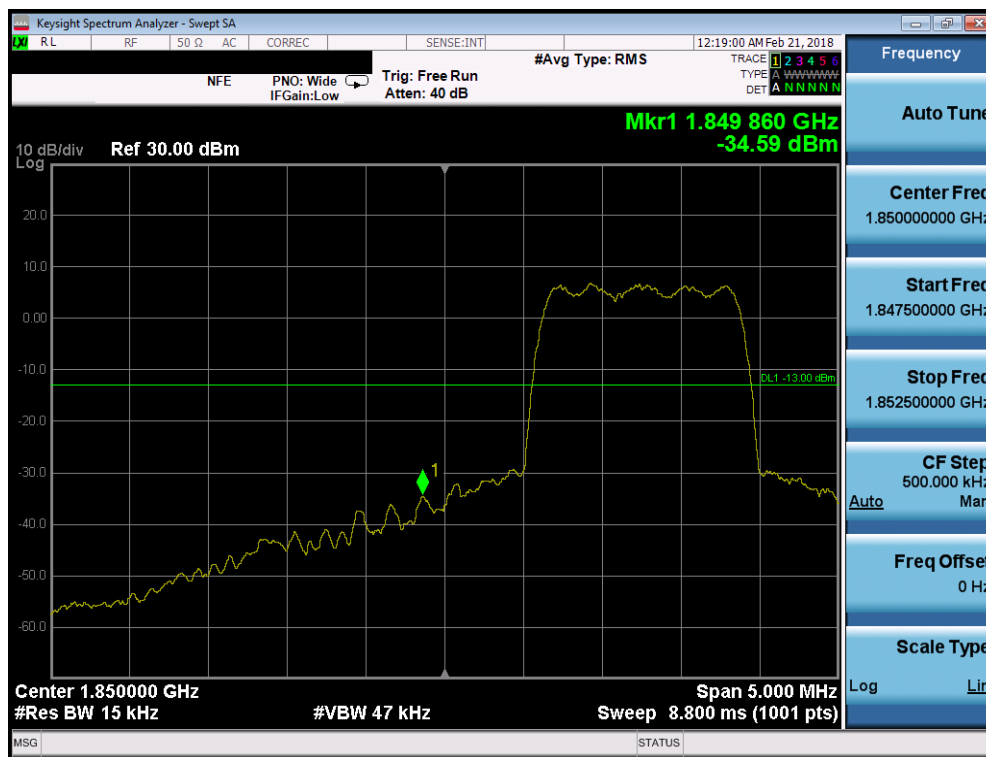
Plot 7-83. Band Edge Plot (PCS CDMA Mode - Low Channel)
