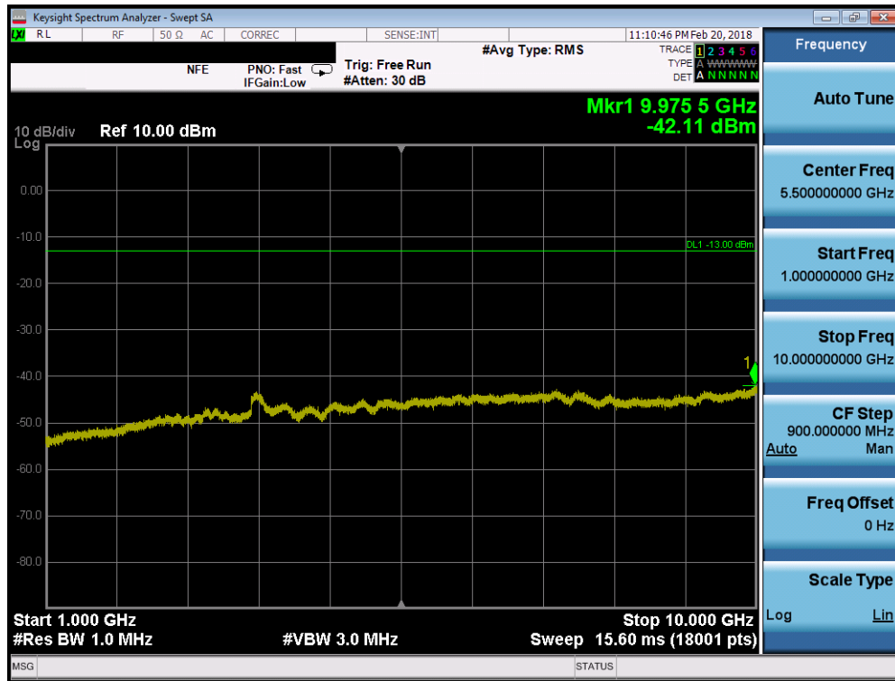
Plot 7-48. Conducted Spurious Plot (Cellular WCDMA Mode - Low Channel)
