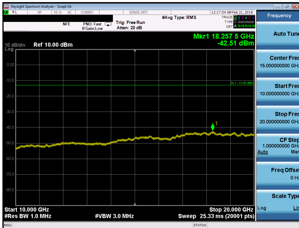
Plot 7-42. Conducted Spurious Plot (PCS CDMA Mode - Mid Channel)
