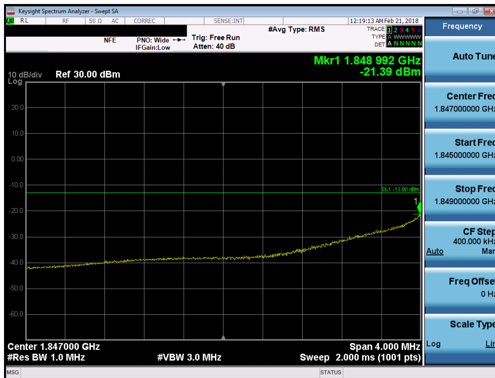
Plot 7-84. 4MHz Span Plot (PCS CDMA Mode - Low Channel)
