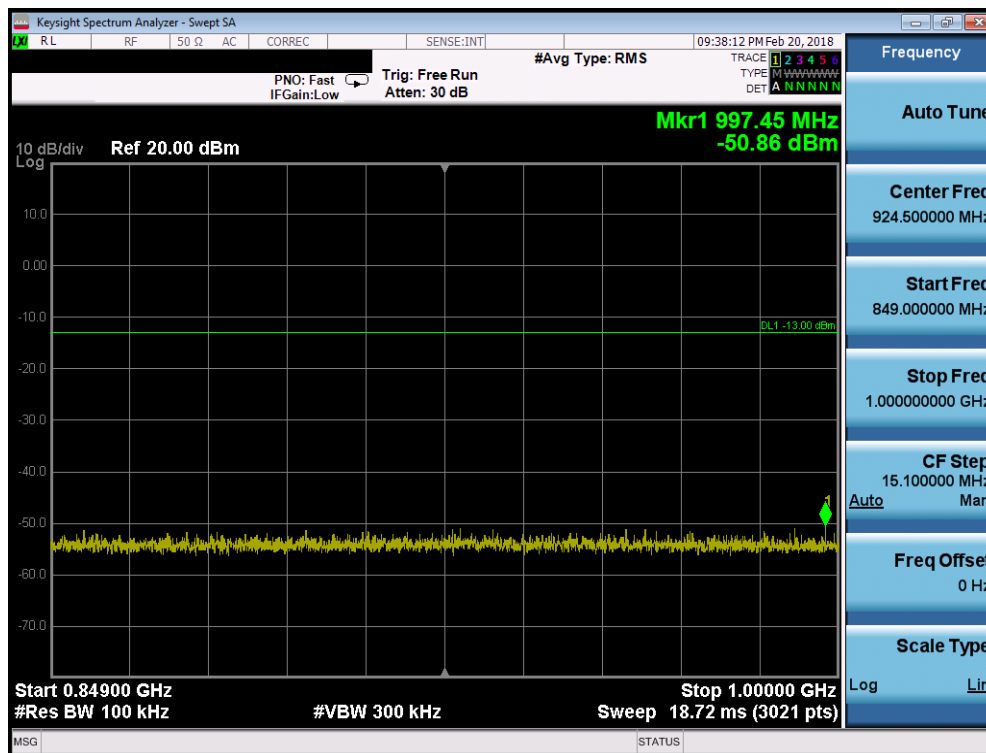
Plot 7-11. Conducted Spurious Plot (Cellular GPRS Mode - Low Channel)
