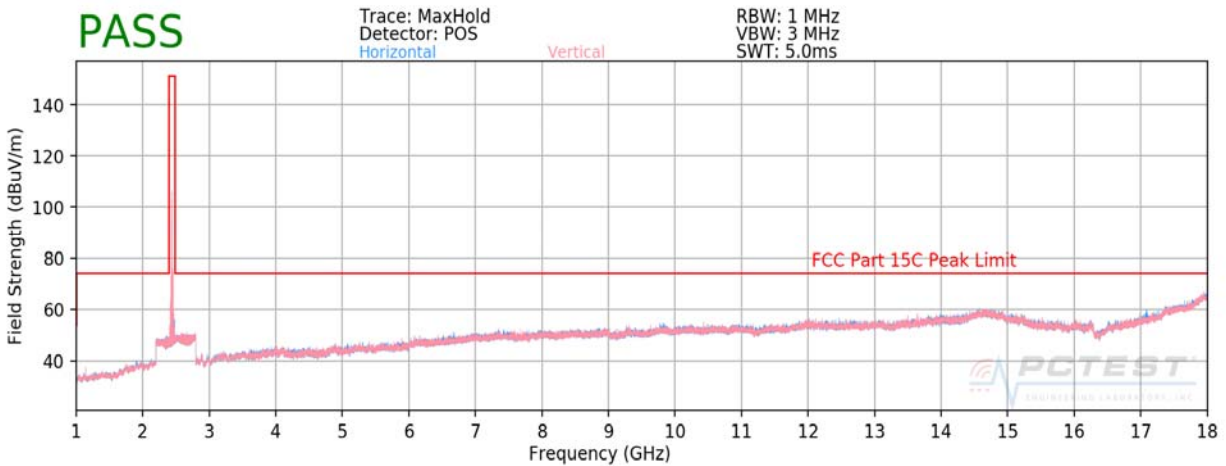
Plot 7-43. Radiated Spurious Plot above 1GHz (BT – Ch. 39)
