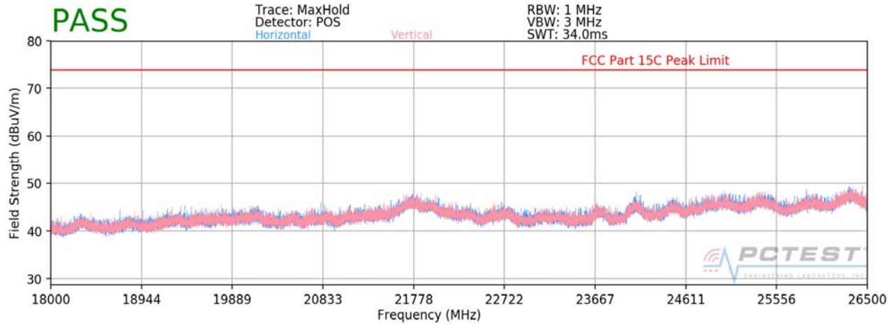
Plot 7-45. Radiated Spurious Plot above 18GHz
