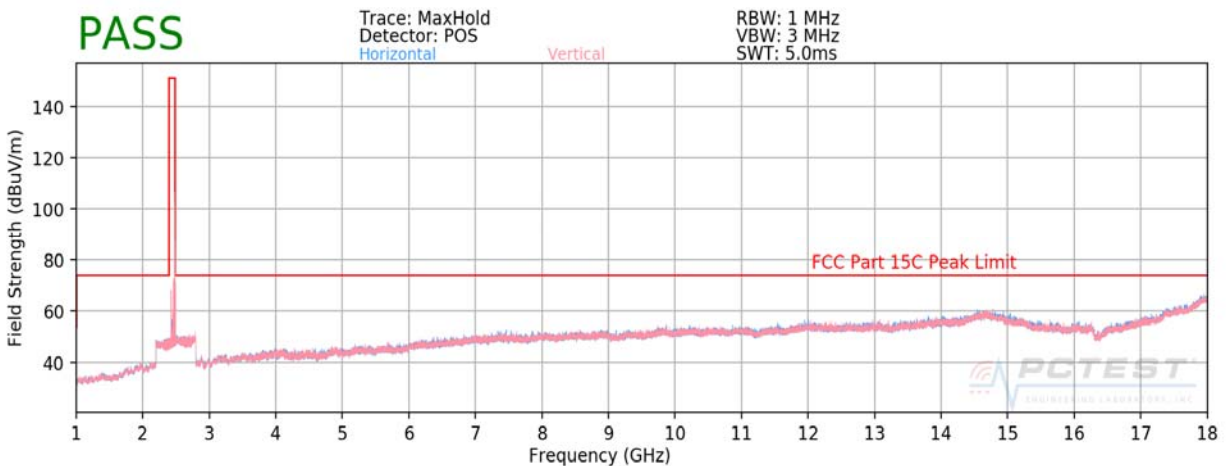
Plot 7-44. Radiated Spurious Plot above 1GHz (BT – Ch. 78)
