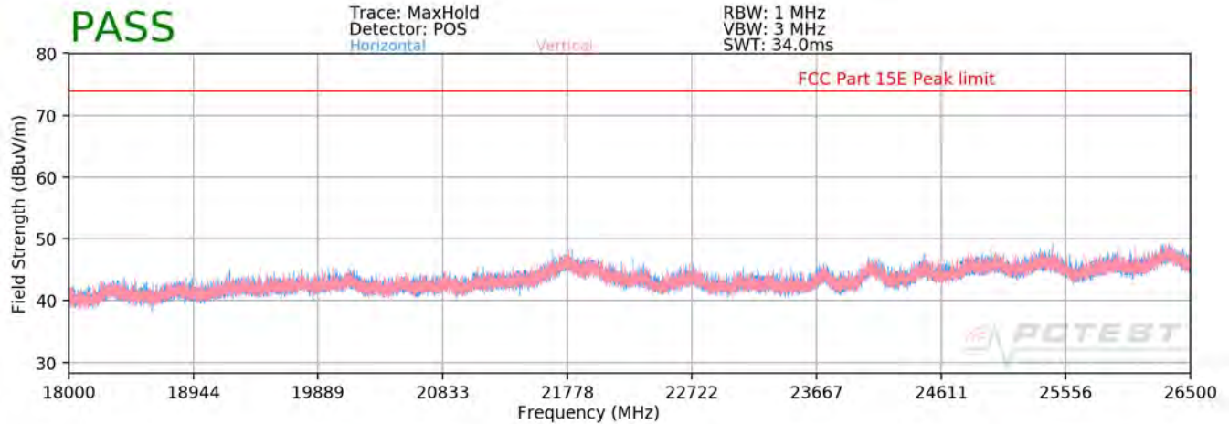
Plot 7-83. Radiated Spurious Plot 18GHz - 26.5GHz (802.11a)
