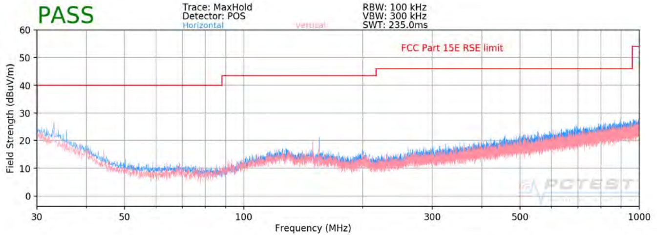
Plot 7-107. Radiated Spurious Plot below 1GHz (802.11a – U3 Ch. 157)
