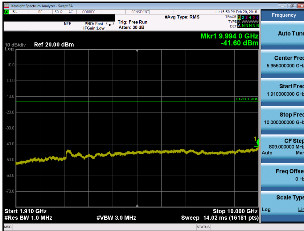
Plot 7-58. Conducted Spurious Plot (PCS WCDMA Mode - Mid Channel)
