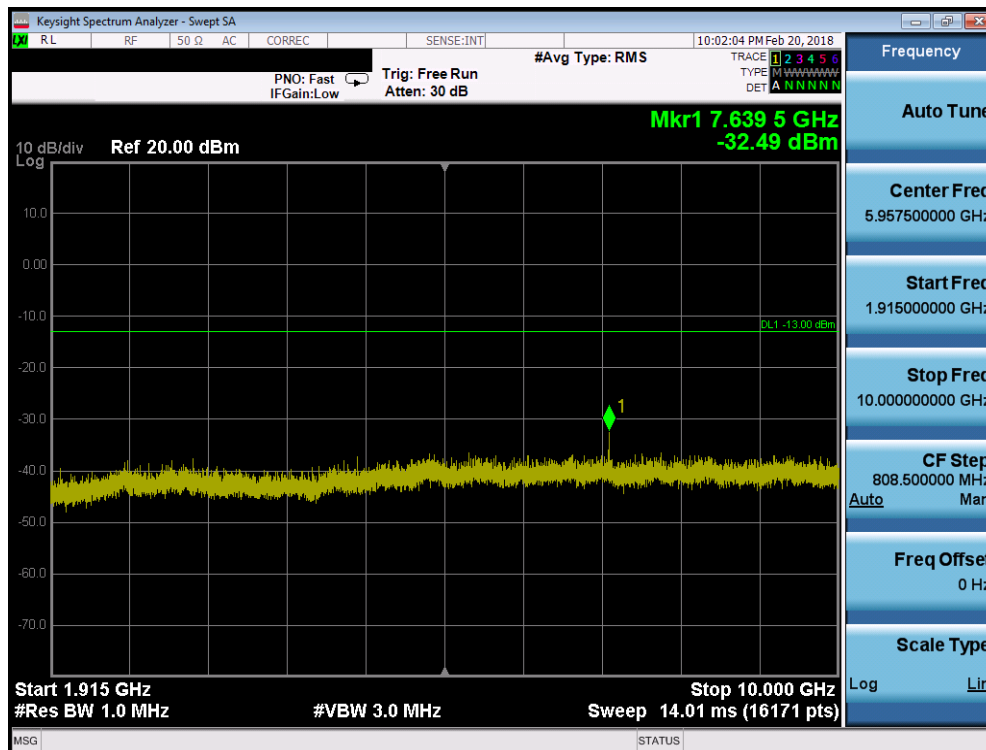
Plot 7-25. Conducted Spurious Plot (PCS GPRS Mode - High Channel)
