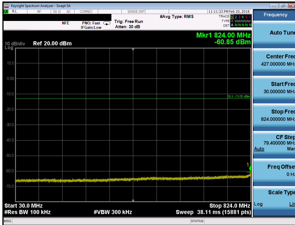
Plot 7-51. Conducted Spurious Plot (Cellular WCDMA Mode - High Channel)
