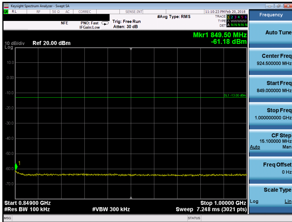
Plot 7-46. Conducted Spurious Plot (Cellular WCDMA Mode - Low Channel)W
