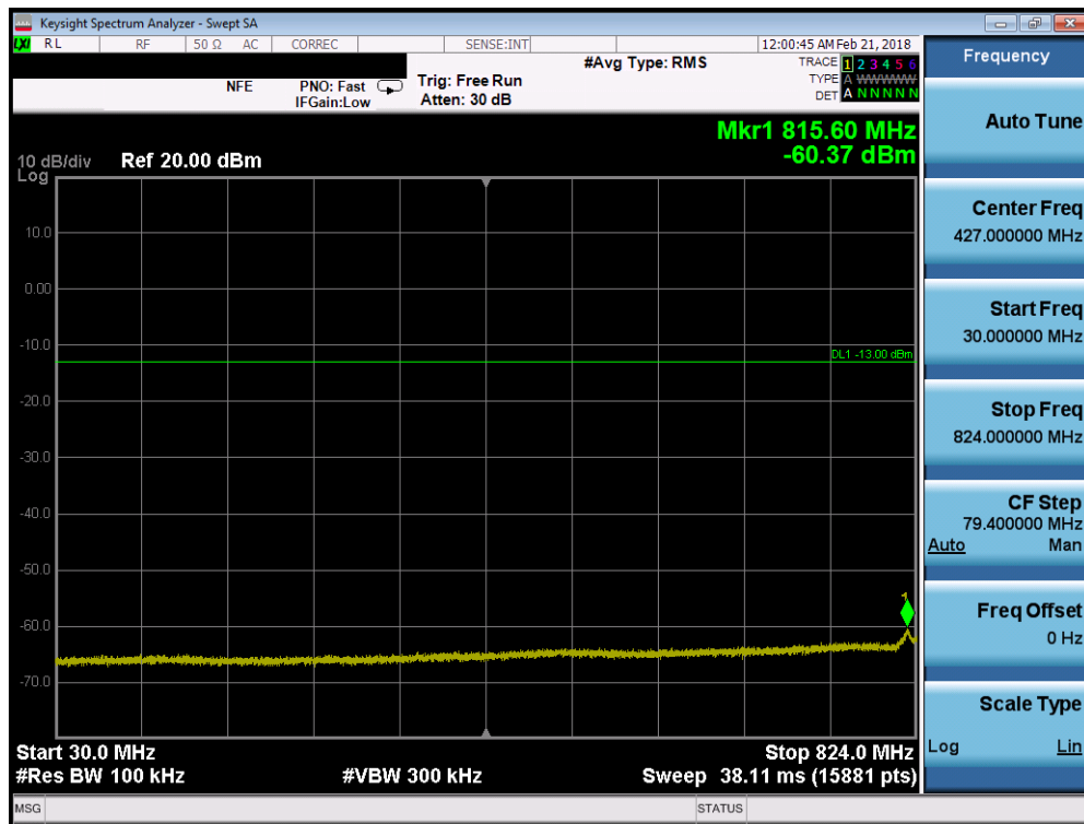
Plot 7-30. Conducted Spurious Plot (Cellular CDMA Mode - Mid Channel)
