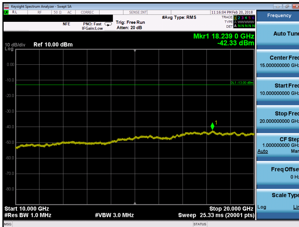
Plot 7-59. Conducted Spurious Plot (PCS WCDMA Mode - Mid Channel)
