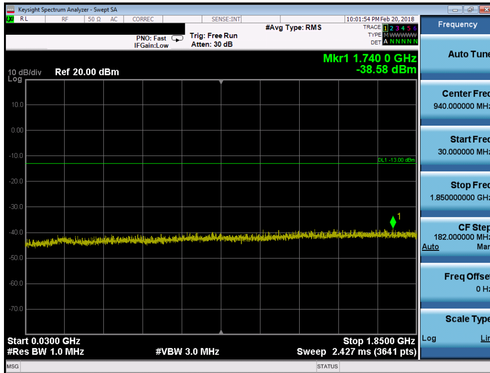
Plot 7-24. Conducted Spurious Plot (PCS GPRS Mode - High Channel)
