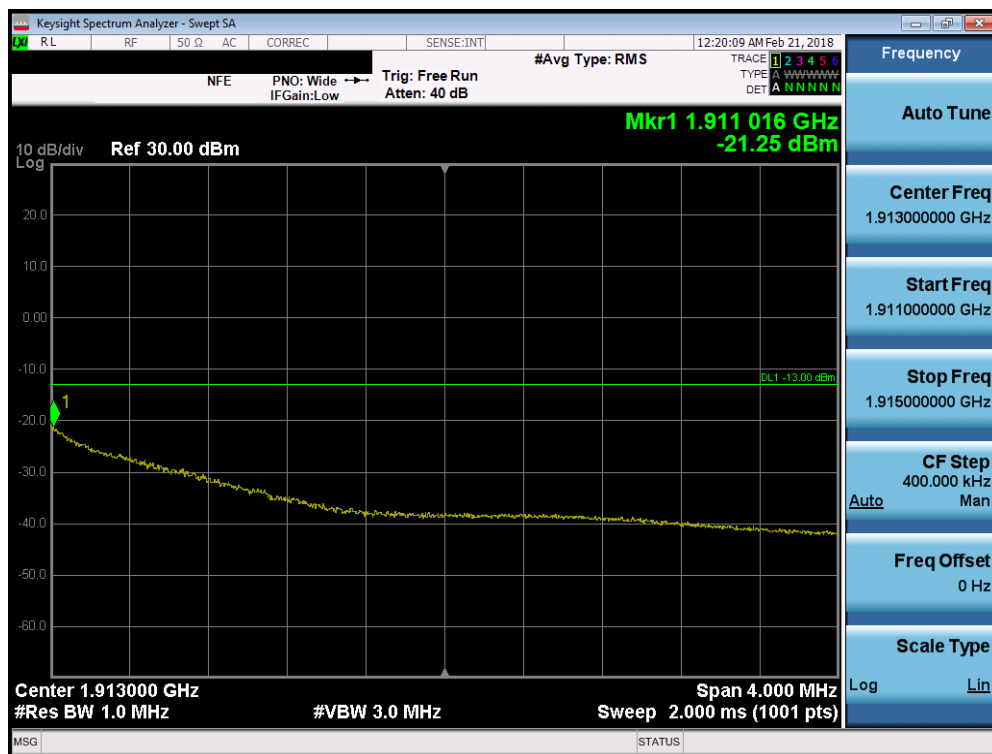
Plot 7-76. 4MHz Span Plot (PCS CDMA Mode - High Channel)
