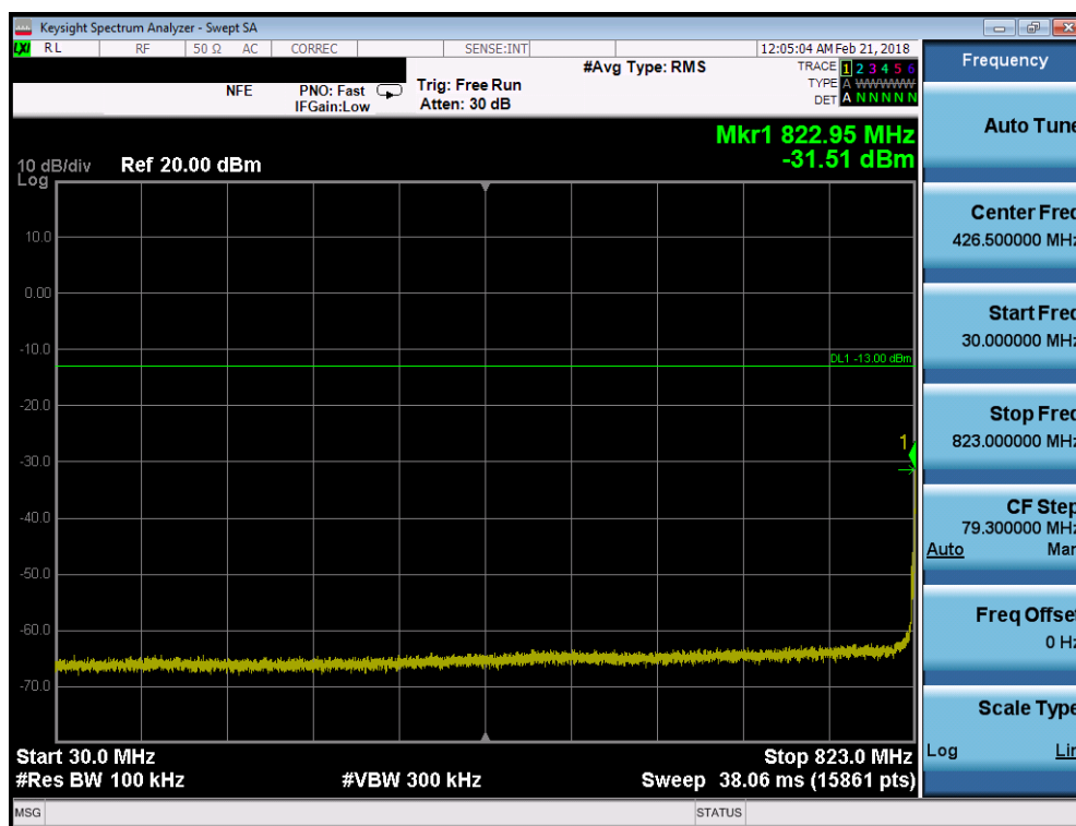
Plot 7-27. Conducted Spurious Plot (Cellular CDMA Mode - Low Channel)
