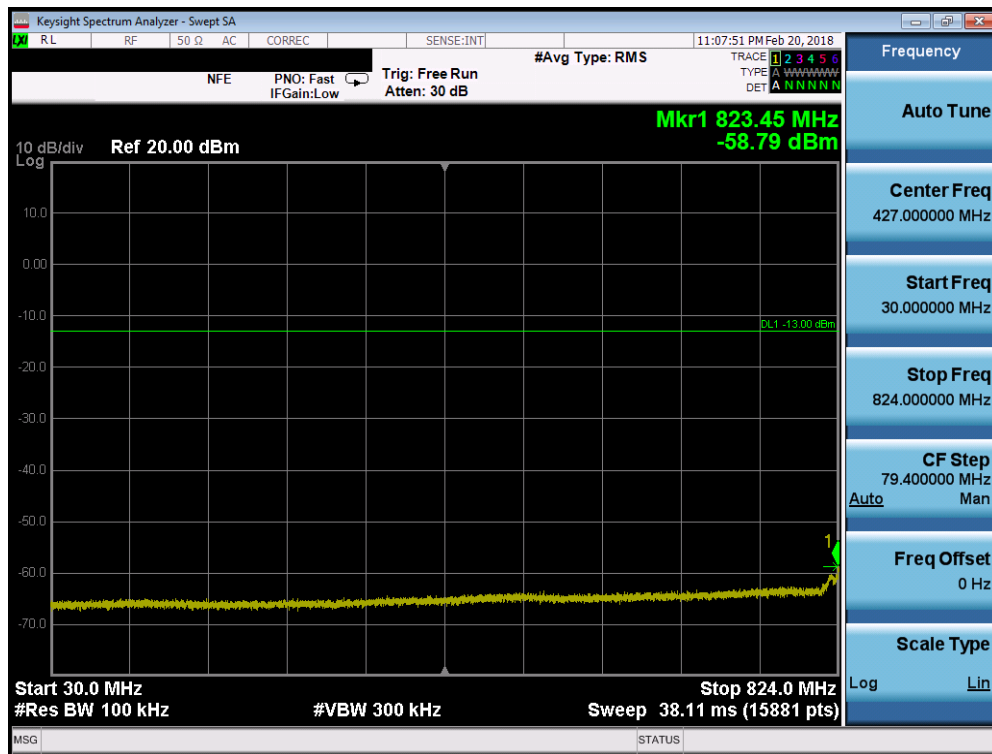
Plot 7-48. Conducted Spurious Plot (Cellular WCDMA Mode - Mid Channel)
