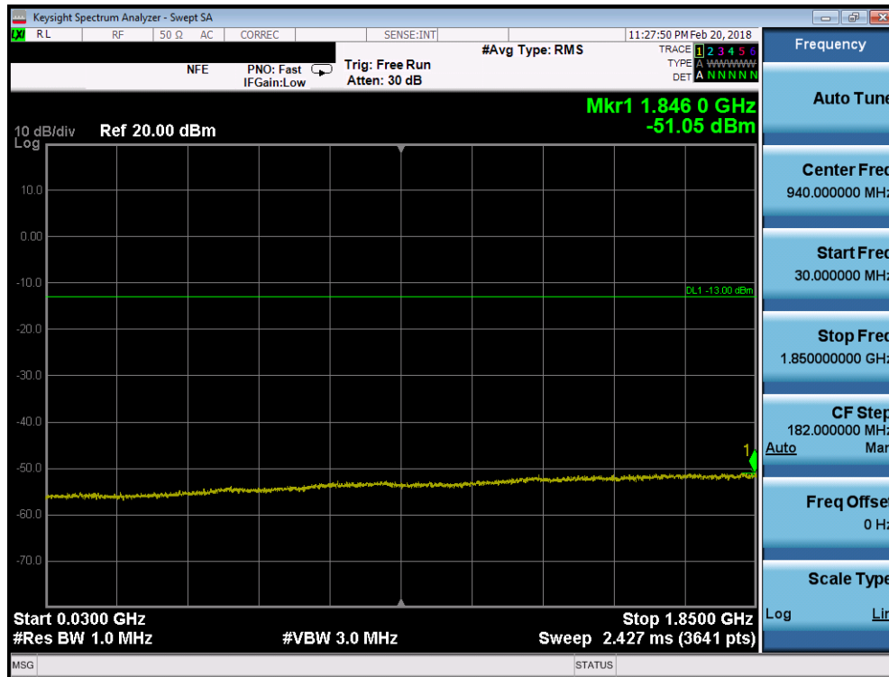
Plot 7-60. Conducted Spurious Plot (PCS WCDMA Mode - High Channel)
