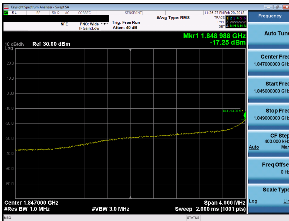
Plot 7-80. 4MHz Span Plot (PCS WCDMA Mode - Low Channel)
