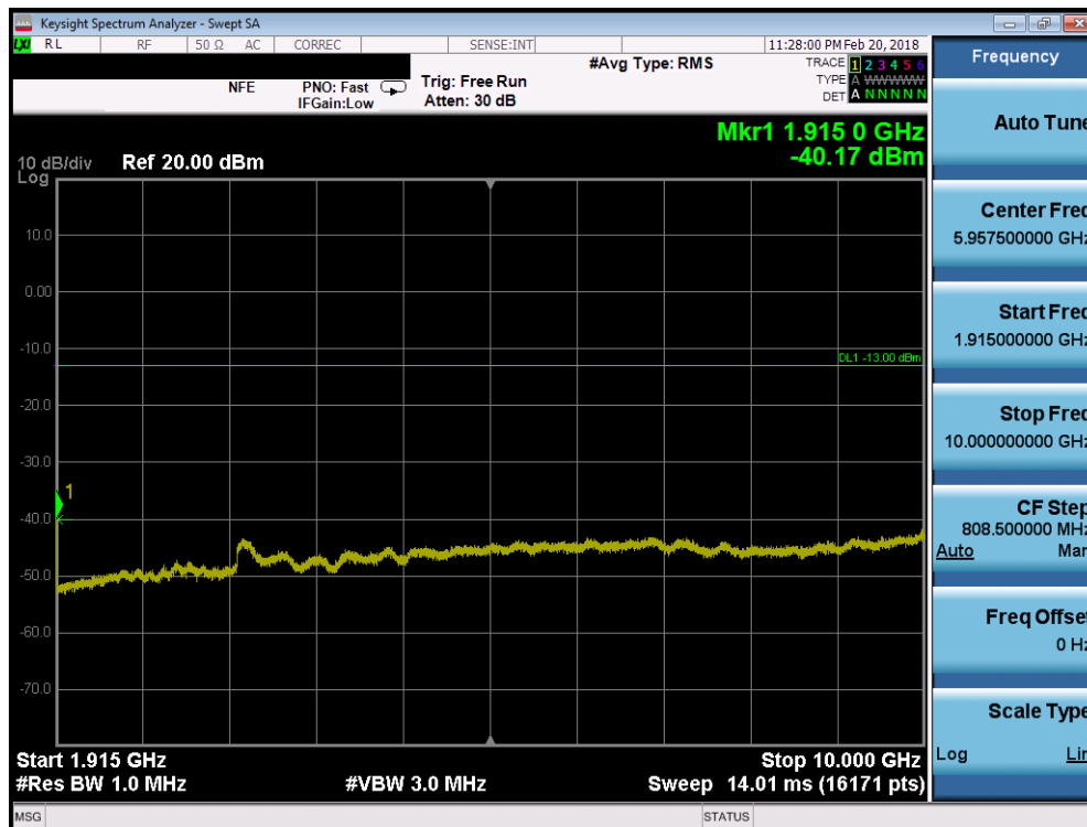
Plot 7-61. Conducted Spurious Plot (PCS WCDMA Mode - High Channel)
