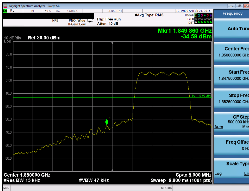
Plot 7-73. Band Edge Plot (PCS CDMA Mode - Low Channel)
