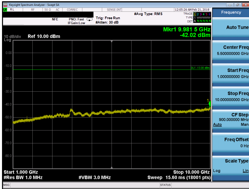
Plot 7-29. Conducted Spurious Plot (Cellular CDMA Mode - Low Channel)
