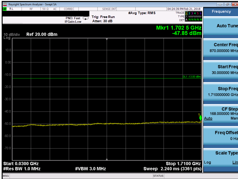
Plot 7-65. Conducted Spurious Plot (Band 4 - 1.4MHz QPSK - RB Size 1, RB Offset 0 - High Channel)
