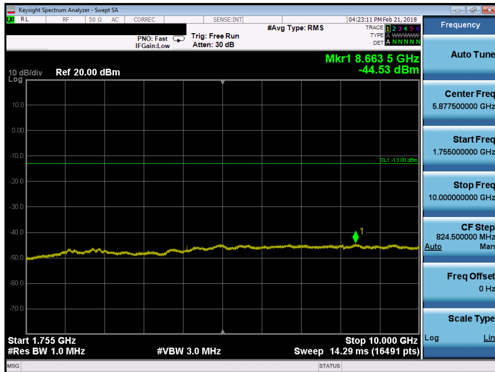
Plot 7-60. Conducted Spurious Plot (Band 4 - 1.4MHz QPSK - RB Size 1, RB Offset 0 - Low Channel)
