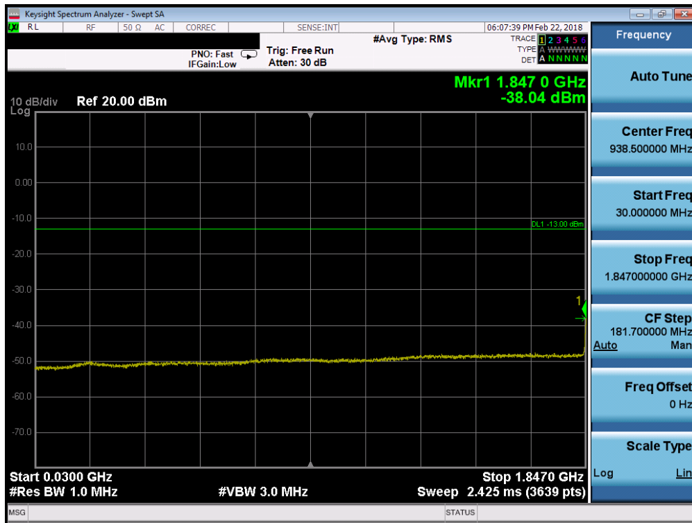
Plot 7-68. Conducted Spurious Plot (Band 25/2 - 1.4MHz QPSK - RB Size 1, RB Offset 0 - Low Channel)
