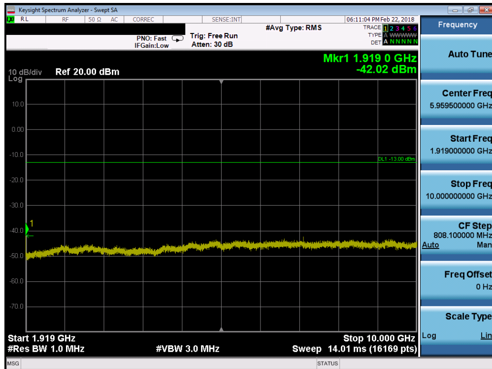
Plot 7-75. Conducted Spurious Plot (Band 25/2 - 1.4MHz QPSK - RB Size 1, RB Offset 0 - High Channel)
