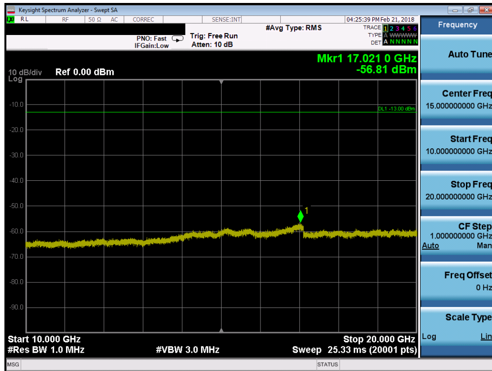
Plot 7-67. Conducted Spurious Plot (Band 4 - 1.4MHz QPSK - RB Size 1, RB Offset 0 - High Channel)
