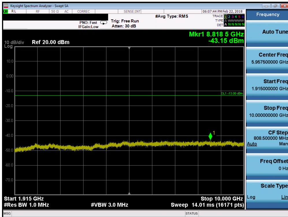
Plot 7-69. Conducted Spurious Plot (Band 25/2 - 1.4MHz QPSK - RB Size 1, RB Offset 0 - Low Channel)
