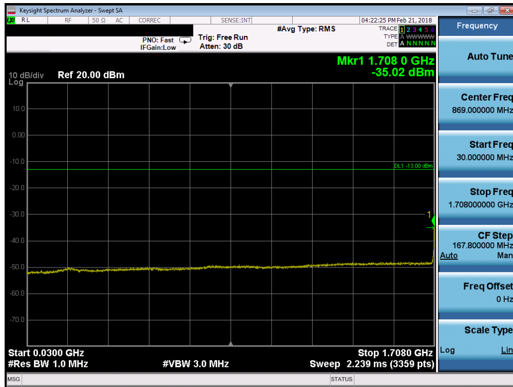
Plot 7-59. Conducted Spurious Plot (Band 4 - 1.4MHz QPSK - RB Size 1, RB Offset 0 - Low Channel)
