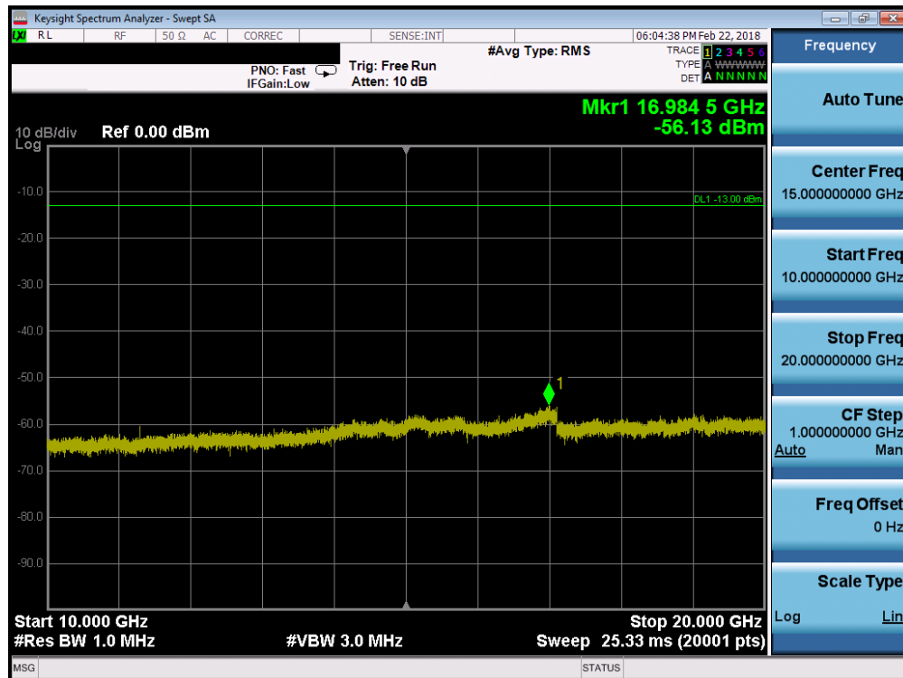
Plot 7-73. Conducted Spurious Plot (Band 25/2 - 1.4MHz QPSK - RB Size 1, RB Offset 0 - Mid Channel)
