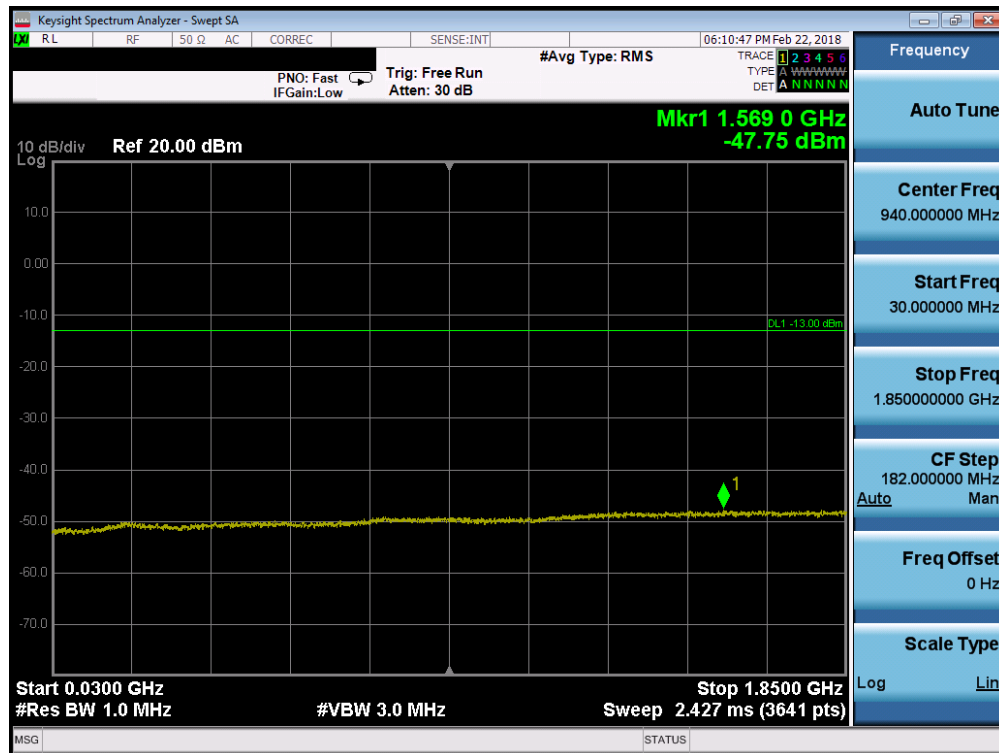
Plot 7-74. Conducted Spurious Plot (Band 25/2 - 1.4MHz QPSK - RB Size 1, RB Offset 0 - High Channel)
