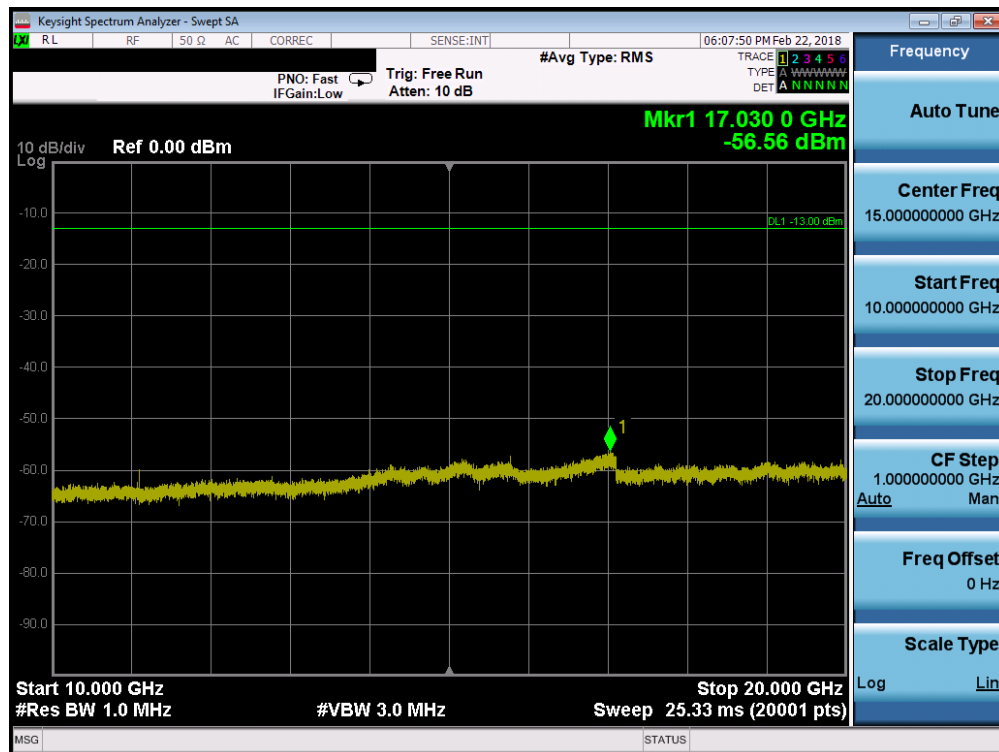
Plot 7-70. Conducted Spurious Plot (Band 25/2 - 1.4MHz QPSK - RB Size 1, RB Offset 0 - Low Channel)
