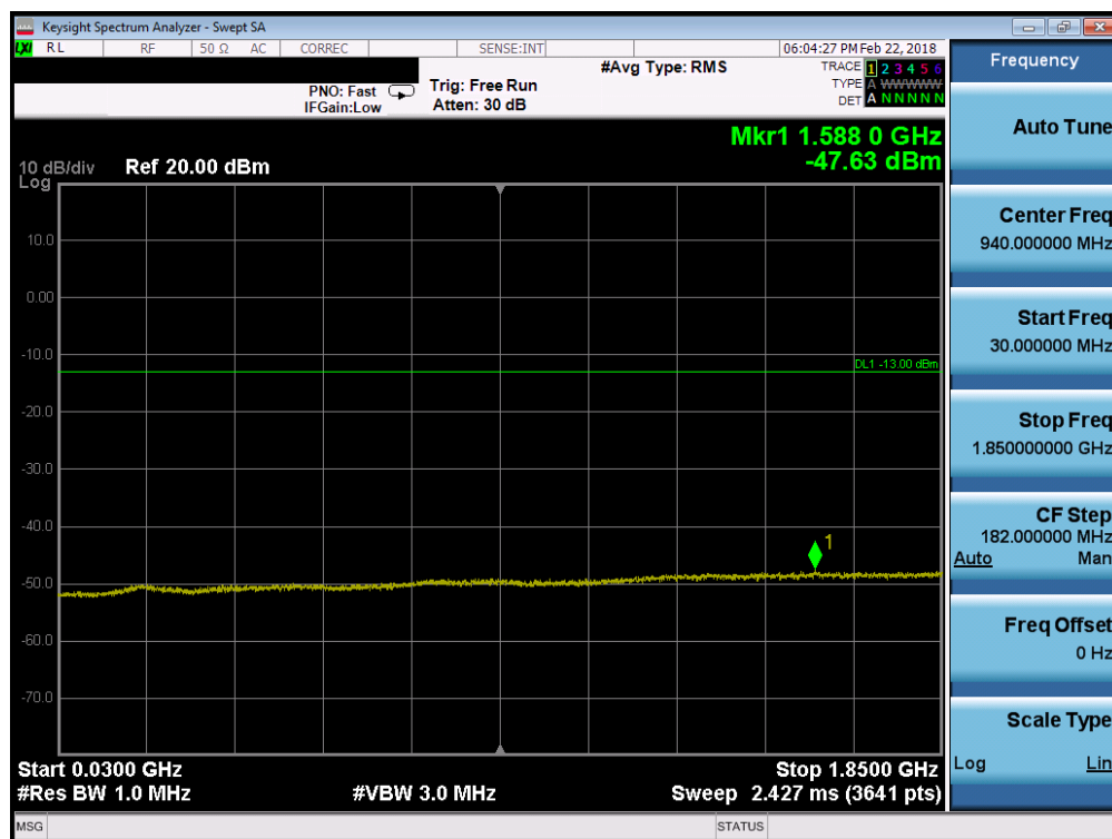
Plot 7-71. Conducted Spurious Plot (Band 25/2 - 1.4MHz QPSK - RB Size 1, RB Offset 0 - Mid Channel)
