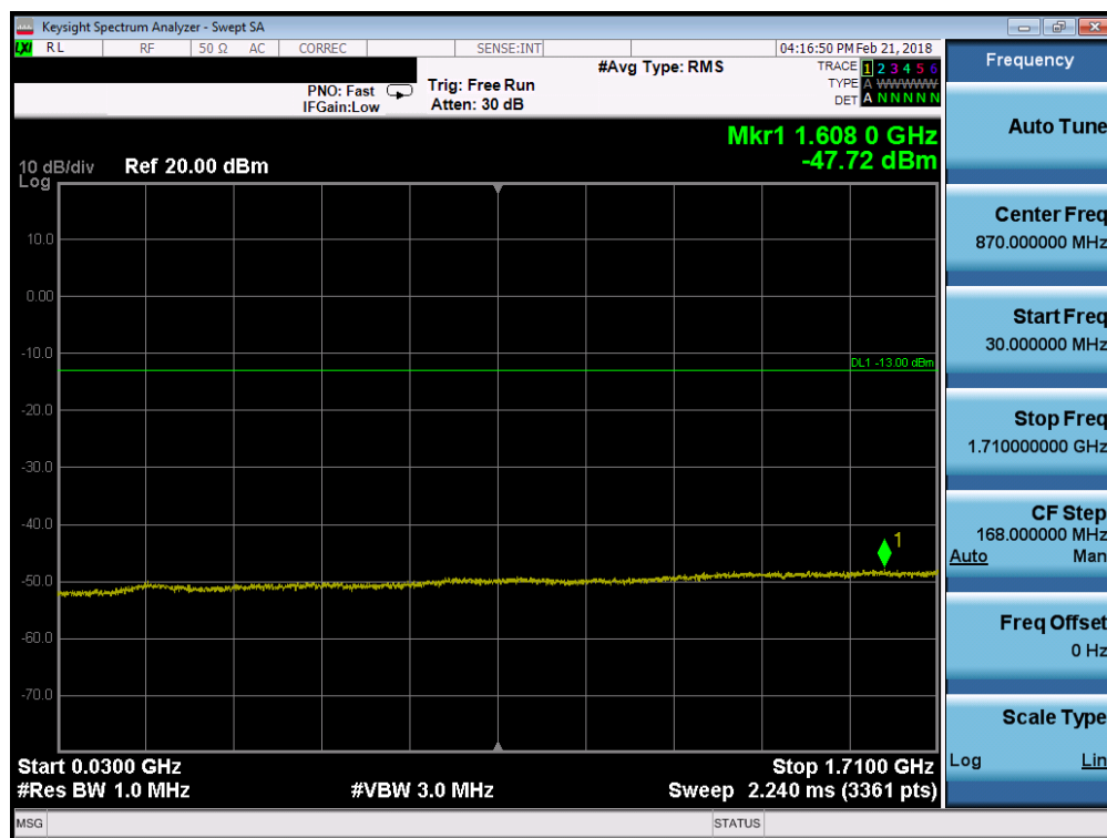
Plot 7-62. Conducted Spurious Plot (Band 4 - 1.4MHz QPSK - RB Size 1, RB Offset 0 - Mid Channel)
