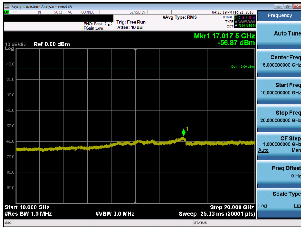
Plot 7-61. Conducted Spurious Plot (Band 4 - 1.4MHz QPSK - RB Size 1, RB Offset 0 - Low Channel)
