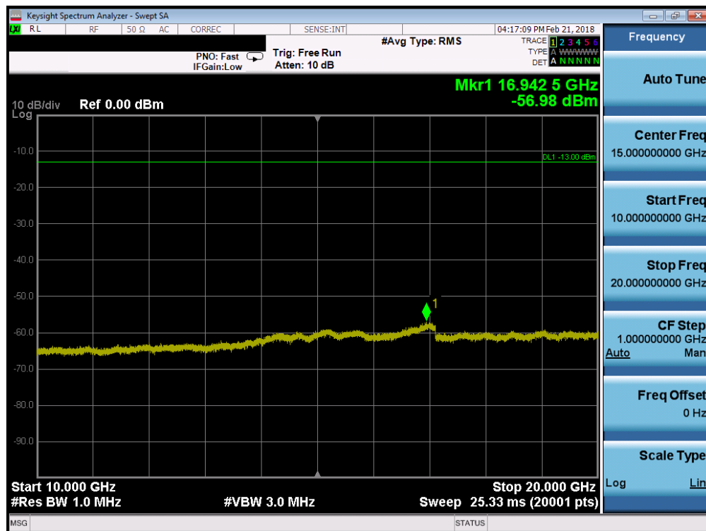
Plot 7-64. Conducted Spurious Plot (Band 4 - 1.4MHz QPSK - RB Size 1, RB Offset 0 - Mid Channel)
