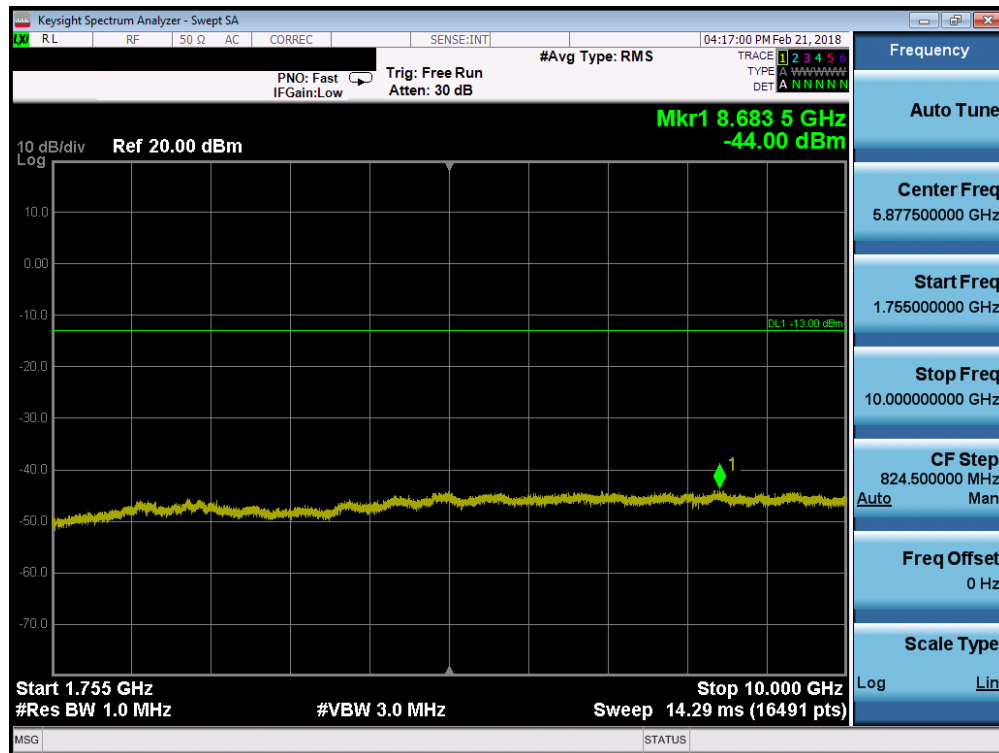
Plot 7-63. Conducted Spurious Plot (Band 4 - 1.4MHz QPSK - RB Size 1, RB Offset 0 - Mid Channel)
