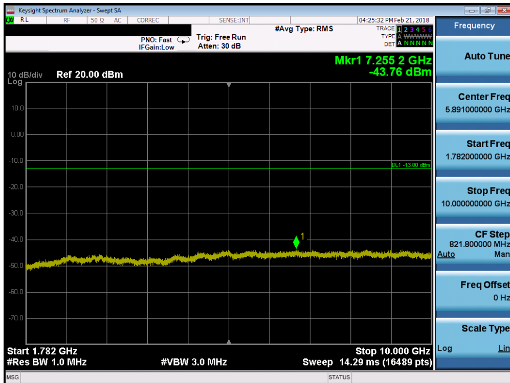
Plot 7-66. Conducted Spurious Plot (Band 4 - 1.4MHz QPSK - RB Size 1, RB Offset 0 - High Channel)
