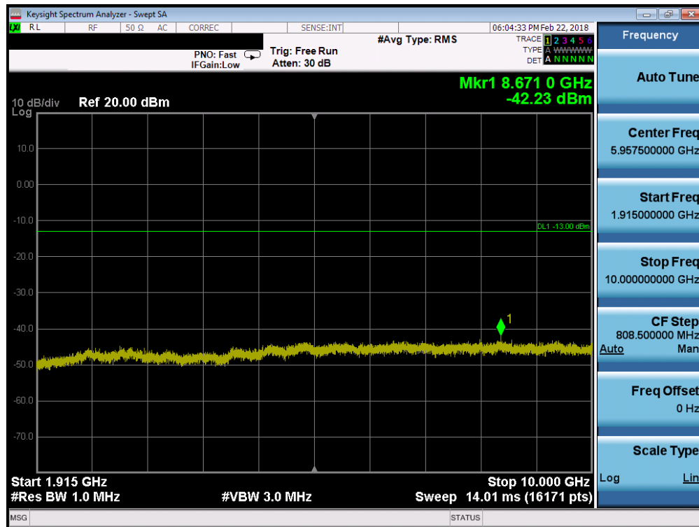
Plot 7-72. Conducted Spurious Plot (Band 25/2 - 1.4MHz QPSK - RB Size 1, RB Offset 0 - Mid Channel)
