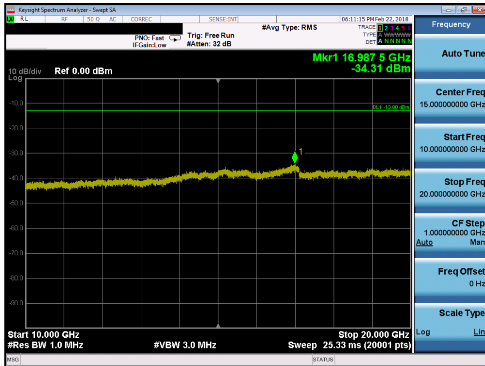
Plot 7-76. Conducted Spurious Plot (Band 25/2 - 1.4MHz QPSK - RB Size 1, RB Offset 0 - High Channel)
