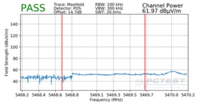
Plot 7-91. Radiated Lower Band Edge Plot (Peak – UNII Band 2C)
