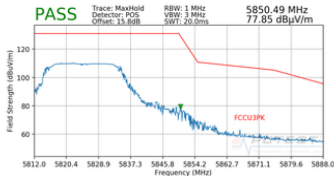
Plot 7-92. Radiated Upper Band Edge Plot (Peak – UNII Band 3)
