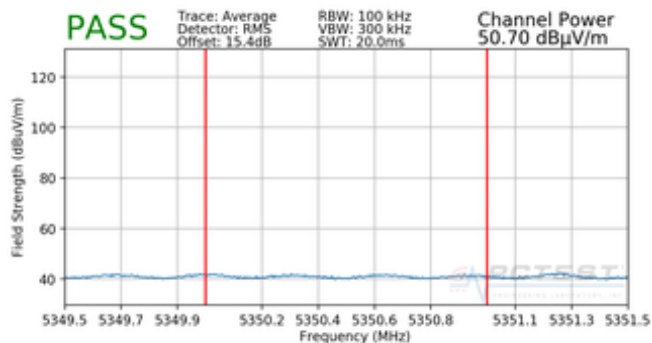
Plot 7-95. Radiated Upper Band Edge Plot (Average – UNII Band 2A)
