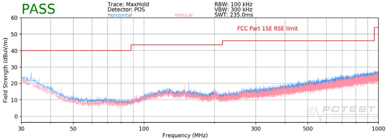
Plot 7-107. Radiated Spurious Plot below 1GHz (802.11a – U3 Ch. 157)
