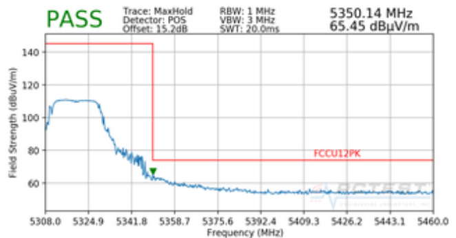
Plot 7-89. Radiated Upper Band Edge Plot (Peak – UNII Band 2A)
