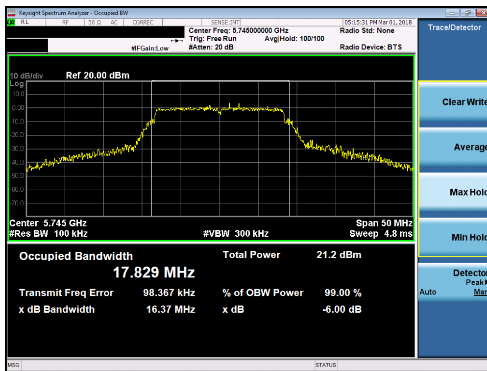
Plot 7-31. 6dB Bandwidth Plot (802.11a (UNII Band 3) – Ch. 149)
