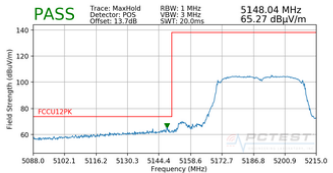
Plot 7-94. Radiated Lower Band Edge Plot (Peak – UNII Band 1)
