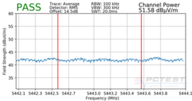
Plot 7-104. Radiated Lower Band Edge Plot (Average – UNII Band 2C)
