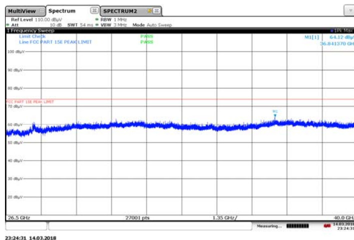
Plot 7-85. Radiated Spurious Plot 26.5GHz - 40GHz (802.11a V Polarization)
