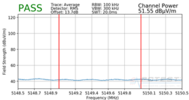
Plot 7-86. Radiated Lower Band Edge Plot (Average – UNII Band 1)
