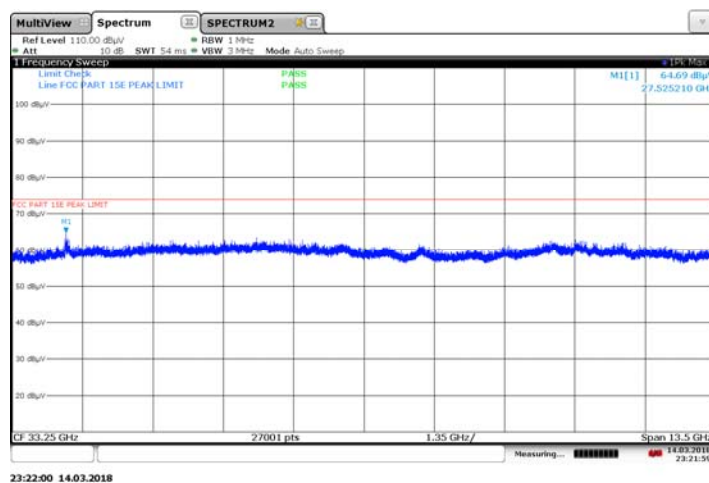
Plot 7-84. Radiated Spurious Plot 26.5GHz - 40GHz (802.11a H Polarization)
