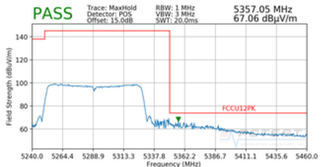
Plot 7-103. Radiated Upper Band Edge Plot (Peak – UNII Band 2A)
