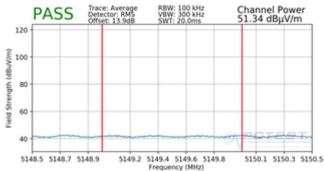
Plot 7-93. Radiated Lower Band Edge Plot (Average – UNII Band 1)
