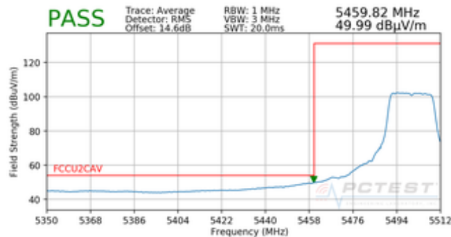
Plot 7-90. Radiated Lower Band Edge Plot (Average – UNII Band 2C)
