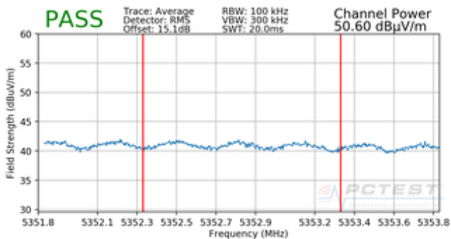
Plot 7-88. Radiated Upper Band Edge Plot (Average – UNII Band 2A)
