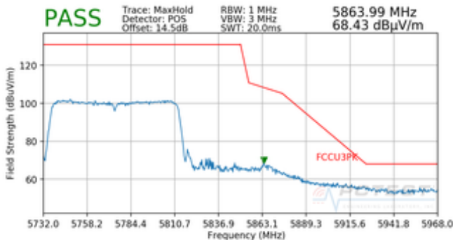
Plot 7-106. Radiated Upper Band Edge Plot (Peak – UNII Band 3)
