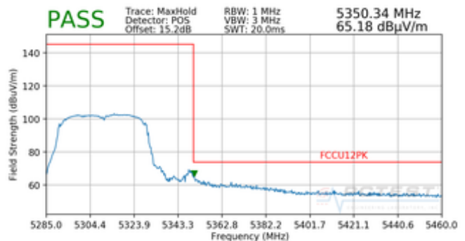
Plot 7-96. Radiated Upper Band Edge Plot (Peak – UNII Band 2A)
