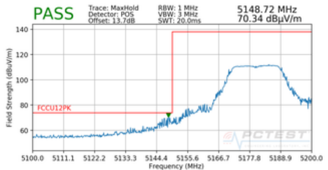
Plot 7-87. Radiated Lower Band Edge Plot (Peak – UNII Band 1)
