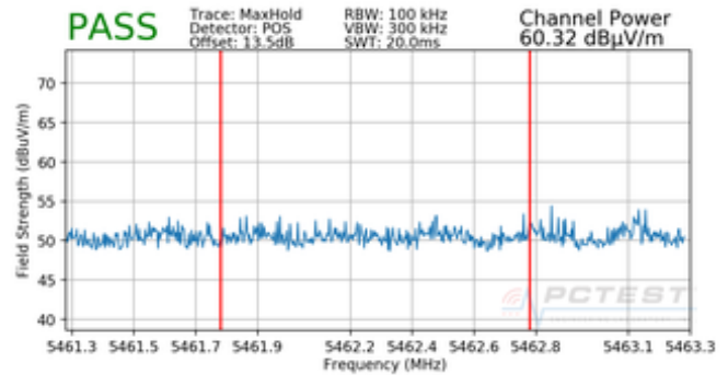
Plot 7-105. Radiated Lower Band Edge Plot (Peak – UNII Band 2C)
