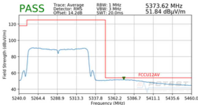
Plot 7-102. Radiated Upper Band Edge Plot (Average – UNII Band 2A)
