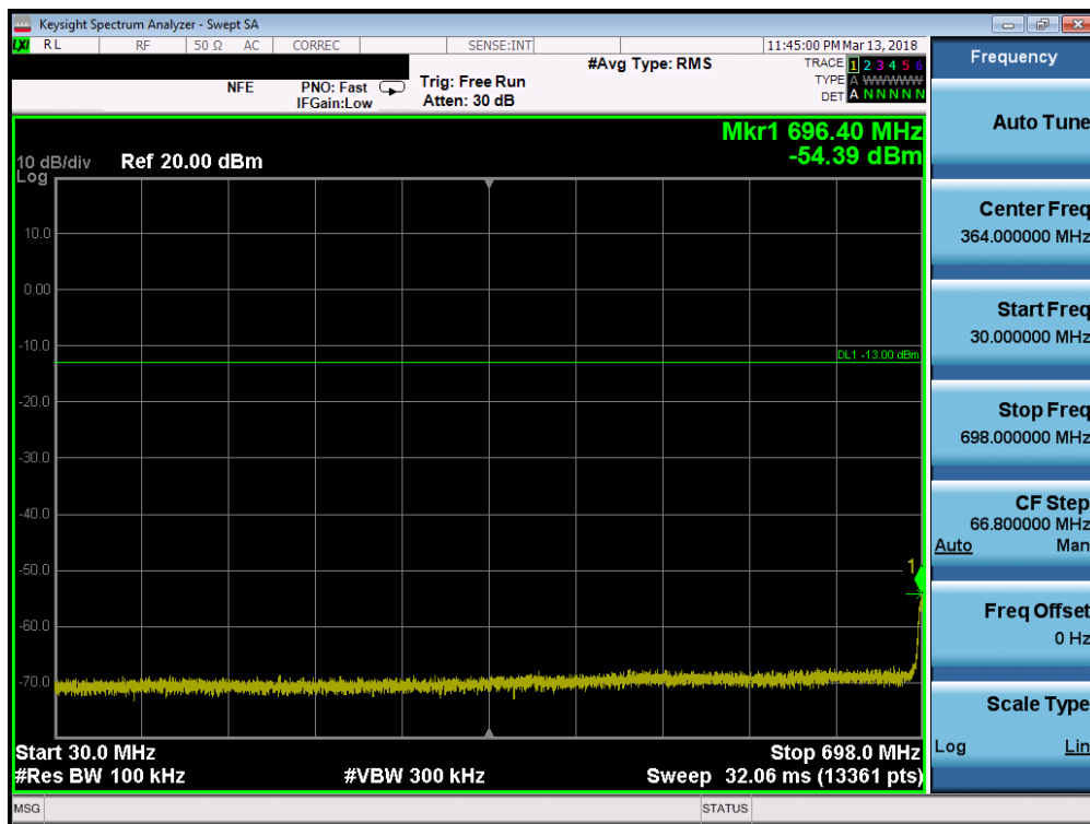
Plot 7-69. Conducted Spurious Plot (Band 12 - 3.0MHz QPSK - RB Size 1, RB Offset 0 - Mid Channel)
