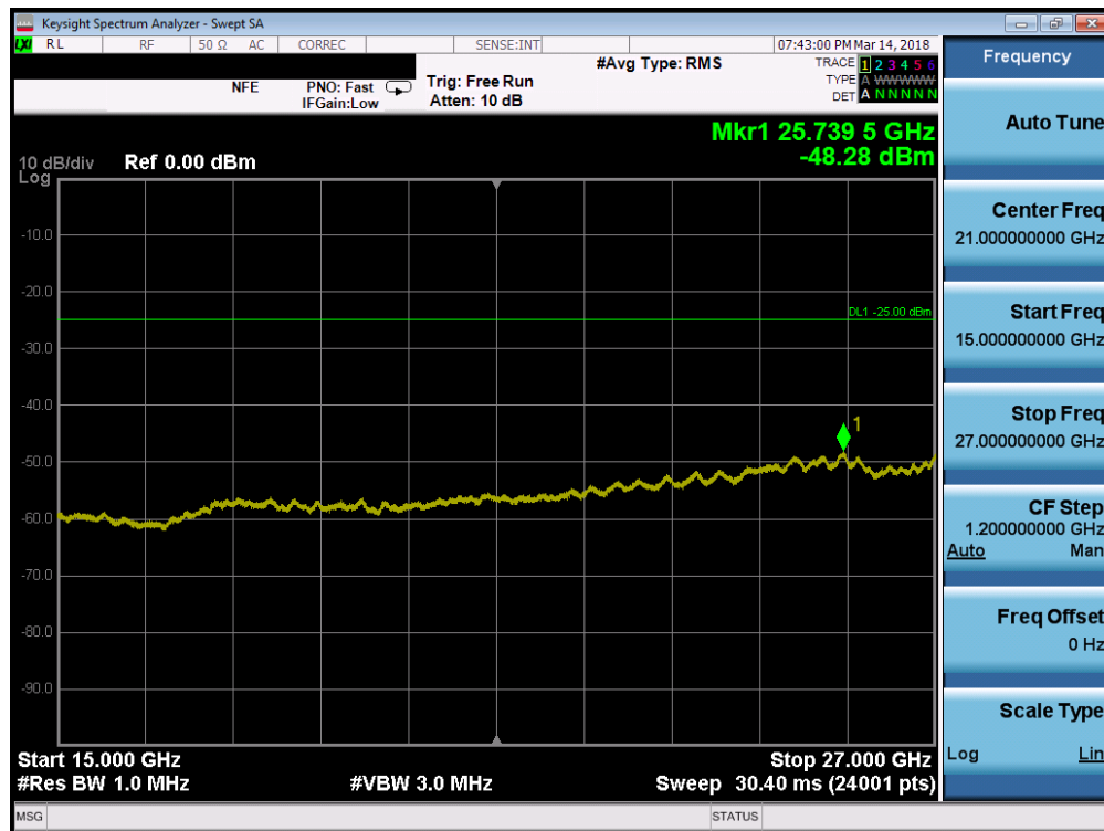
Plot 7-104. Conducted Spurious Plot (Band 7 - 10.0MHz QPSK - RB Size 1, RB Offset 0 - Low Channel)
