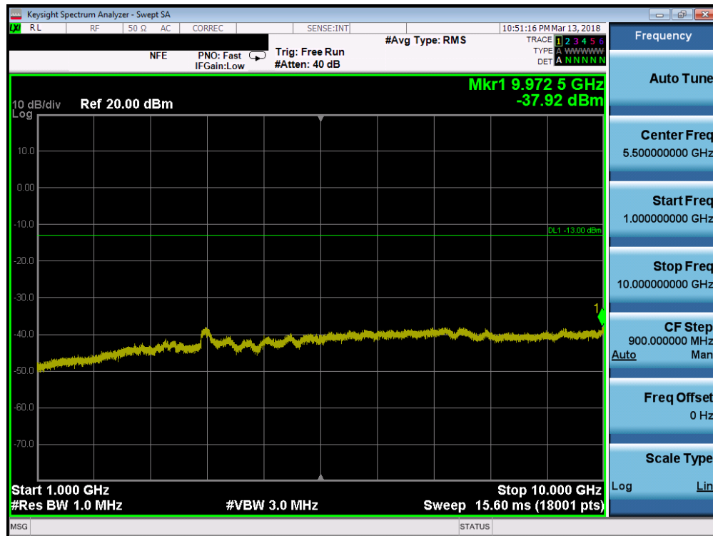
Plot 7-83. Conducted Spurious Plot (Band 5 - 3.0MHz QPSK - RB Size 1, RB Offset 0 - High Channel)
