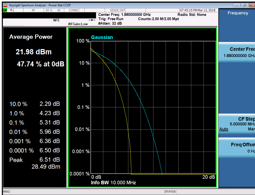
Plot 7-211. PAR Plot (Band 2 - 10.0MHz QPSK - Full RB Configuration)
