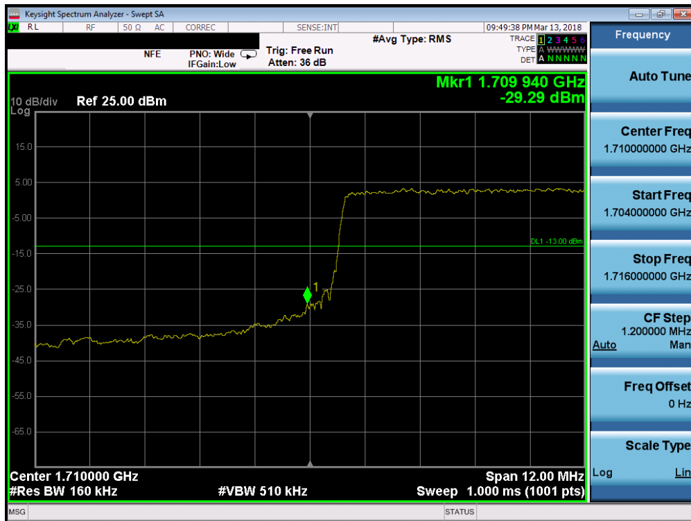
Plot 7-161. Lower Band Edge Plot (Band 66/4 - 15.0MHz QPSK - Full RB Configuration)
