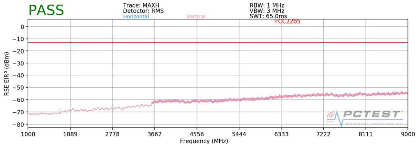
Plot 7-77. Radiated Spurious Plot above 1GHz (Cell WCDMA)
