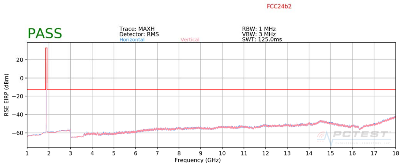
Plot 7-80. Radiated Spurious Plot above 1GHz (PCS WCDMA)
