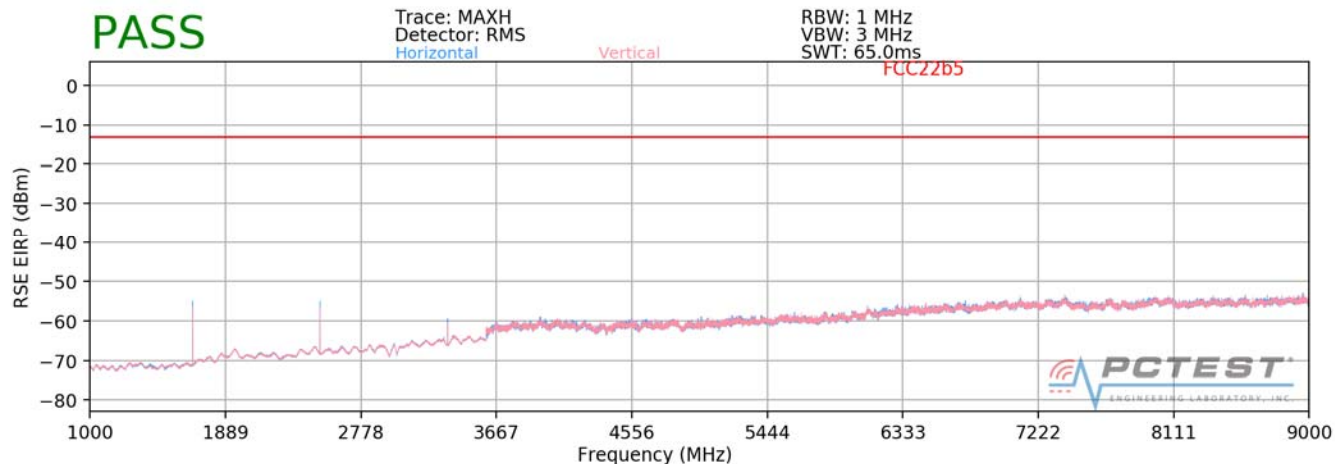
Plot 7-76. Radiated Spurious Plot above 1GHz (Cell GPRS)
