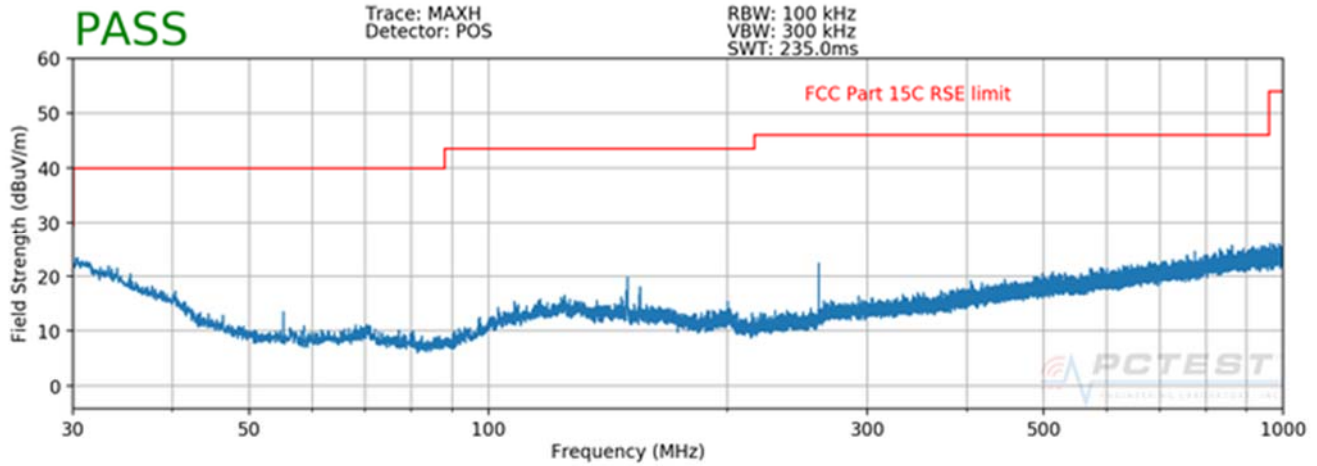
Plot 7-49. Radiated Spurious Plot below 1GHz (Pol. H)
