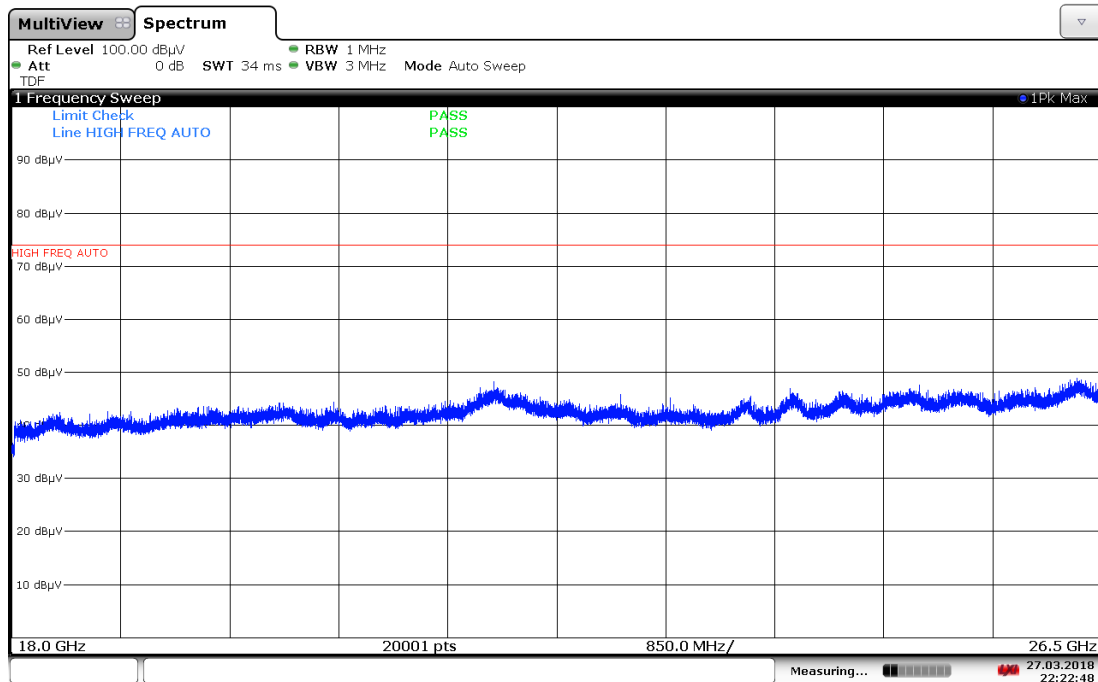
Plot 7-84. Radiated Spurious Plot 18GHz - 26.5GHz (802.11a) – Vertical
