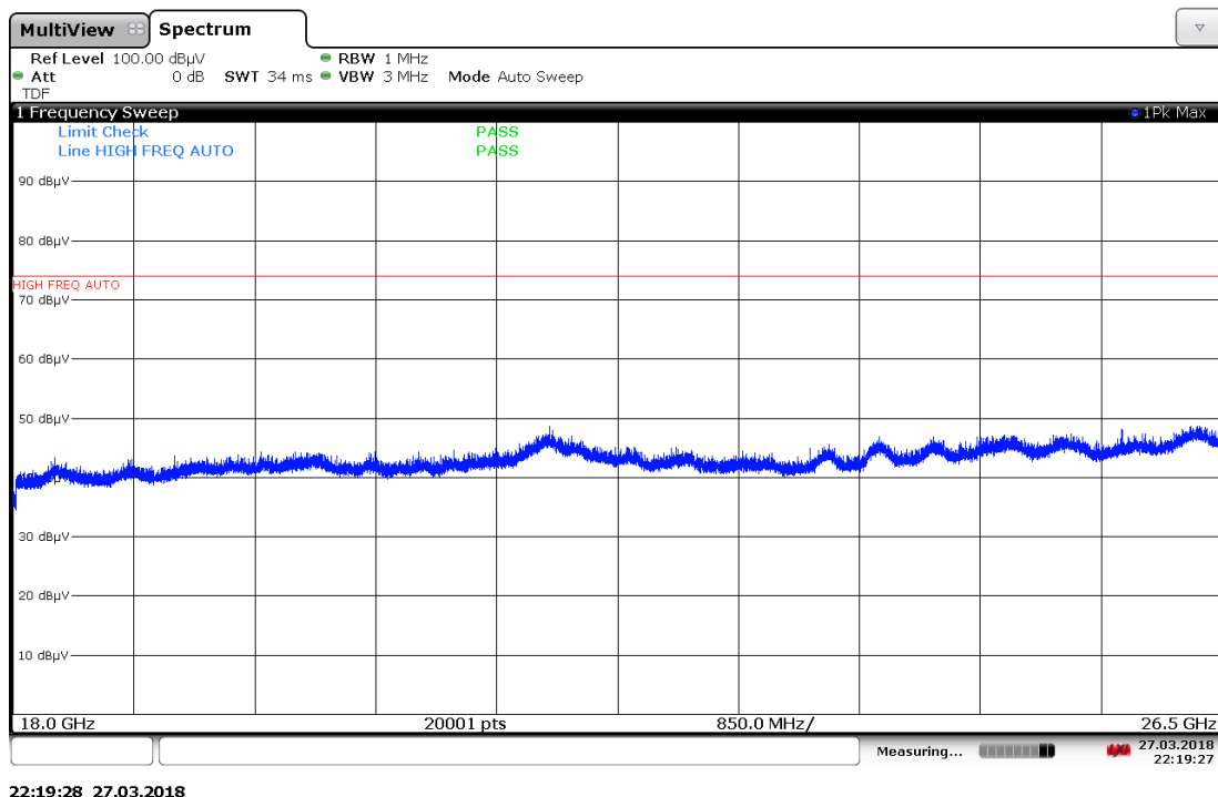
Plot 7-35. Radiated Spurious Plot above 18GHz – Vertical
