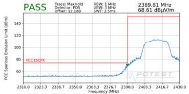
Plot 7-37. Radiated Restricted Lower Band Edge Measurement (Peak)
