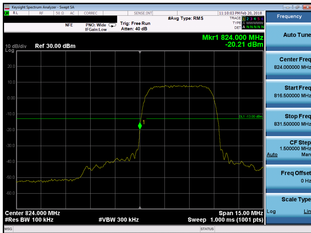
Plot 7-77. Band Edge Plot (Cellular WCDMA Mode - Low Channel)
