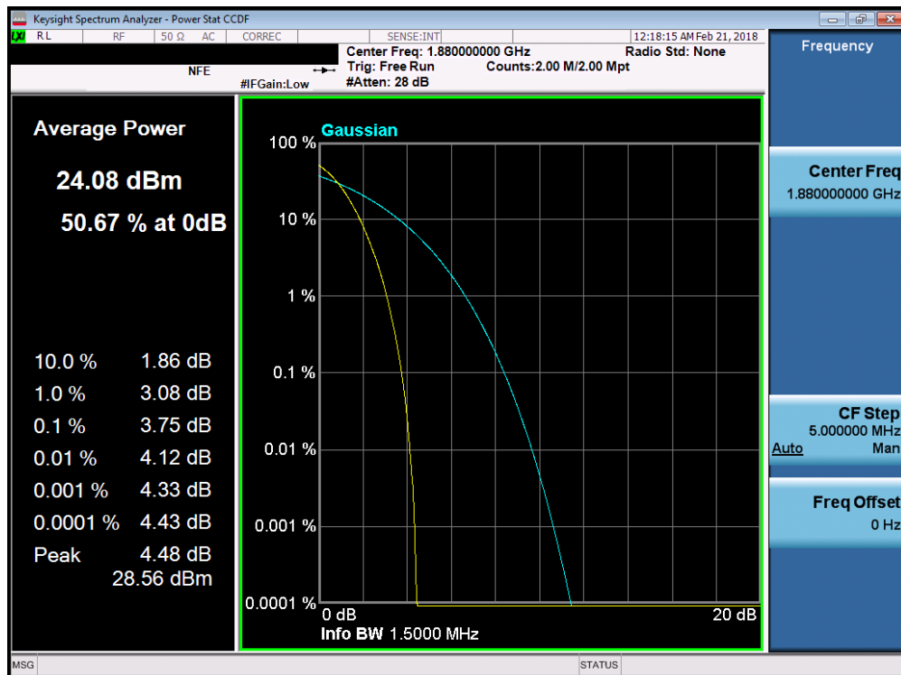
Plot 7-88. Peak-Average Ratio Plot (PCS CDMA Mode)
