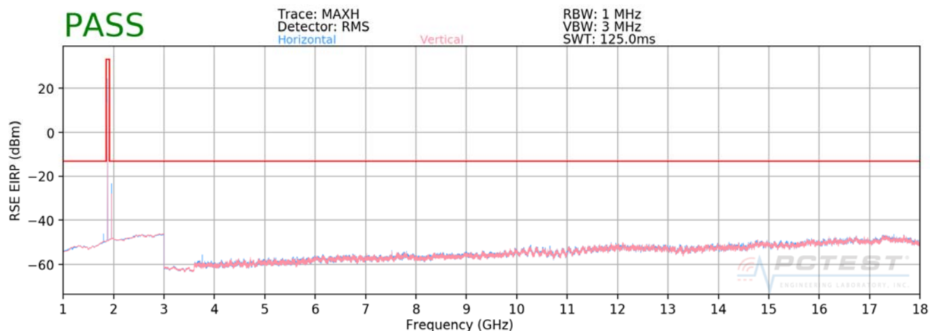
Plot 7-95. Radiated Spurious Plot Above 1GHz (PCS CDMA Mode)
