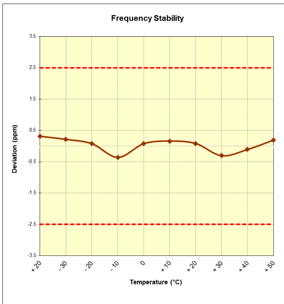
Figure 7-9. Frequency Stability Graph (Cellular CDMA Mode – Ch. 384)
