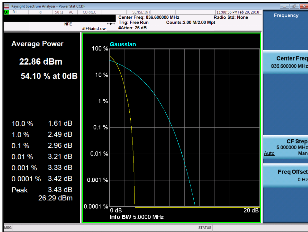
Plot 7-89. Peak-Average Ratio Plot (Cellular WCDMA Mode)
