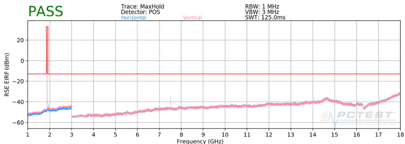
Plot 7-94. Radiated Spurious Plot Above 1GHz (PCS GPRS Mode)
