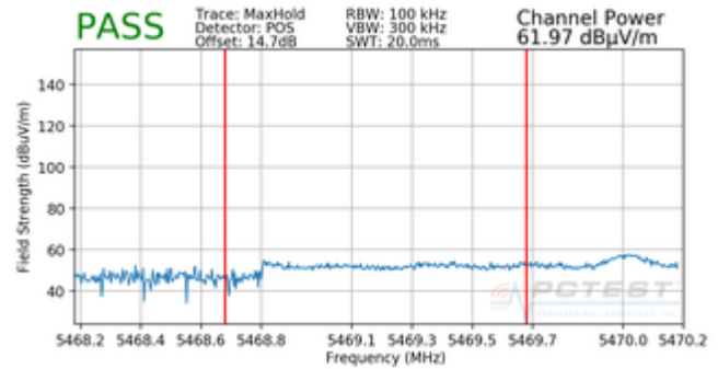
Plot 7-90. Radiated Lower Band Edge Plot (Peak – UNII Band 2C)
