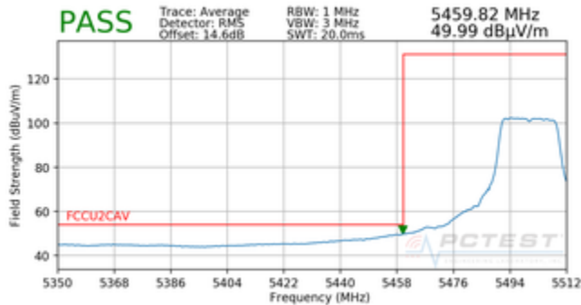
Plot 7-89. Radiated Lower Band Edge Plot (Average – UNII Band 2C)
