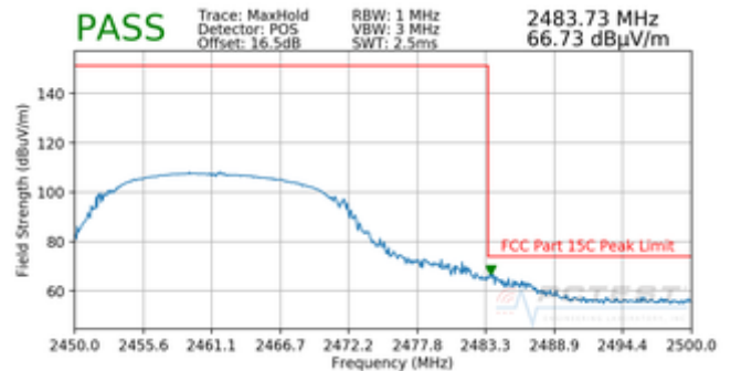
Plot 7-42. Radiated Restricted Upper Band Edge Measurement (Peak)
