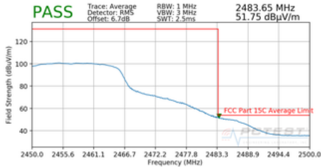
Plot 7-39. Radiated Restricted Upper Band Edge Measurement (Average)
