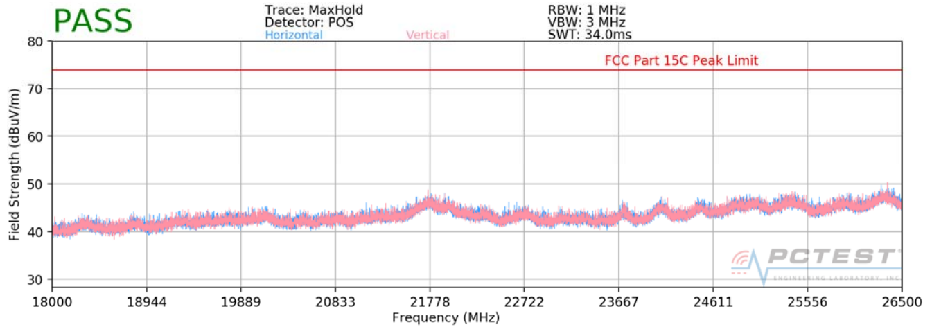
Plot 7-34. Radiated Spurious Plot above 18GHz
