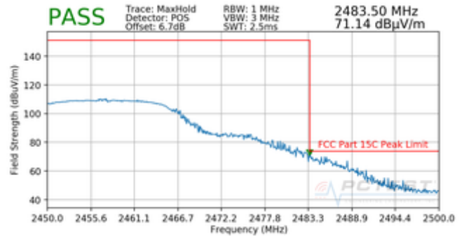
Plot 7-40. Radiated Restricted Upper Band Edge Measurement (Peak)
