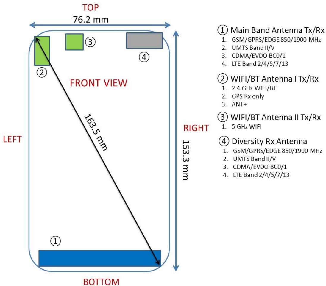
Figure F-1 DUT Antenna Locations
