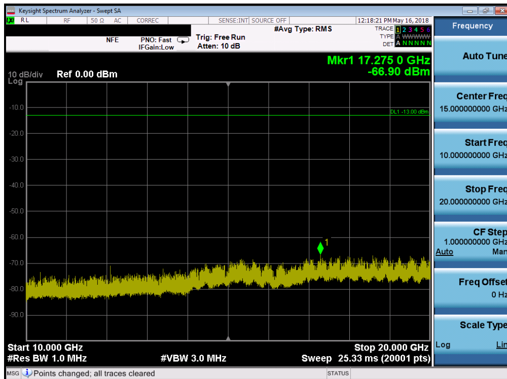
Plot 7-79. Conducted Spurious Plot (Band 66/4 - 10.0MHz QPSK - RB Size 1, RB Offset 0 - Mid Channel)
