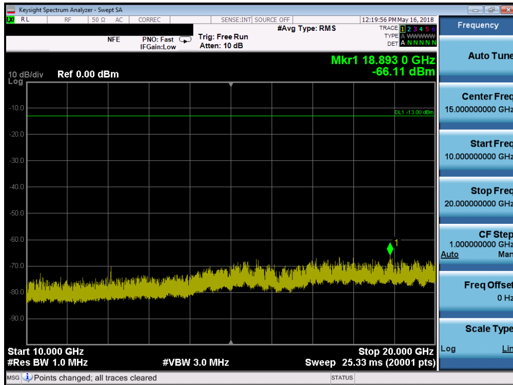
Plot 7-76. Conducted Spurious Plot (Band 66/4 - 10.0MHz QPSK - RB Size 1, RB Offset 0 - Low Channel)
