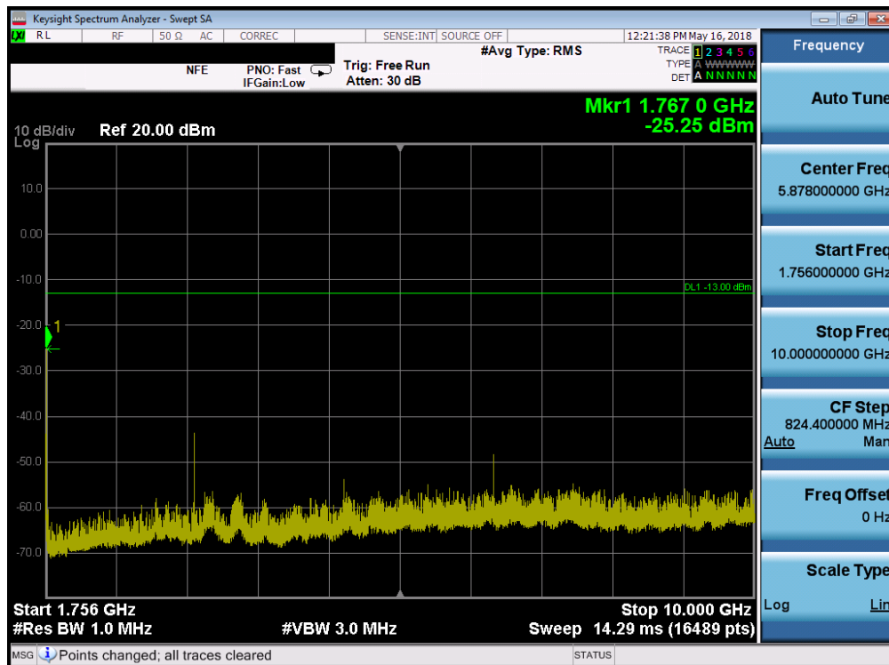
Plot 7-81. Conducted Spurious Plot (Band 66/4 - 10.0MHz QPSK - RB Size 1, RB Offset 0 - High Channel)
