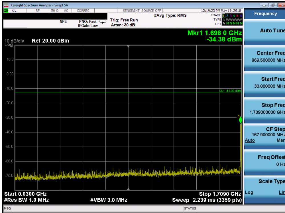
Plot 7-74. Conducted Spurious Plot (Band 66/4 - 10.0MHz QPSK - RB Size 1, RB Offset 0 - Low Channel)
