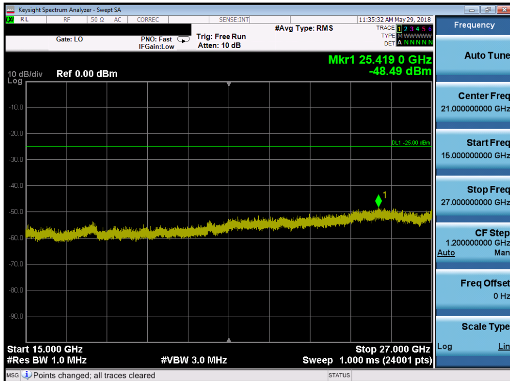
Plot 7-97. Conducted Spurious Plot (Band 41 - 20.0MHz QPSK - RB Size 1, RB Offset 0 - Mid Channel)
