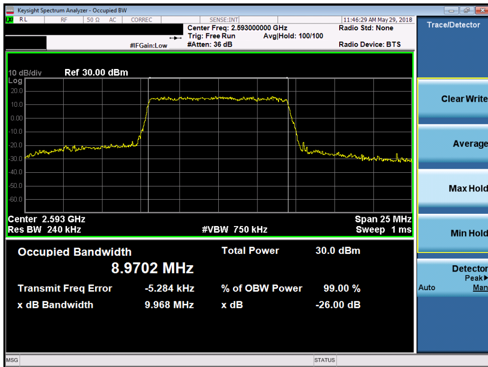
Plot 7-48. Occupied Bandwidth Plot (Band 41 - 10.0MHz 16-QAM - Full RB Configuration)
