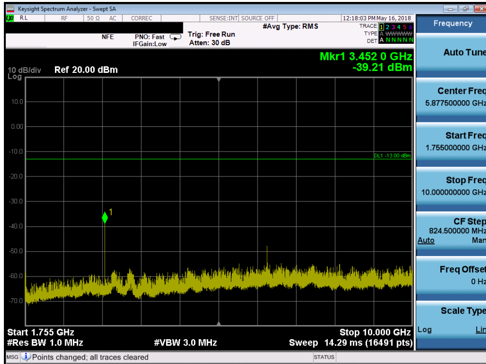
Plot 7-78. Conducted Spurious Plot (Band 66/4 - 10.0MHz QPSK - RB Size 1, RB Offset 0 - Mid Channel)
