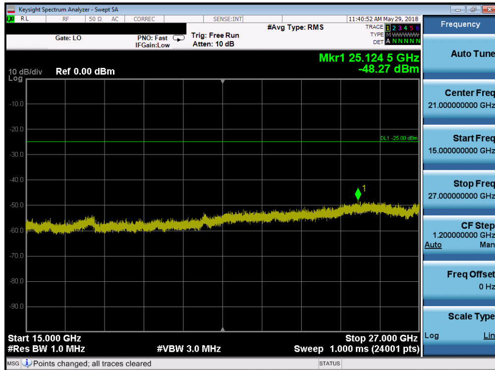
Plot 7-100. Conducted Spurious Plot (Band 41 - 20.0MHz QPSK - RB Size 1, RB Offset 0 - High Channel)
