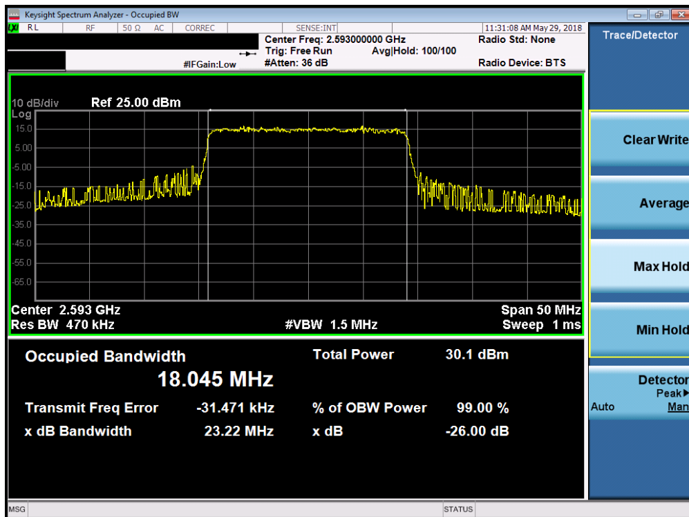
Plot 7-52. Occupied Bandwidth Plot (Band 41 - 20.0MHz 16-QAM - Full RB Configuration)
