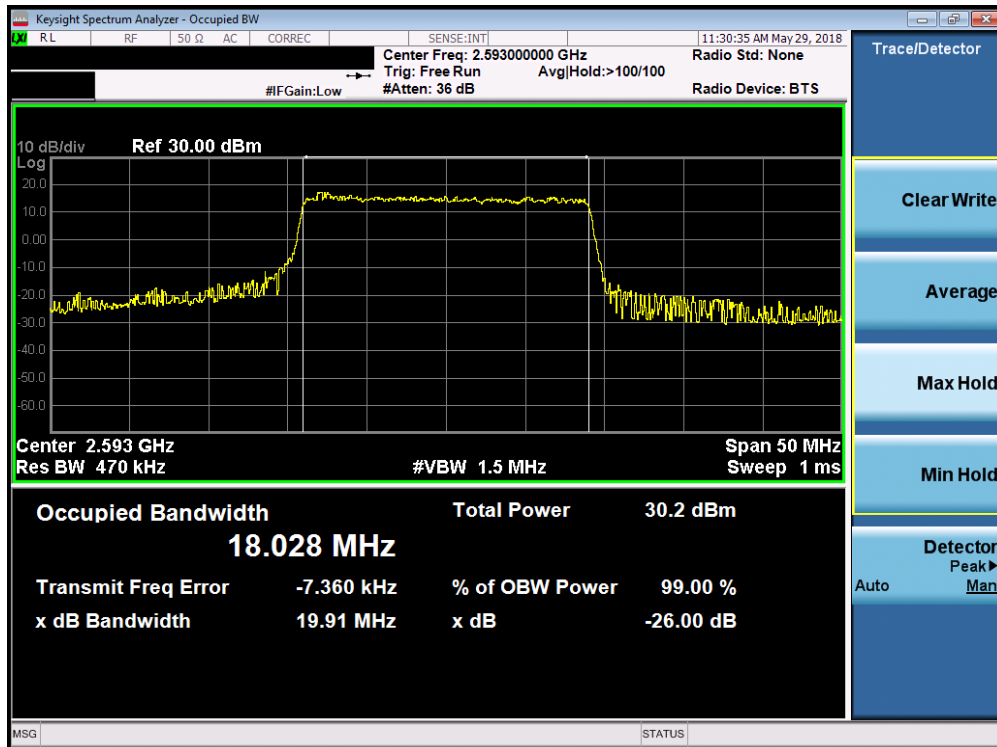
Plot 7-51. Occupied Bandwidth Plot (Band 41 - 20.0MHz QPSK - Full RB Configuration)
