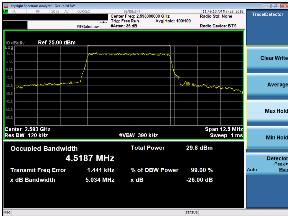
Plot 7-46. Occupied Bandwidth Plot (Band 41 - 5.0MHz 16-QAM - Full RB Configuration)
