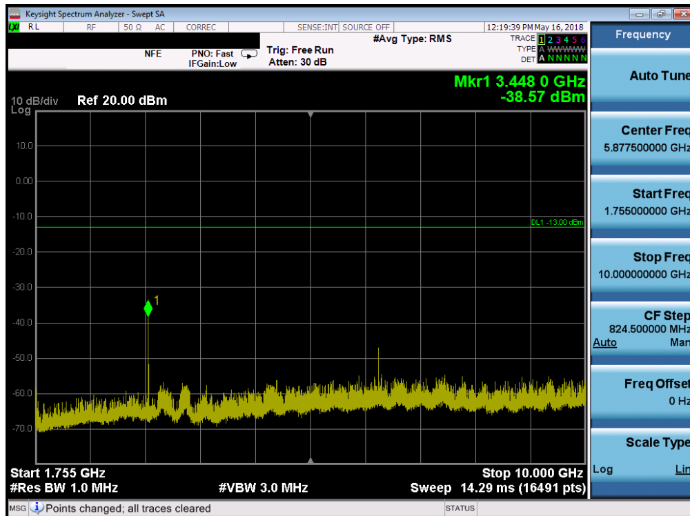
Plot 7-75. Conducted Spurious Plot (Band 66/4 - 10.0MHz QPSK - RB Size 1, RB Offset 0 - Low Channel)
