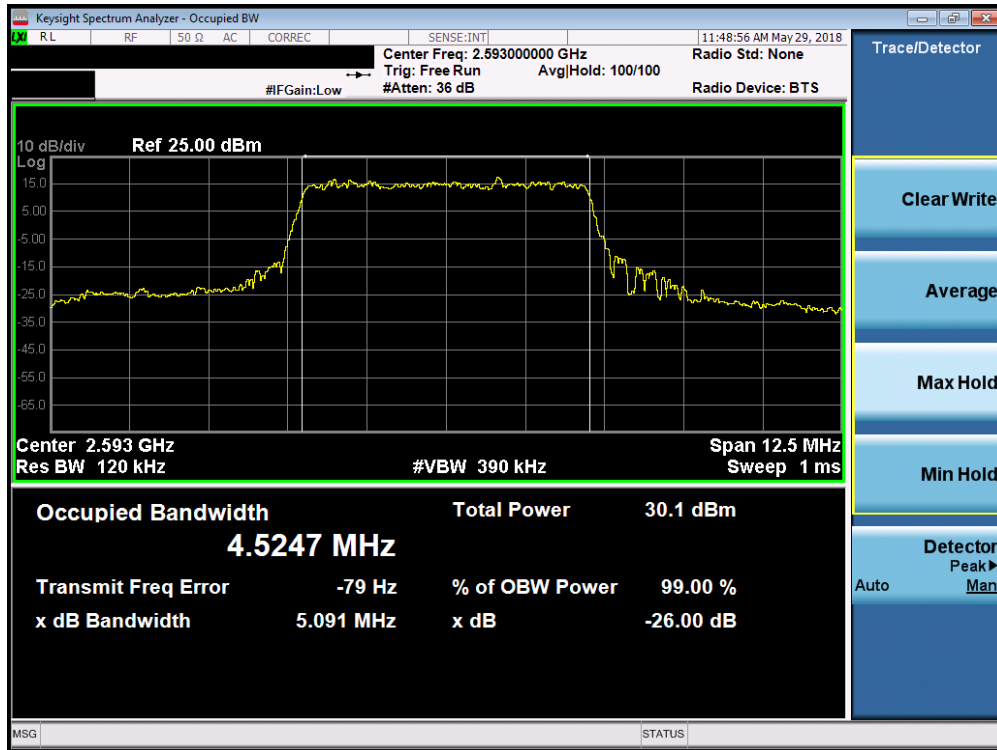
Plot 7-45. Occupied Bandwidth Plot (Band 41 - 5.0MHz QPSK - Full RB Configuration)
