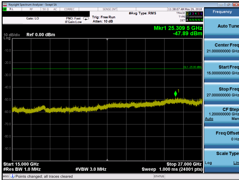
Plot 7-94. Conducted Spurious Plot (Band 41 - 20.0MHz QPSK - RB Size 1, RB Offset 0 - Low Channel)
