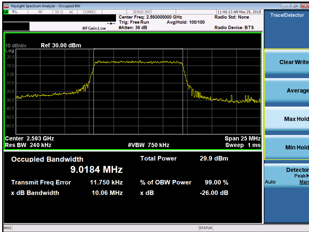
Plot 7-47. Occupied Bandwidth Plot (Band 41 - 10.0MHz QPSK - Full RB Configuration)
