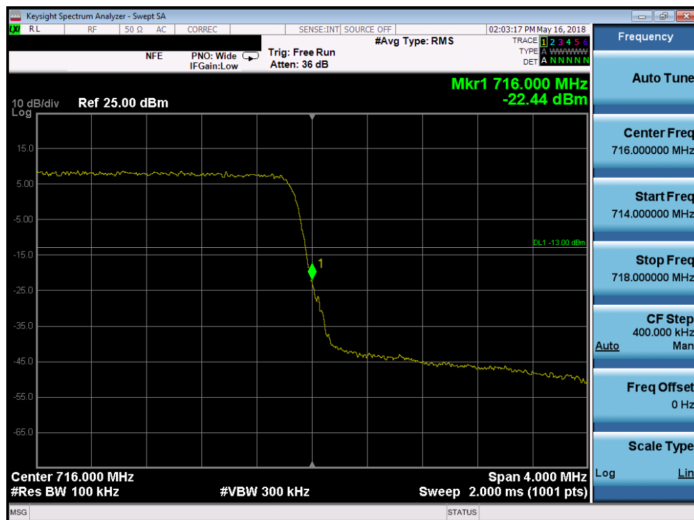
Plot 7-104. Upper Band Edge Plot (Band 12 - 3.0MHz QPSK - Full RB Configuration)
