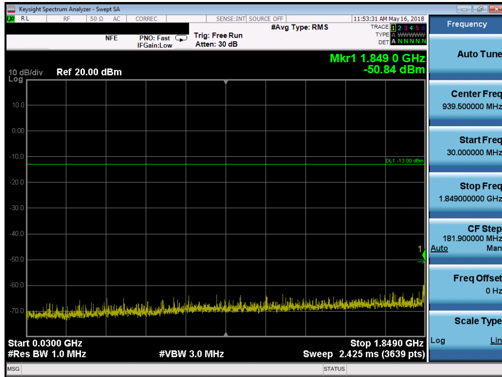
Plot 7-83. Conducted Spurious Plot (Band 2 - 10.0MHz QPSK - RB Size 1, RB Offset 0 - Low Channel)
