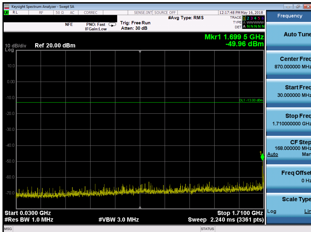
Plot 7-77. Conducted Spurious Plot (Band 66/4 - 10.0MHz QPSK - RB Size 1, RB Offset 0 - Mid Channel)
