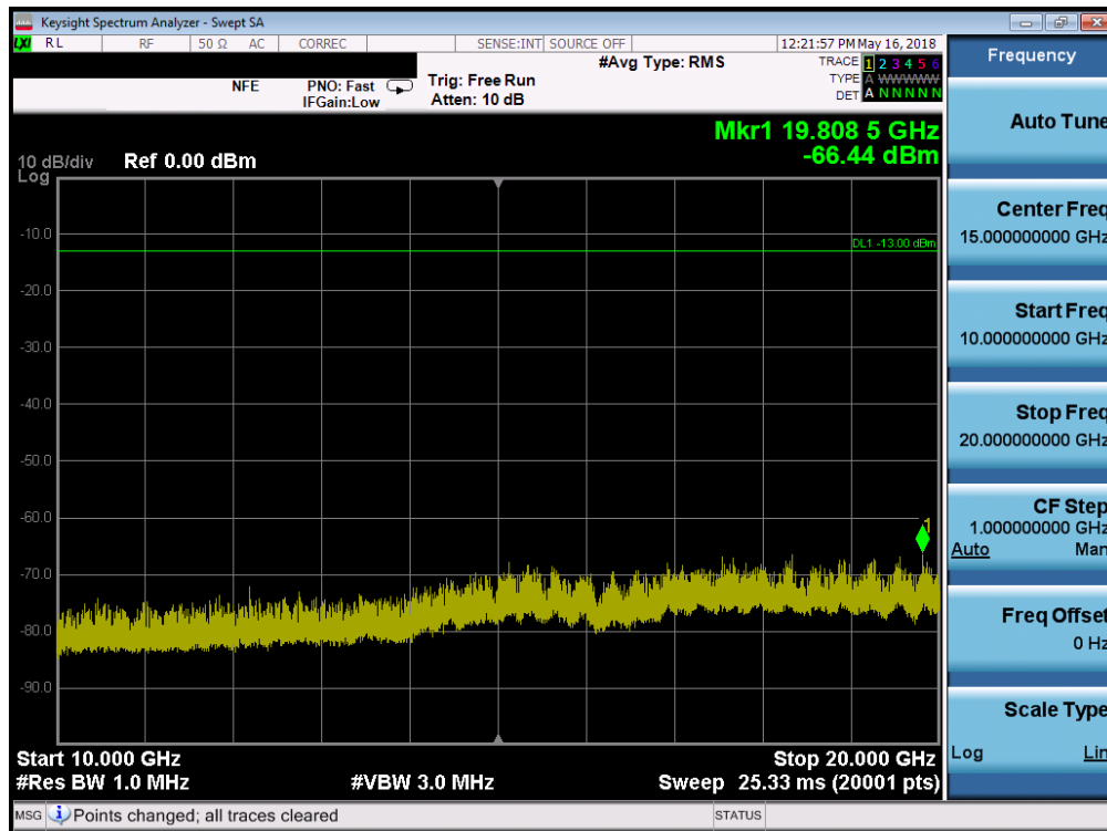
Plot 7-82. Conducted Spurious Plot (Band 66/4 - 10.0MHz QPSK - RB Size 1, RB Offset 0 - High Channel)
