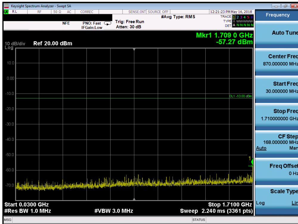
Plot 7-80. Conducted Spurious Plot (Band 66/4 - 10.0MHz QPSK - RB Size 1, RB Offset 0 - High Channel)
