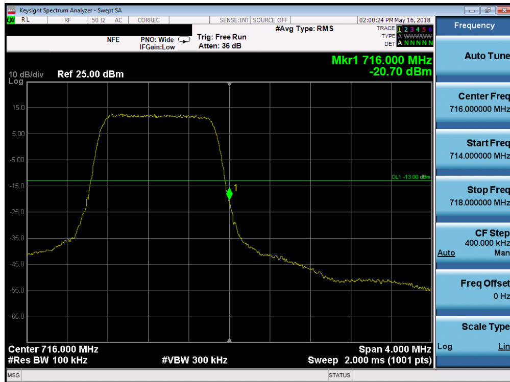
Plot 7-102. Upper Band Edge Plot (Band 12 - 1.4MHz QPSK - Full RB Configuration)
