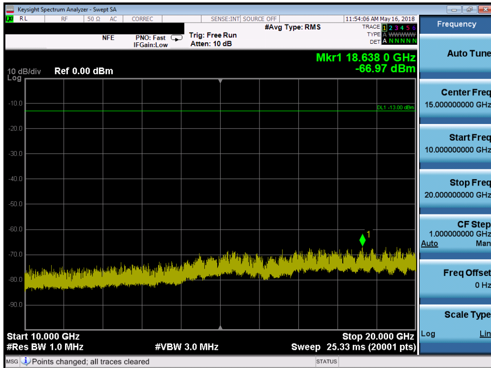
Plot 7-85. Conducted Spurious Plot (Band 2 - 10.0MHz QPSK - RB Size 1, RB Offset 0 - Low Channel)
