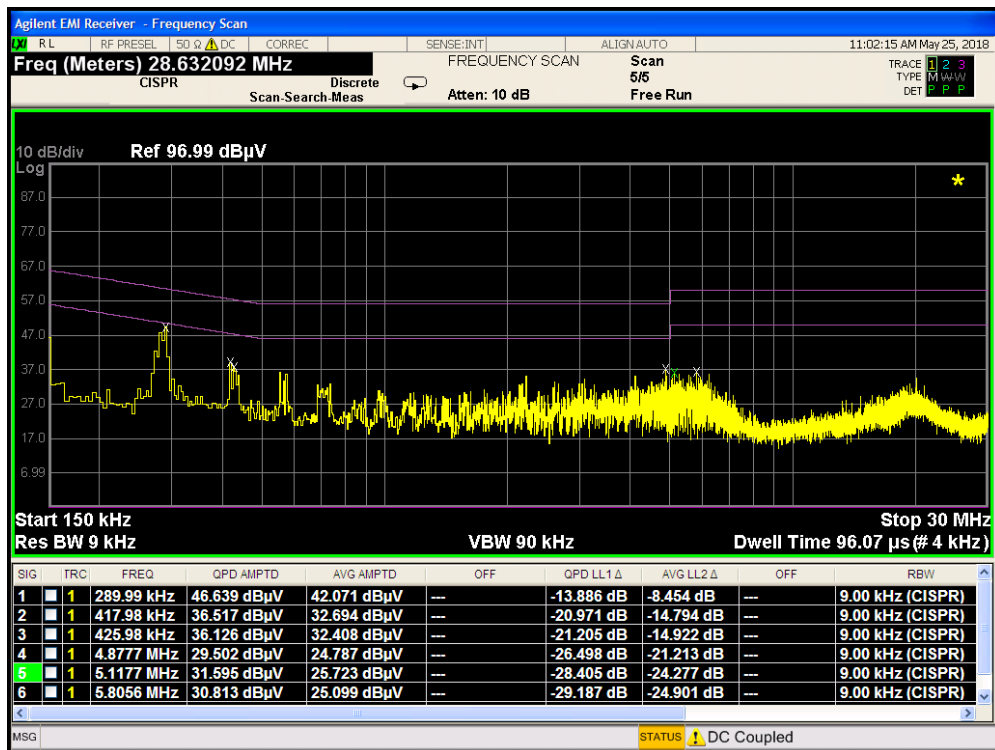
Plot 7-42. Line Conducted Plot with 802.11b (L1)
