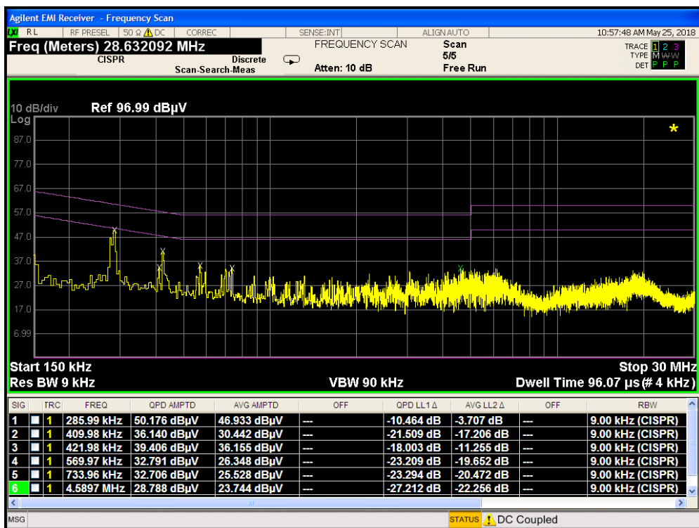
Plot 7-43. Line Conducted Plot with 802.11b (N)
