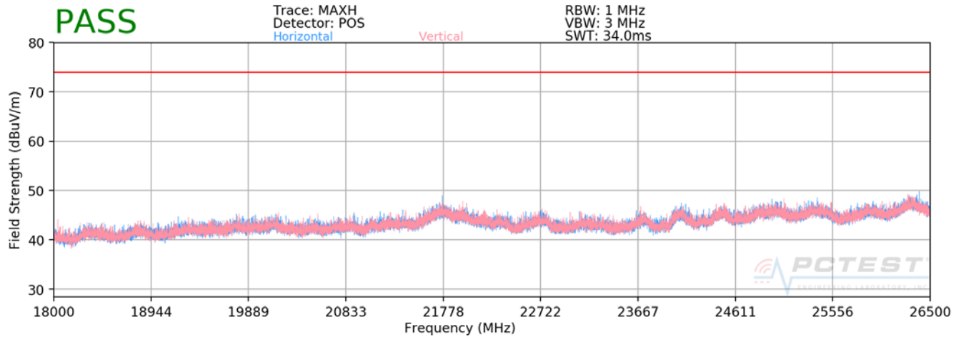
Plot 7-34. Radiated Spurious Plot above 18GHz ANT1
