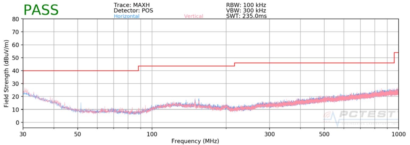
Plot 7-41. Radiated Spurious Plot below 1GHz ANT1
