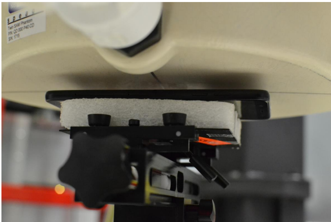
SAR Test Setup Photo 8 – Back Side at 10mm
