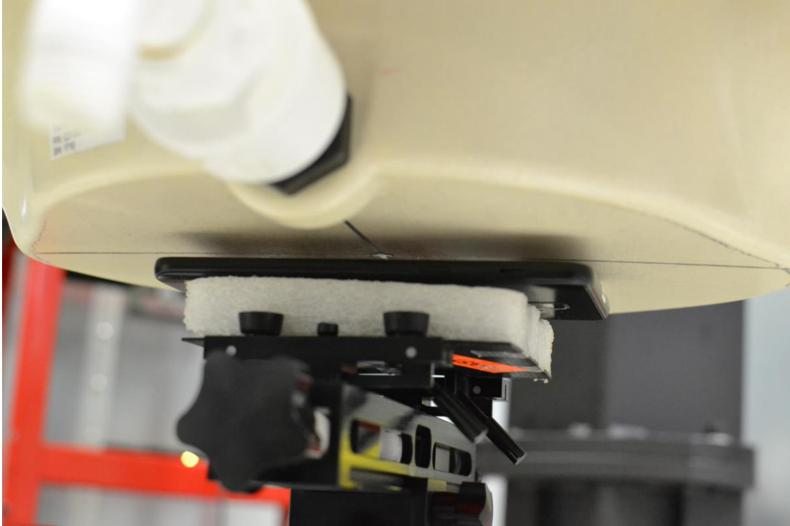
SAR Test Setup Photo 11 – Front Side at 7mm
