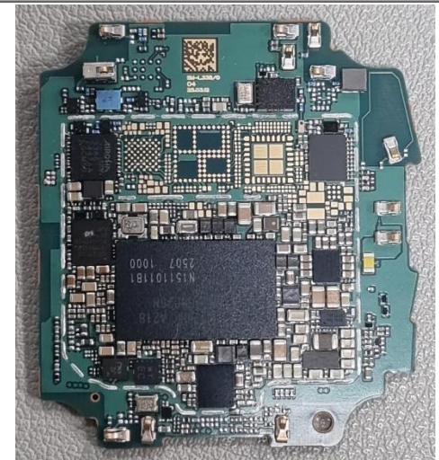
PBA Bottom(Shield can open)
