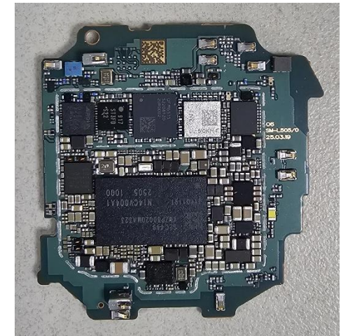
PBA Bottom(Shield can open)
