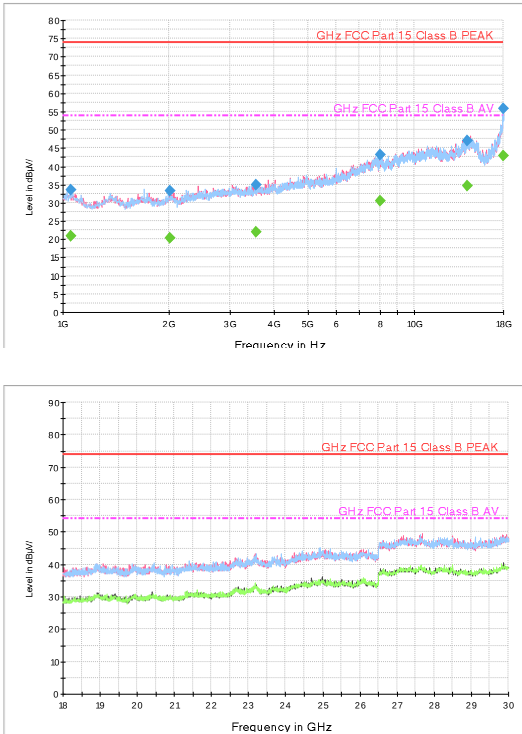
Figure 4: LTE B5 Middle ch Idle
