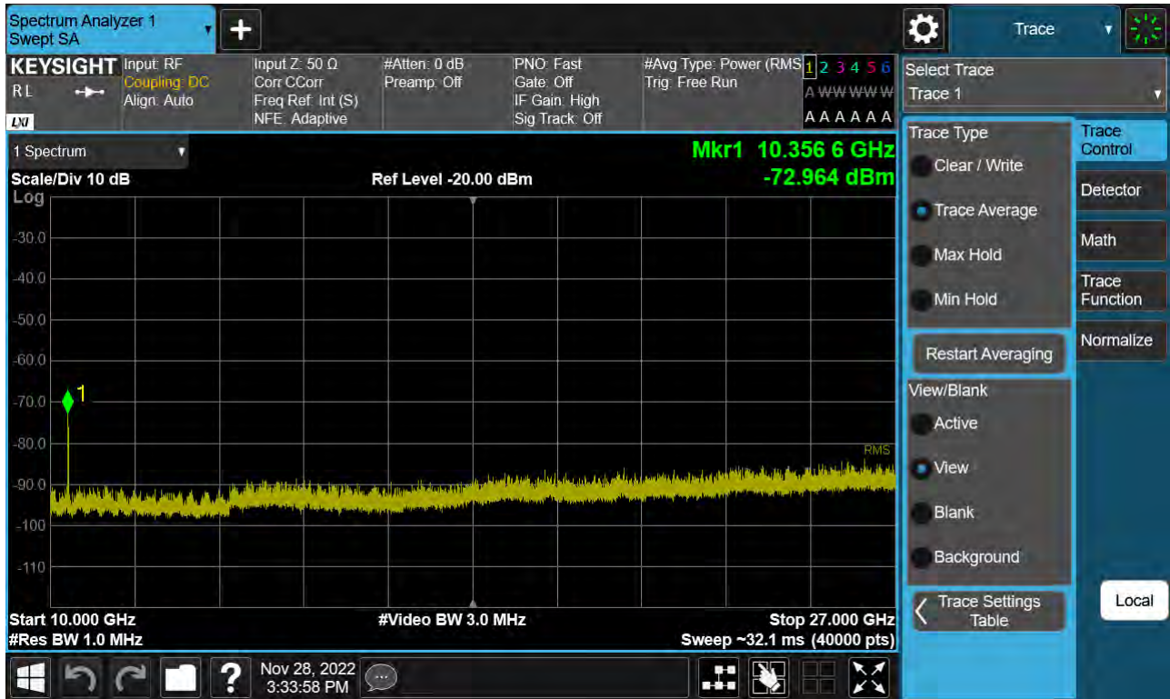
Sub6 n41. Conducted Spurious Plot 2 (10 MHz Ch. 518598 BPSK RB 1)
