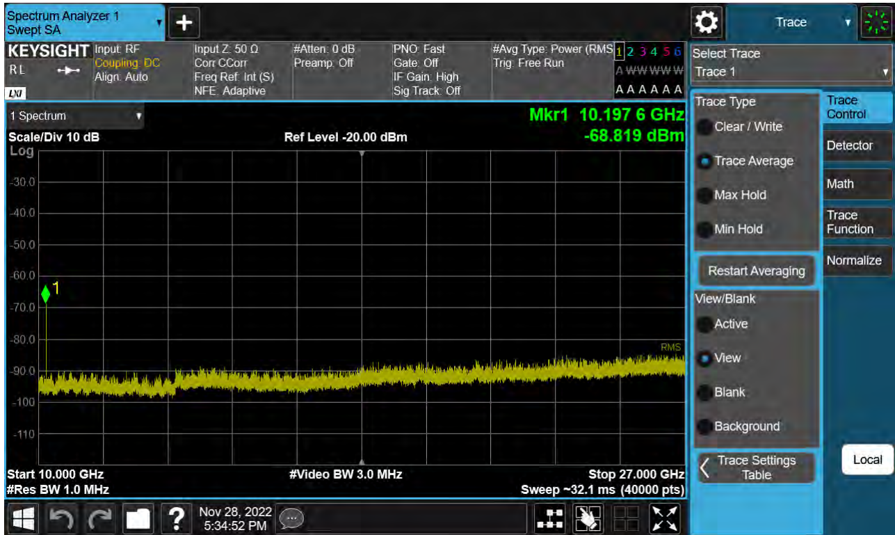
Sub6 n41. Conducted Spurious Plot 2 (90 MHz Ch. 518598 BPSK RB 1)
