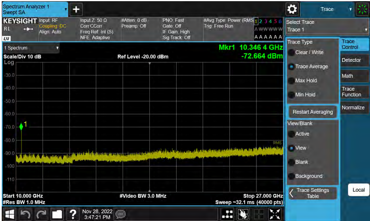
Sub6 n41. Conducted Spurious Plot 2 (15 MHz Ch. 518598 BPSK RB 1)
