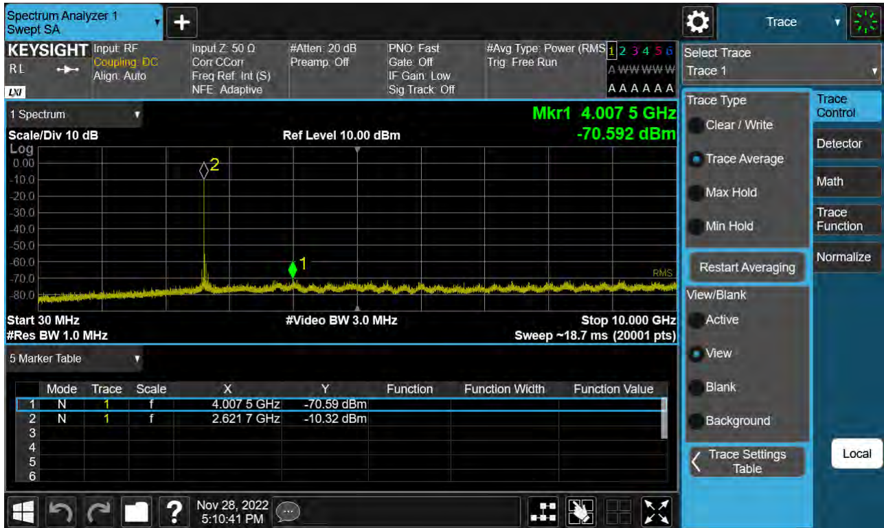
Sub6 n41. Conducted Spurious Plot 1 (70 MHz Ch.531000 BPSK RB 1)
