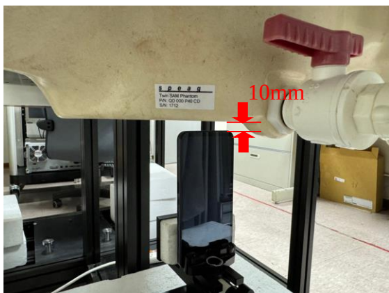
Photograph 10. Body, Bottom Edge, 10mm
