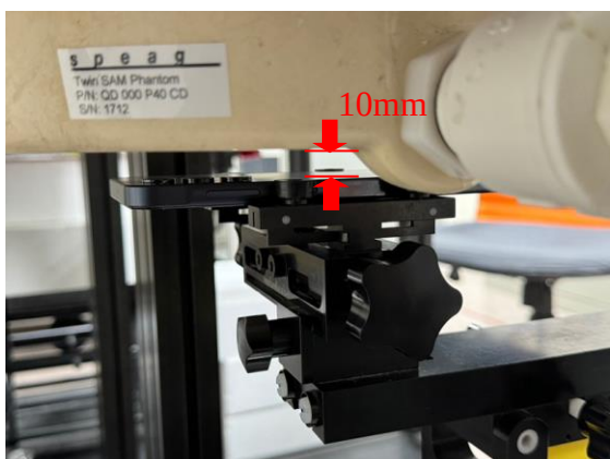
Photograph 12. Body, Rear Side, 10mm
