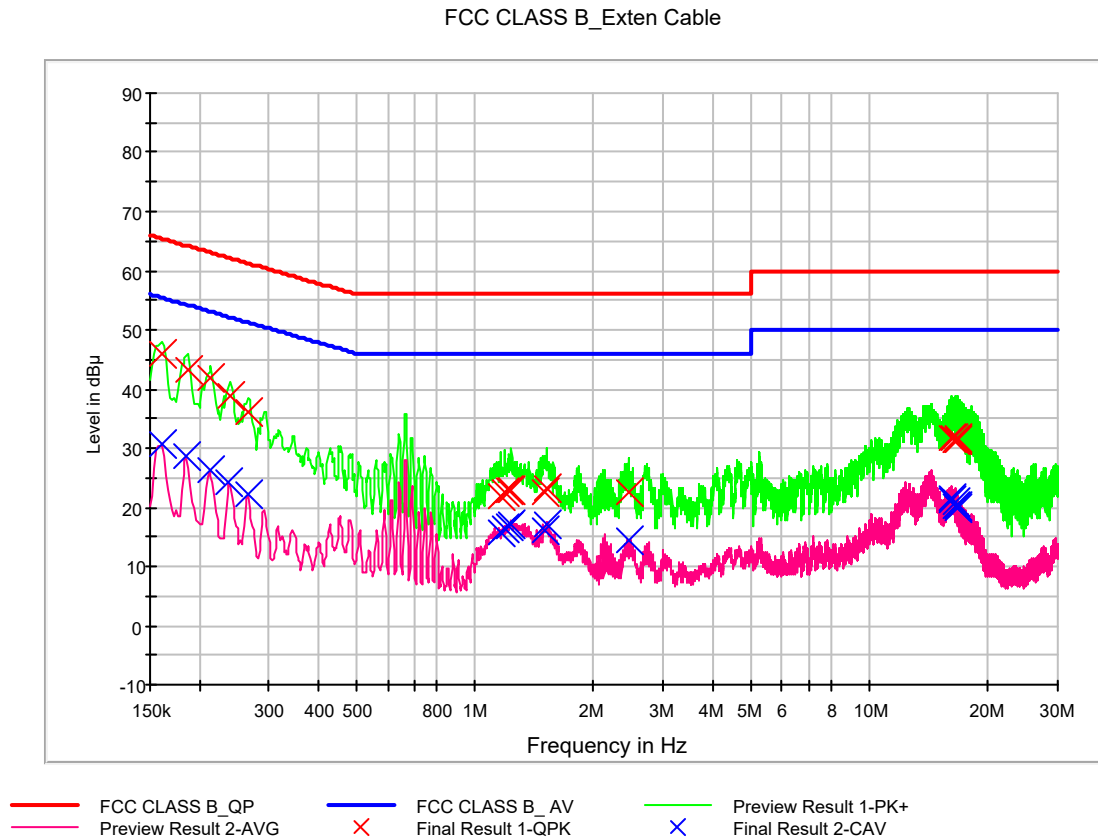
Figure 1: Conducted Emission, Line (L1)
