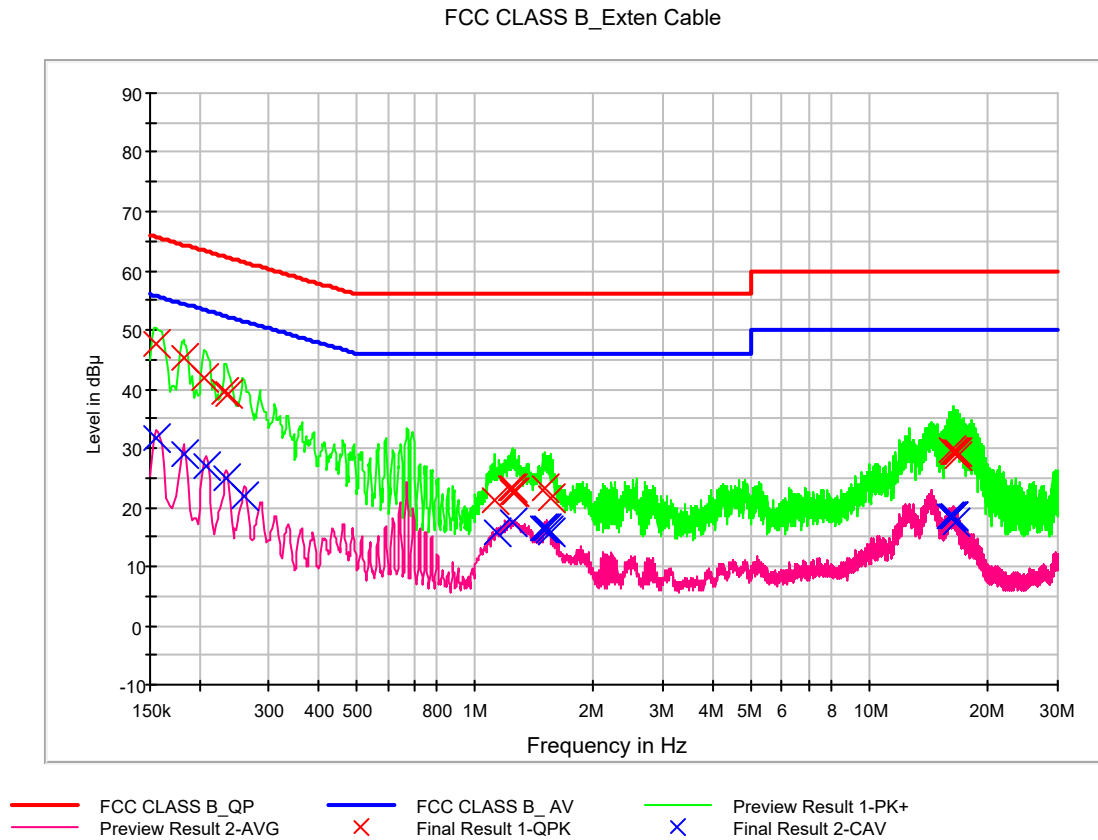
Figure 2: Conducted Emission, Line (N)
