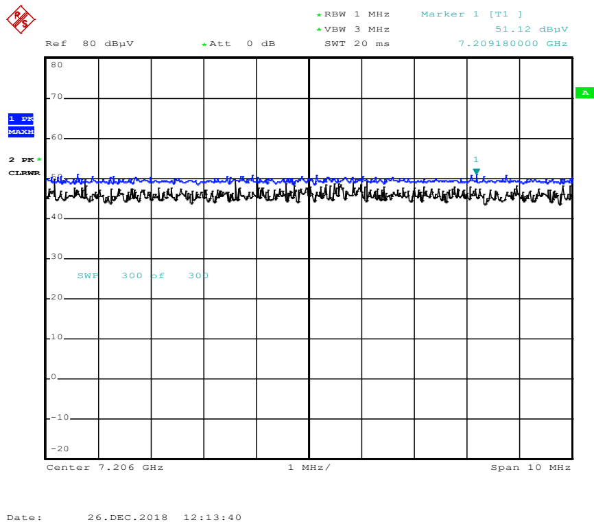
Radiated Spurious Emissions plot – Peak Reading (Ch.0 3 rd Harmonic)
