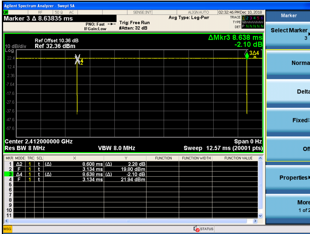
Duty cycle plot (802.11b(1Mbps))
