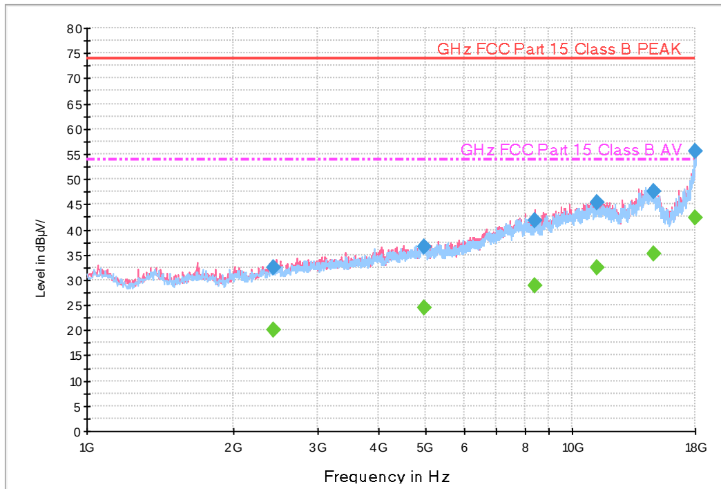
Figure 4: LTE B5 Middle ch Idle
