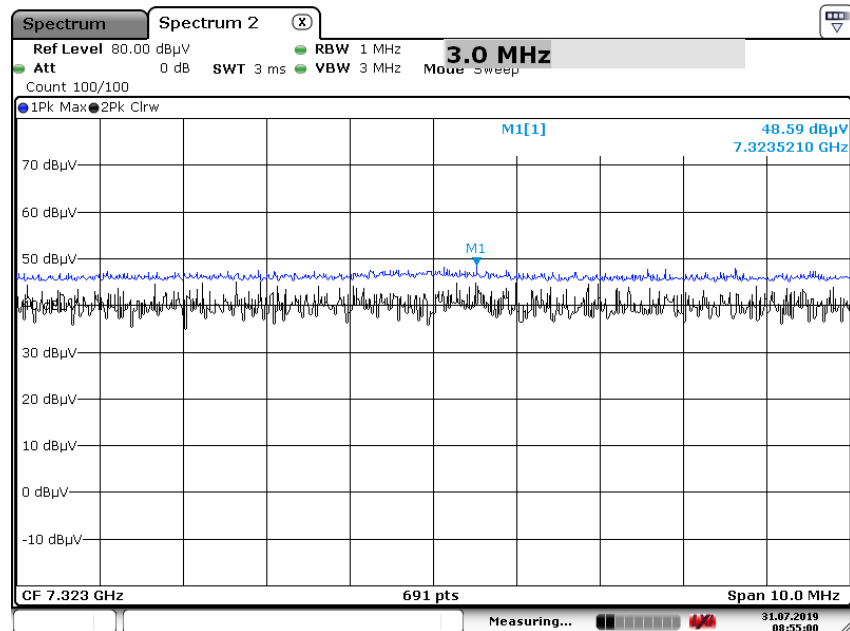
Radiated Spurious Emissions plot – Peak Reading (GFSK, Ch.39 3rd Harmonic)
