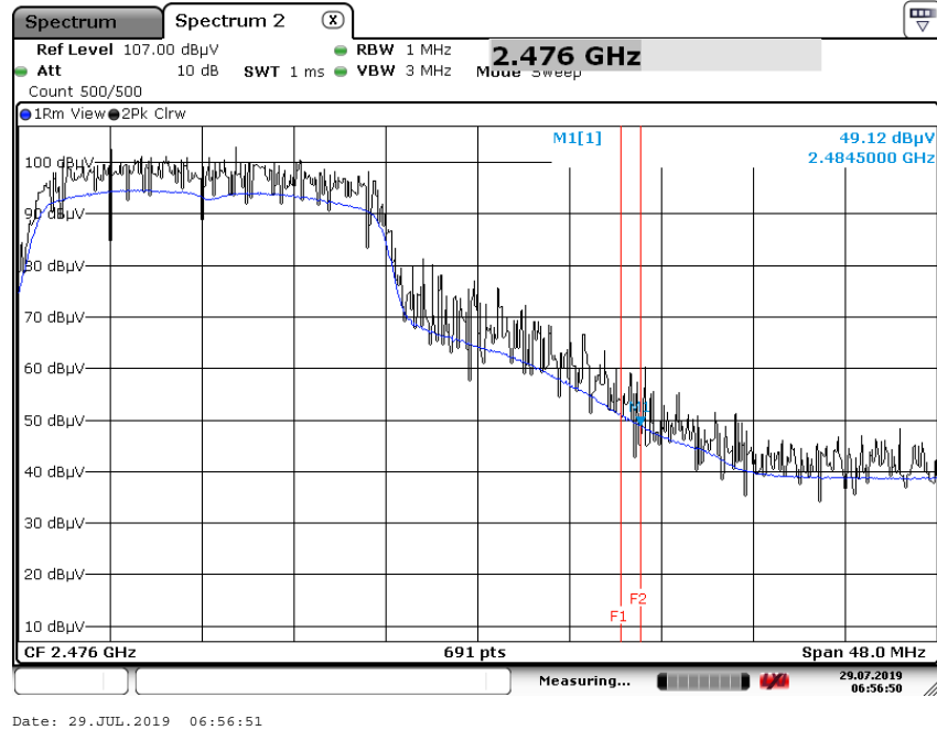
Radiated Restricted Band Edges plot – Peak Reading (802.11n(HT20) Ch.11)_ 2 484.5 MHz ~ 2.5 GHz
