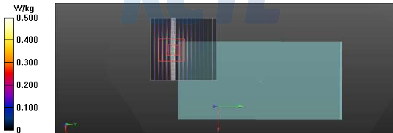
<Plot. Combine Average SAR 1g Result>
