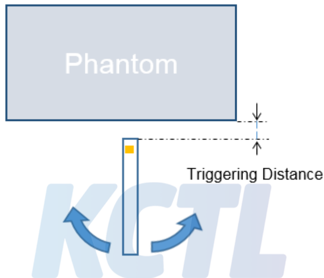
Proximity sensor tilt angle assessment (Bottom) KDB 616217 §6.4
