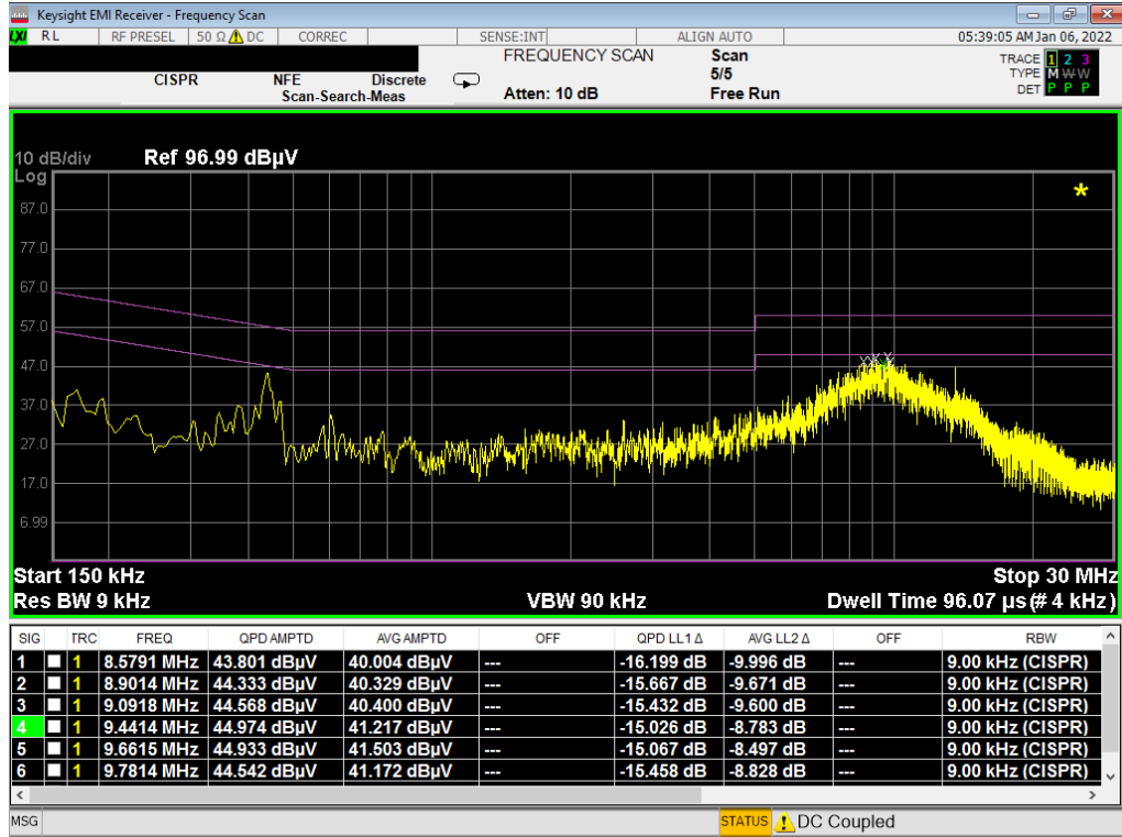
Plot 7-5. Line-Conducted Test Plot (L1)
