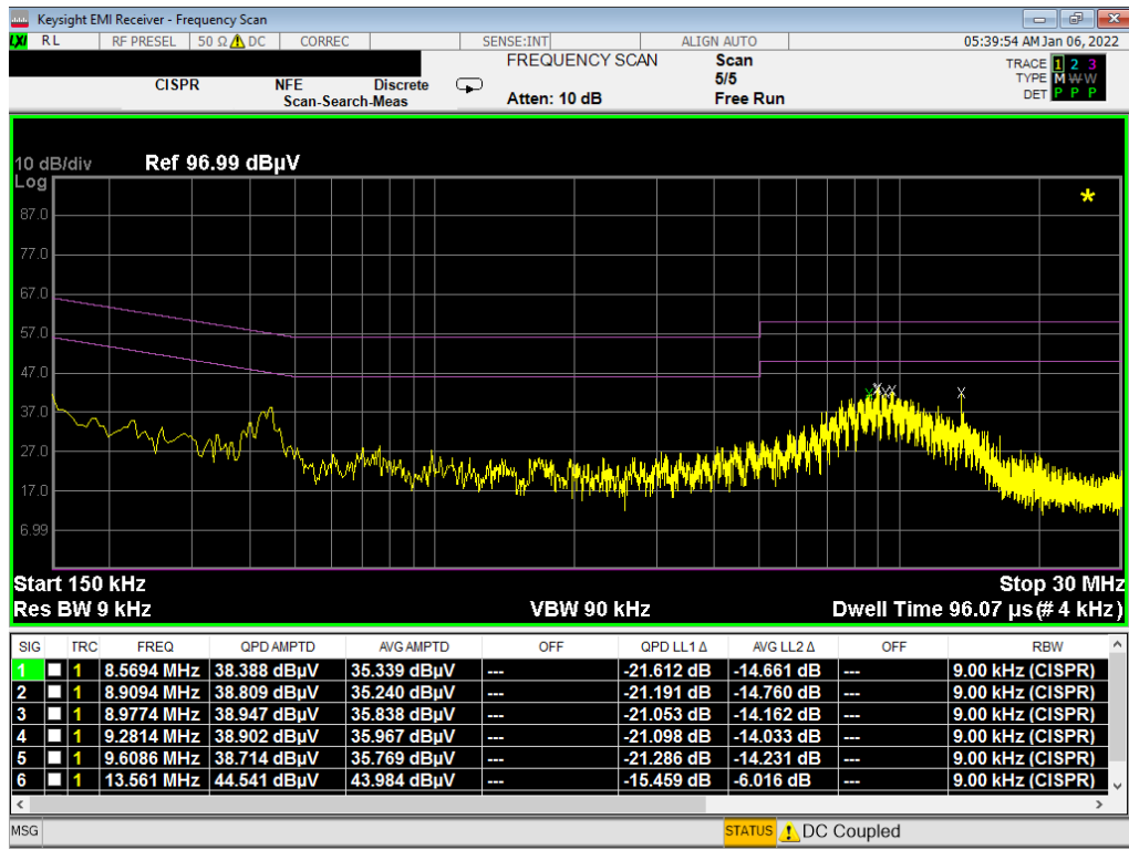
Plot 7-6. Line-Conducted Test Plot (N)
