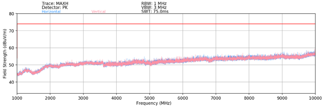
Plot 7-2. Radiated Spurious Plot above 1GHz
