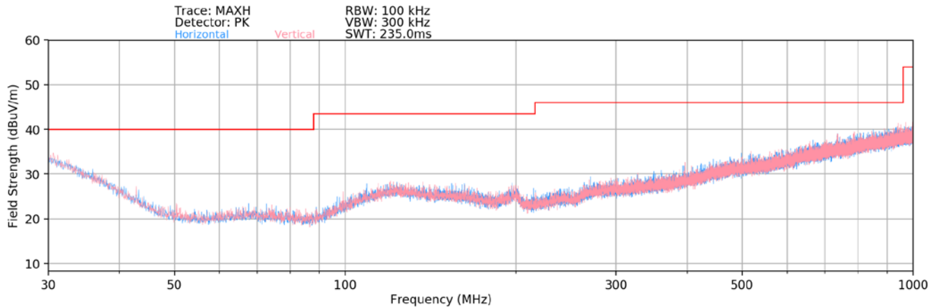
Plot 7-1. Radiated Spurious Plot below 1GHz
