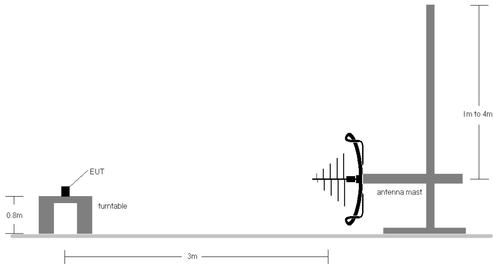
Figure 7-1. Radiated Test Setup <1GHz
