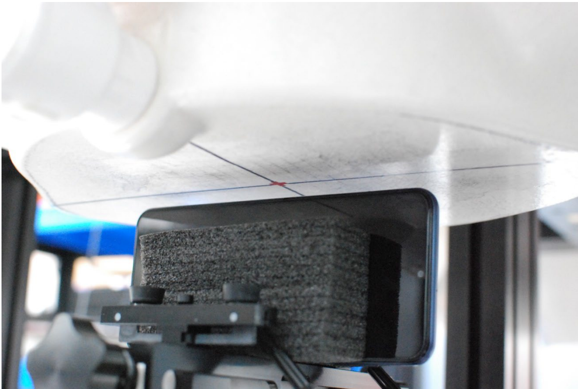
SAR Test Setup Photo 18 – Phablet, Left Edge at 6 mm
