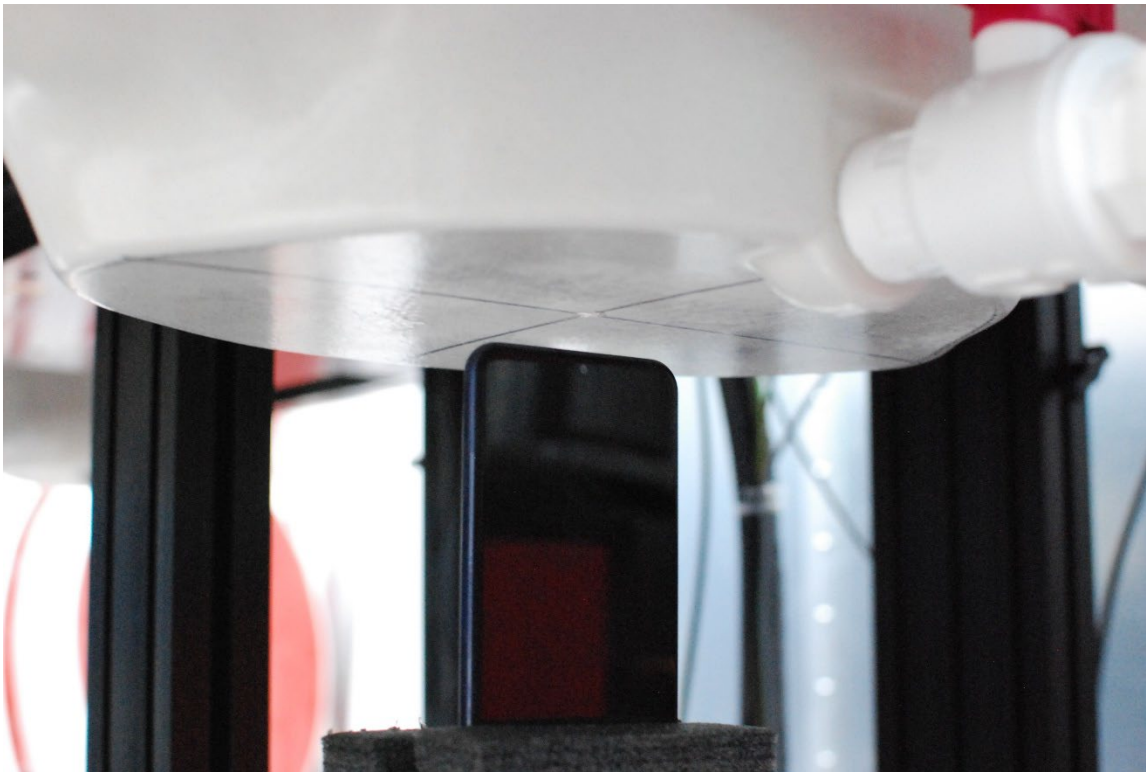
SAR Test Setup Photo 14 – Hotspot, Top Edge at 10 mm
