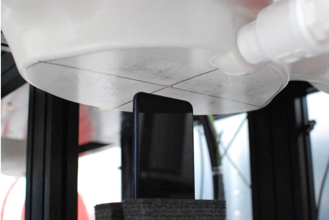
SAR Test Setup Photo 11 – Hotspot, Bottom Edge at 10 mm
