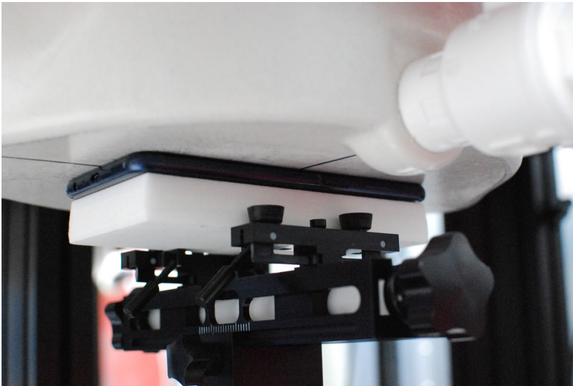
SAR Test Setup Photo 10 – Phablet, Front Side at 0 mm
