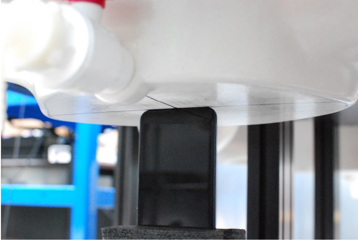
SAR Test Setup Photo 13 – Phablet, Bottom Edge at 0 mm
