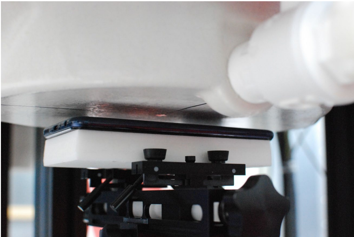
SAR Test Setup Photo 6 – Phablet, Back Side at 11 mm
