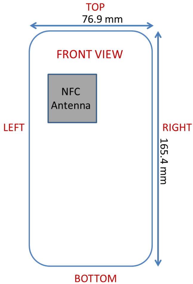
Figure E-2 NFC Antenna Locations
