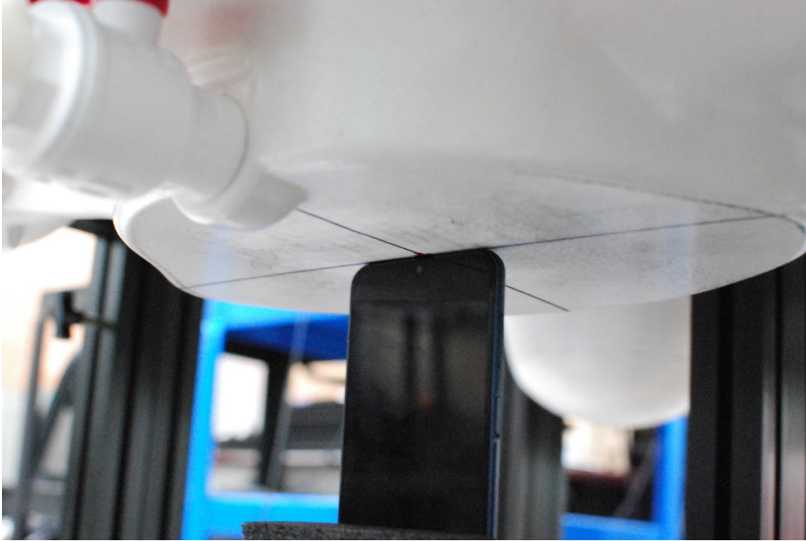
SAR Test Setup Photo 15 – Phablet, Top Edge at 0 mm
