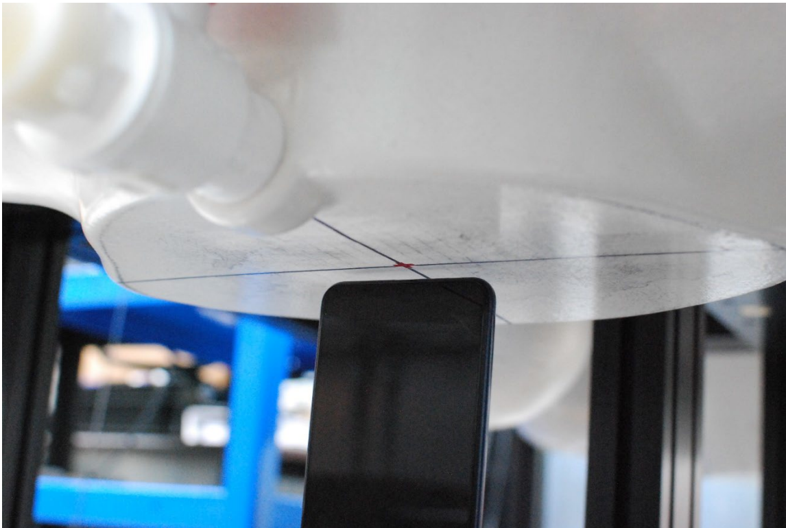
SAR Test Setup Photo 12 – Phablet, Bottom Edge at 5 mm
