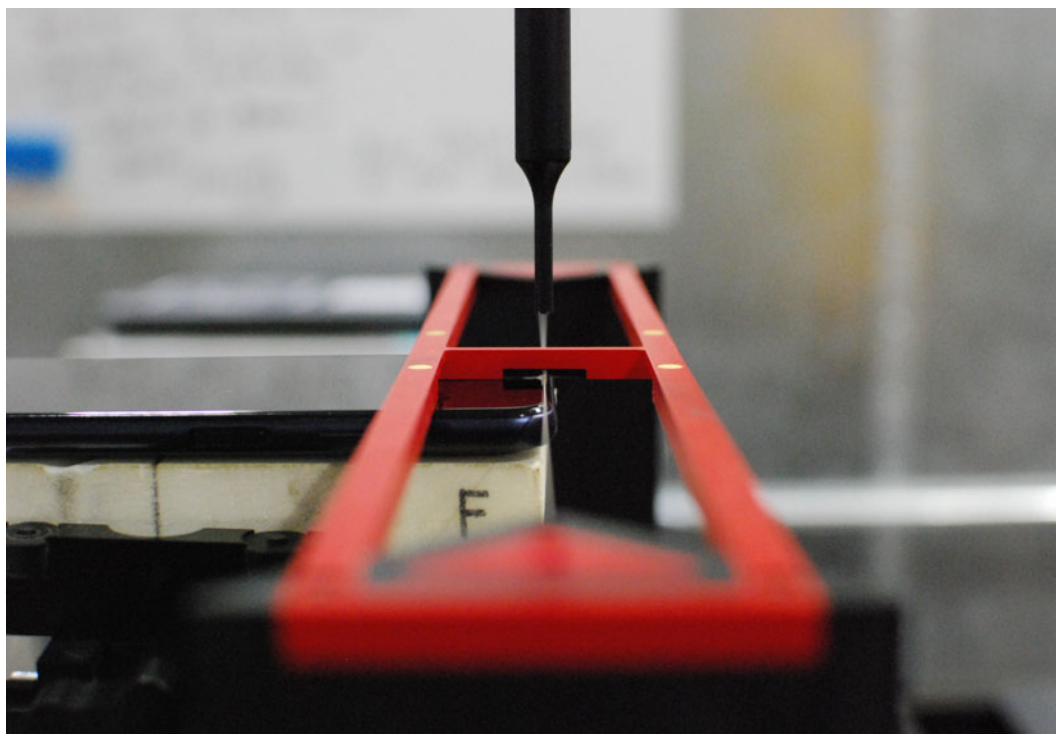
Figure 18-2 HAC Phantom Plane Alignment
