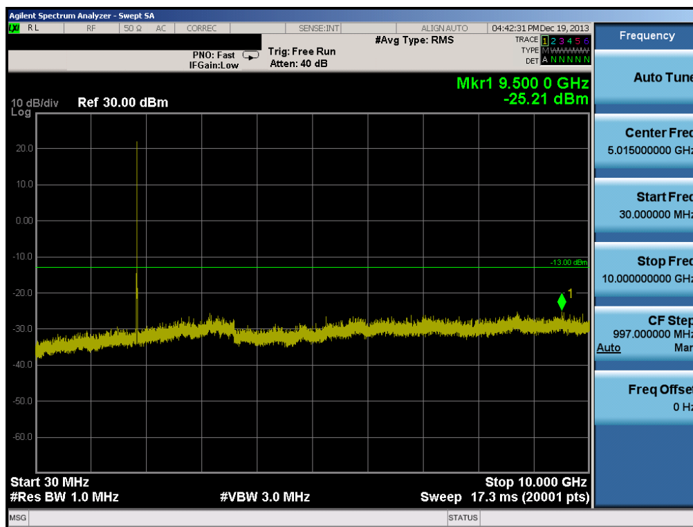
Plot 6-28. Conducted Spurious Plot (PCS WCDMA Mode – Ch. 9262)
