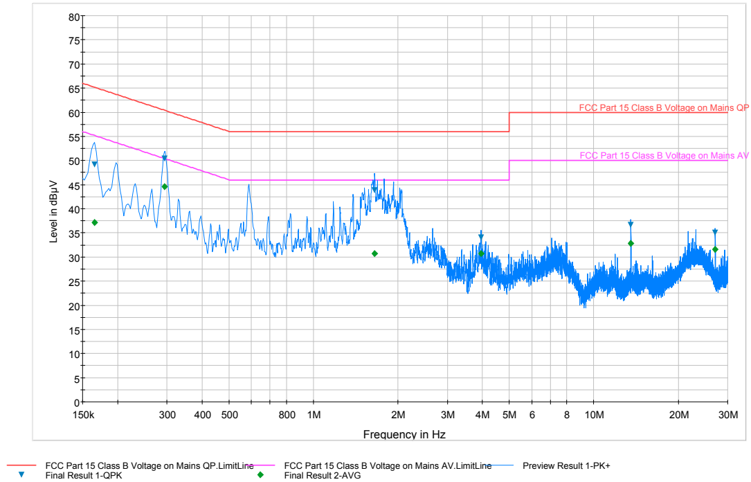
Plot 8-1. Line-Conducted Test Plot (L1)
