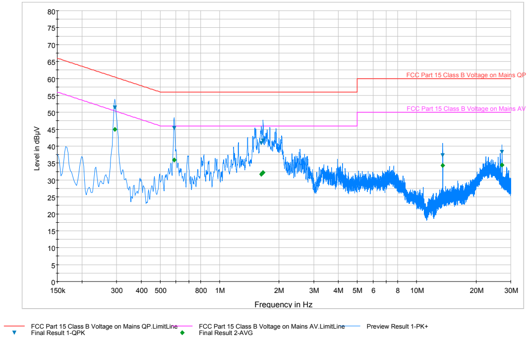
Plot 8-2. Line-Conducted Test Plot (N)
