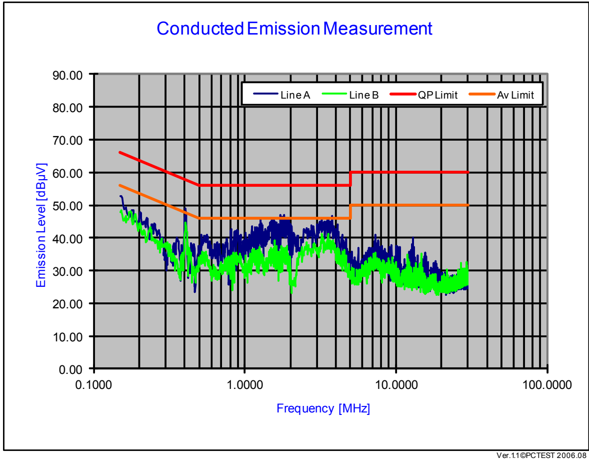
Plot 6-6. Line Conducted Plot with Bluetooth (LE)
