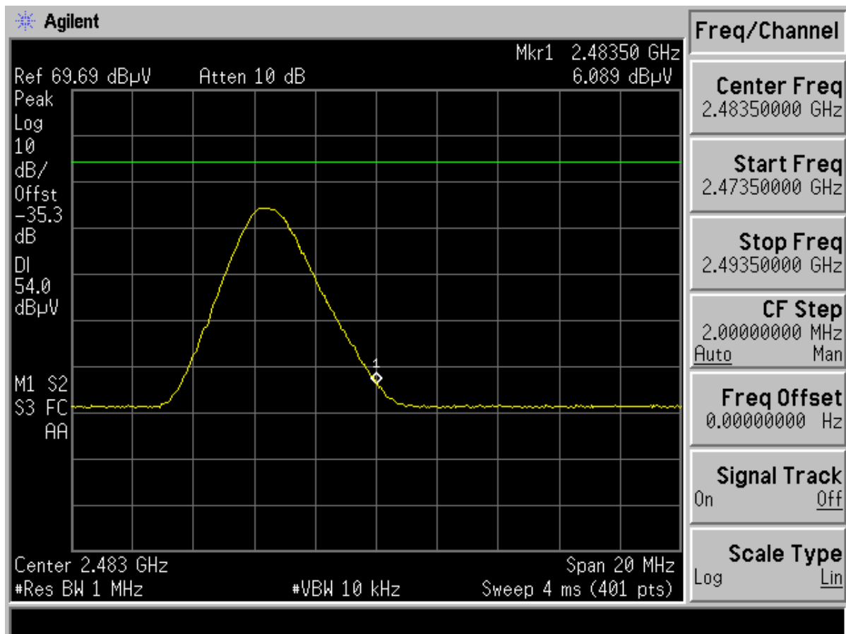
Plot 6-4. Radiated Restricted Upper Band Edge Measurement (Average)
