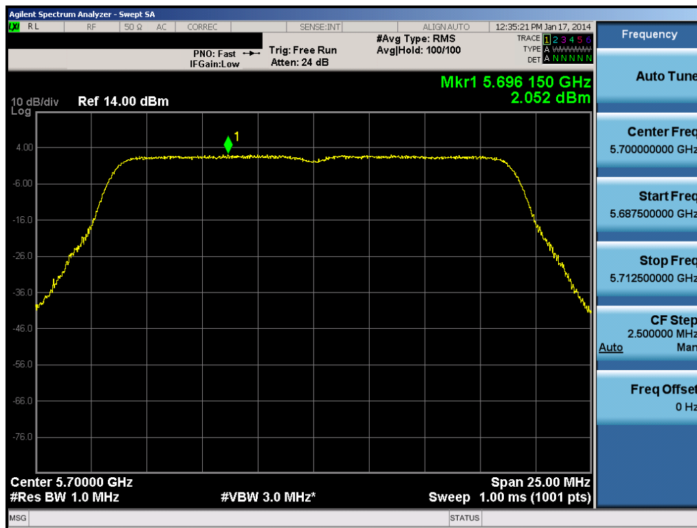
Plot 6-54. Peak Power Spectral Density Plot (20MHz BW 802.11n (UNII Band 2C) – Ch. 140)
