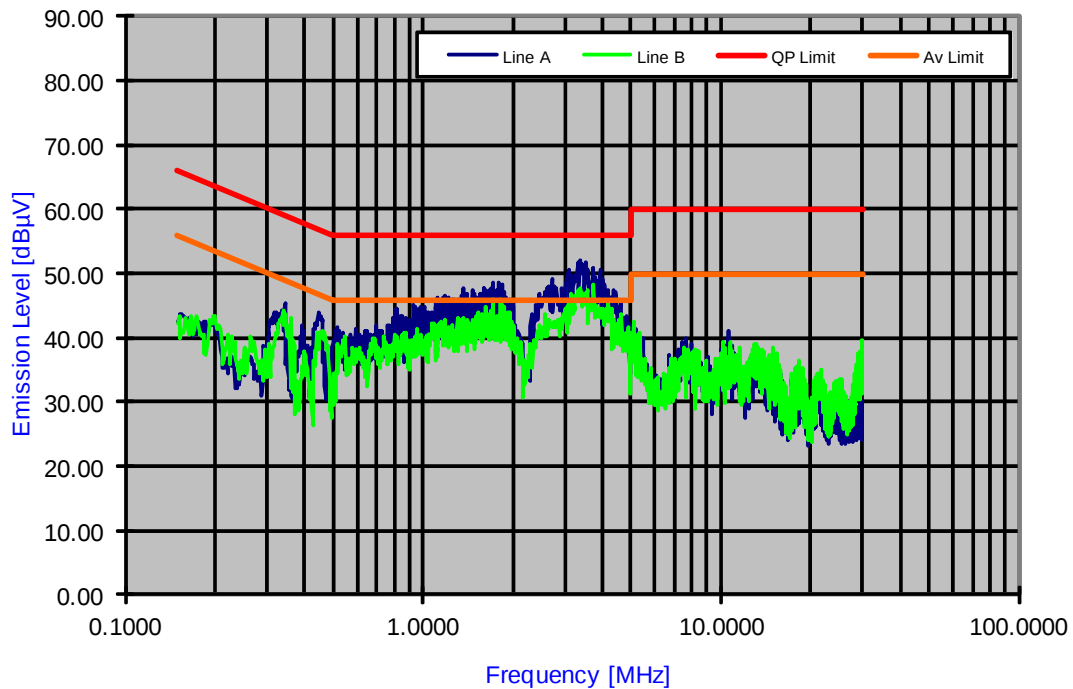
Plot 6-84. Line Conducted Plot with 802.11a (UNII Band 2A)
