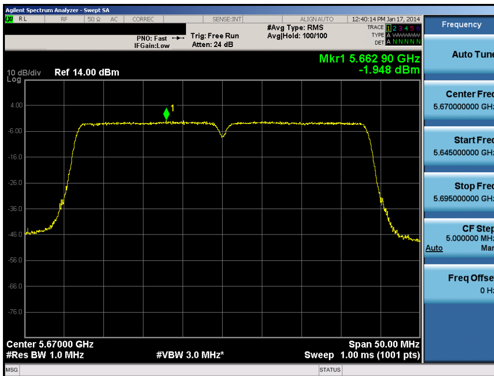
Plot 6-57. Peak Power Spectral Density Plot (40MHz BW 802.11n (UNII Band 2C) – Ch. 134)
