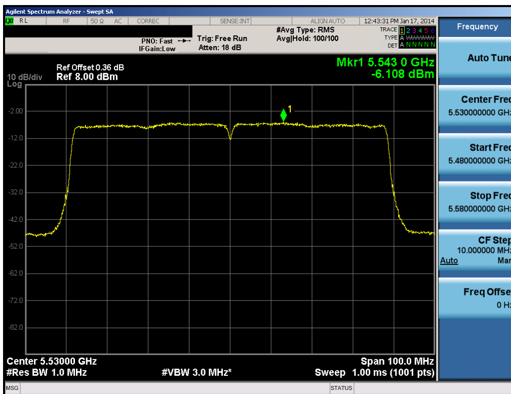
Plot 6-58. Peak Power Spectral Density Plot (80MHz BW 802.11ac (UNII Band 2C) – Ch. 106)
