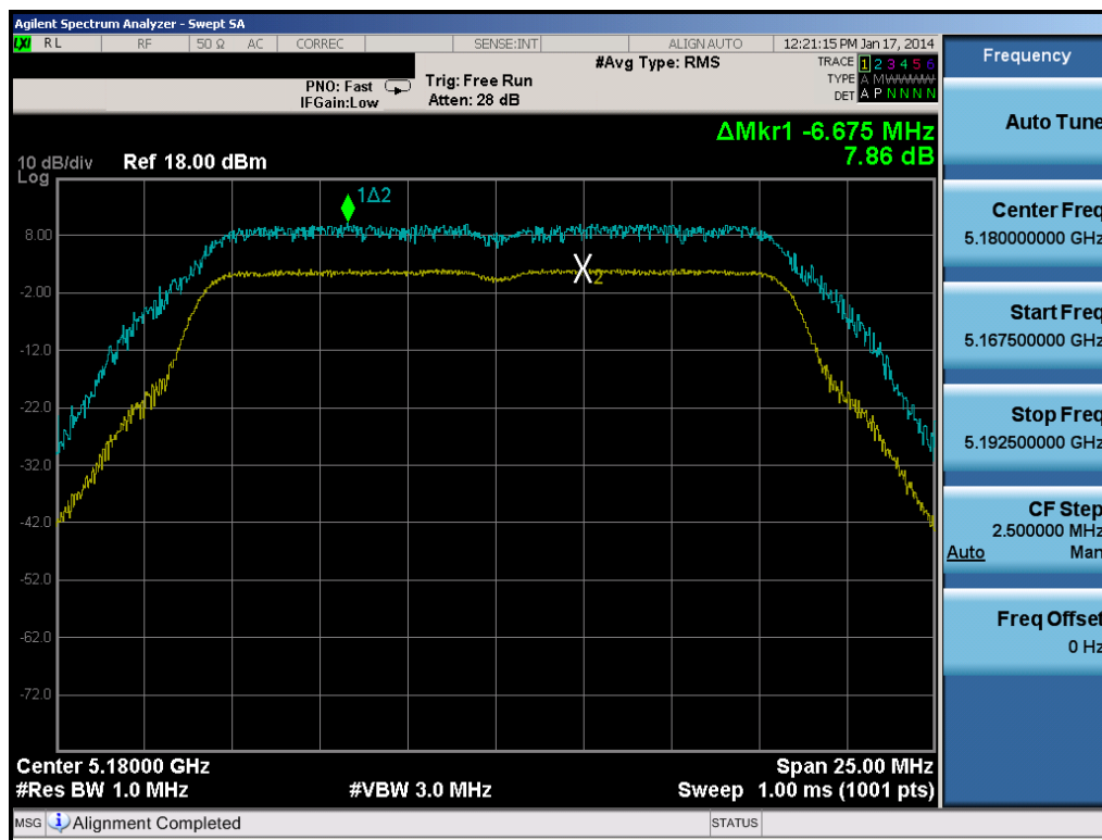
Plot 6-59. Peak Excursion Ratio Plot (802.11a)
