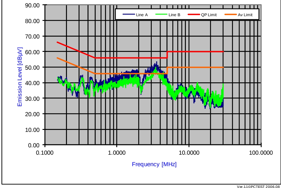
Plot 6-85. Line Conducted Plot with 802.11a (UNII Band 2C)
