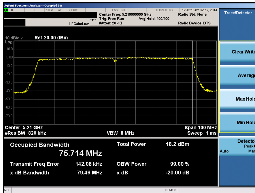
Plot 6-30. 20dB Bandwidth Plot (80MHz BW 802.11n (UNII Band 1) – Ch. 42)
